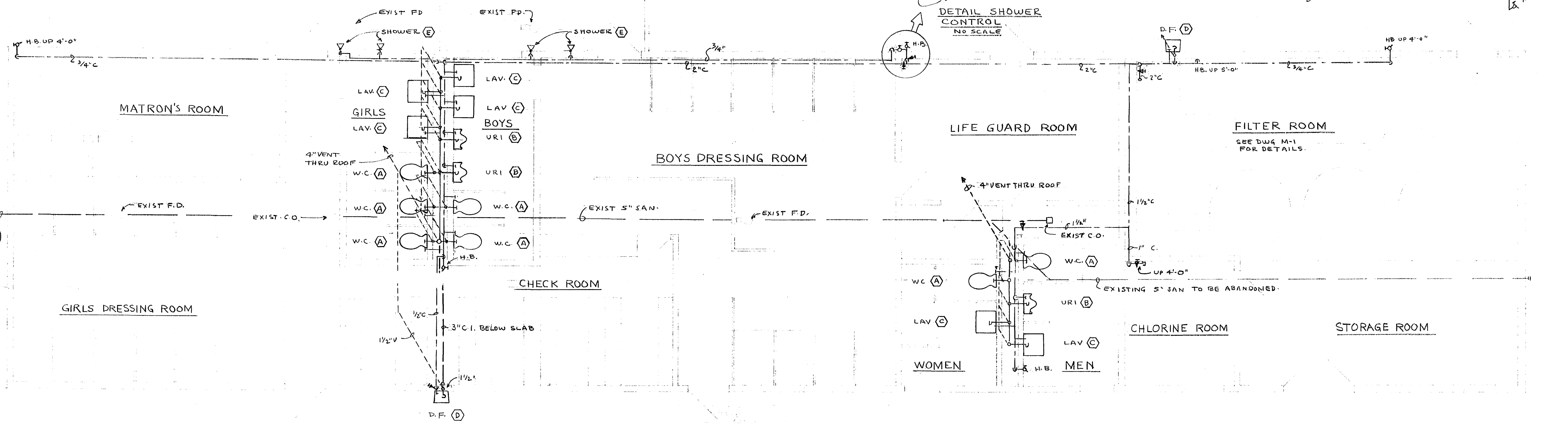
PLAN BATH HOUSE SCALE 1/4" = 1'-0"
