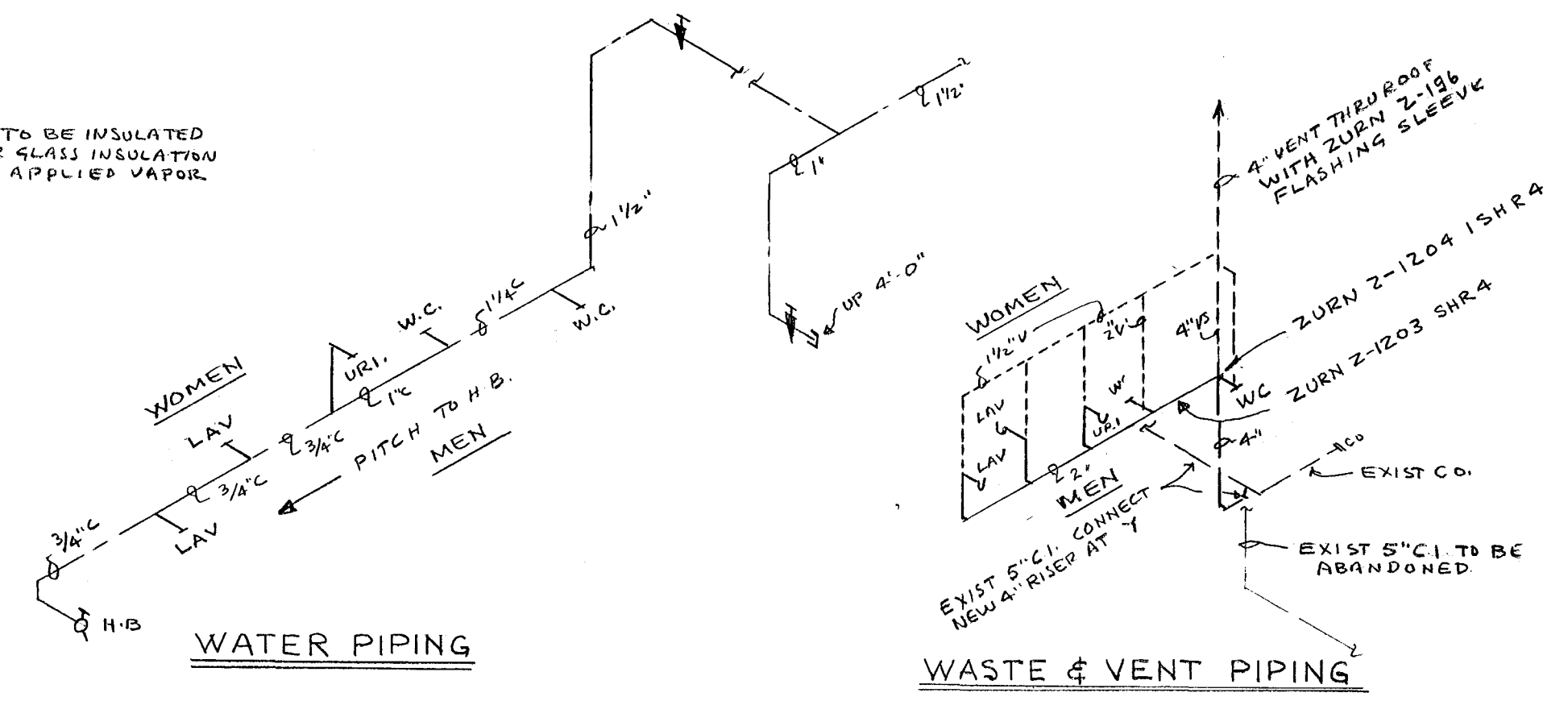
PIPING SCHEMATICS TOILETS NO SCALE
