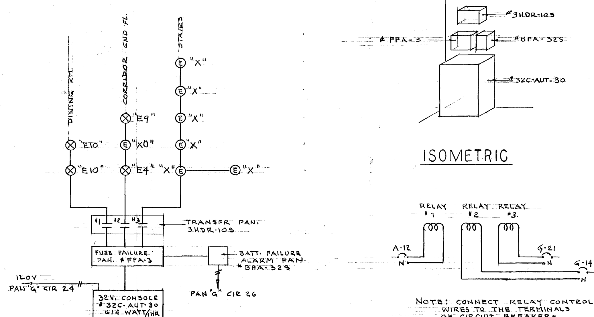
EMERG. LTG. SCHEMATIC
