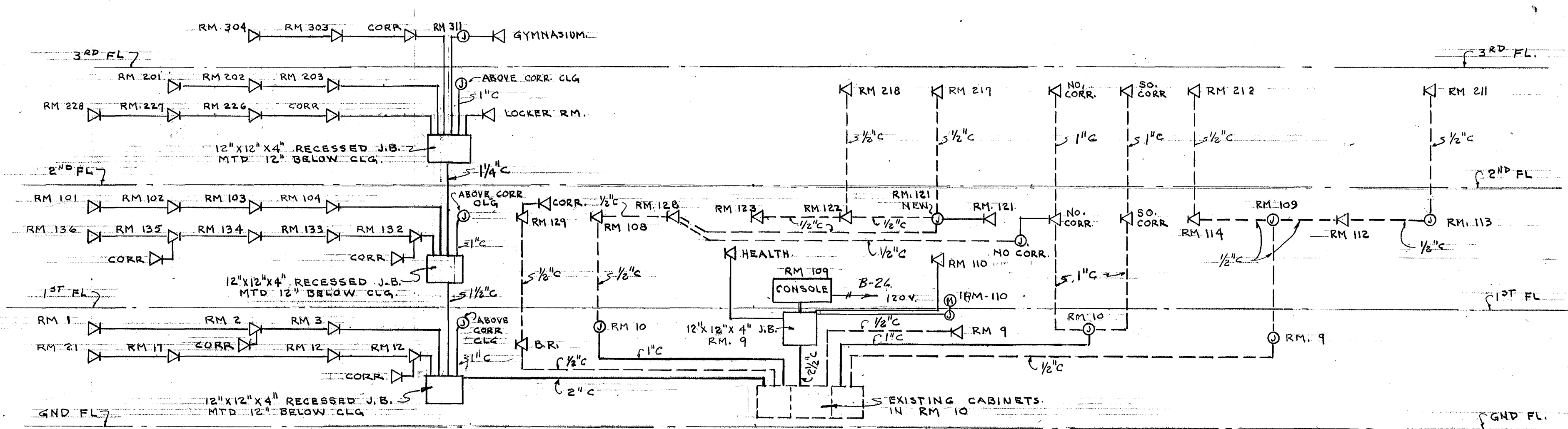
TELEPHONE RISER DIAGRAM
