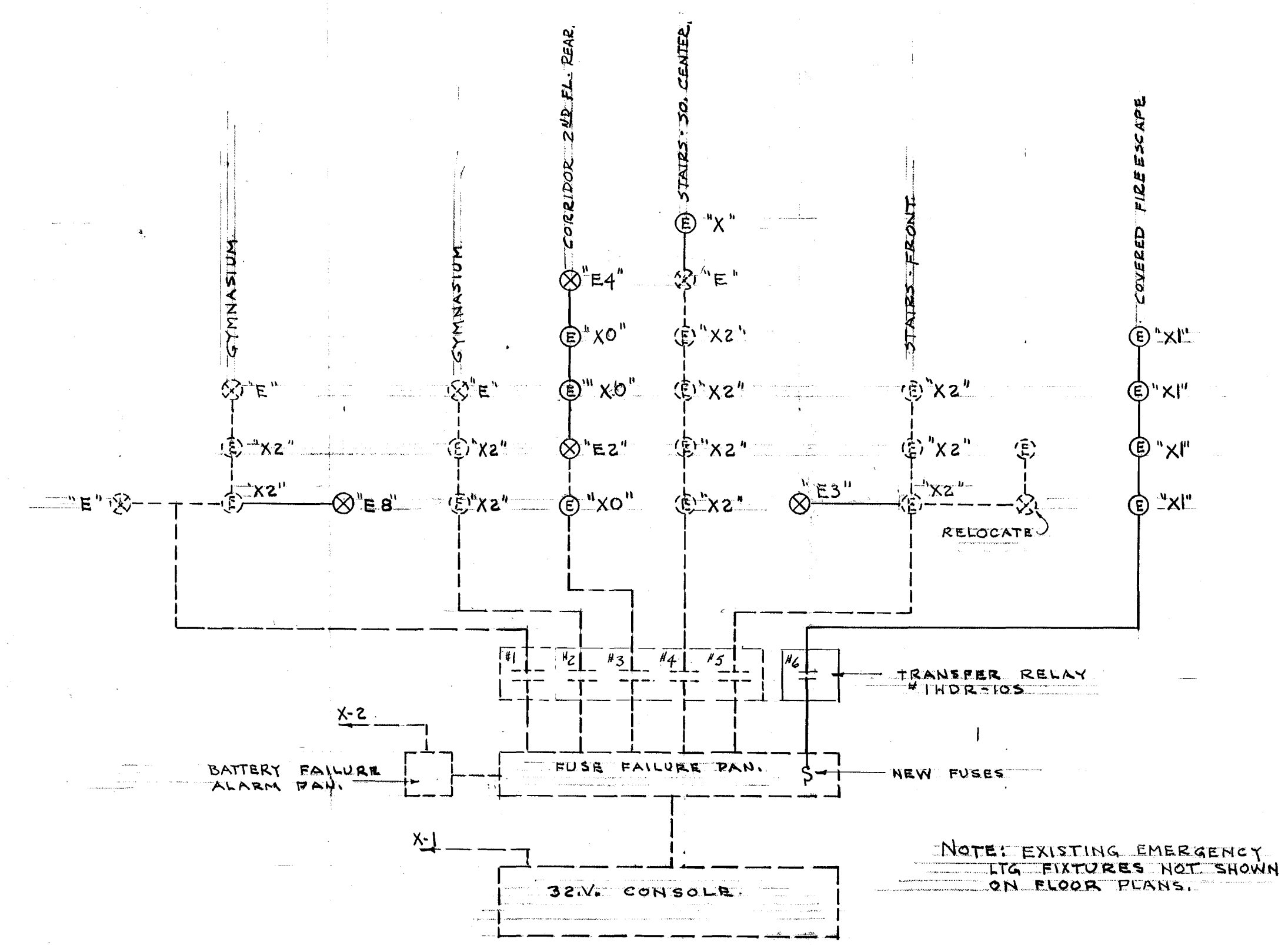
EMERGENCY LIGHTING SCHEMATIC
