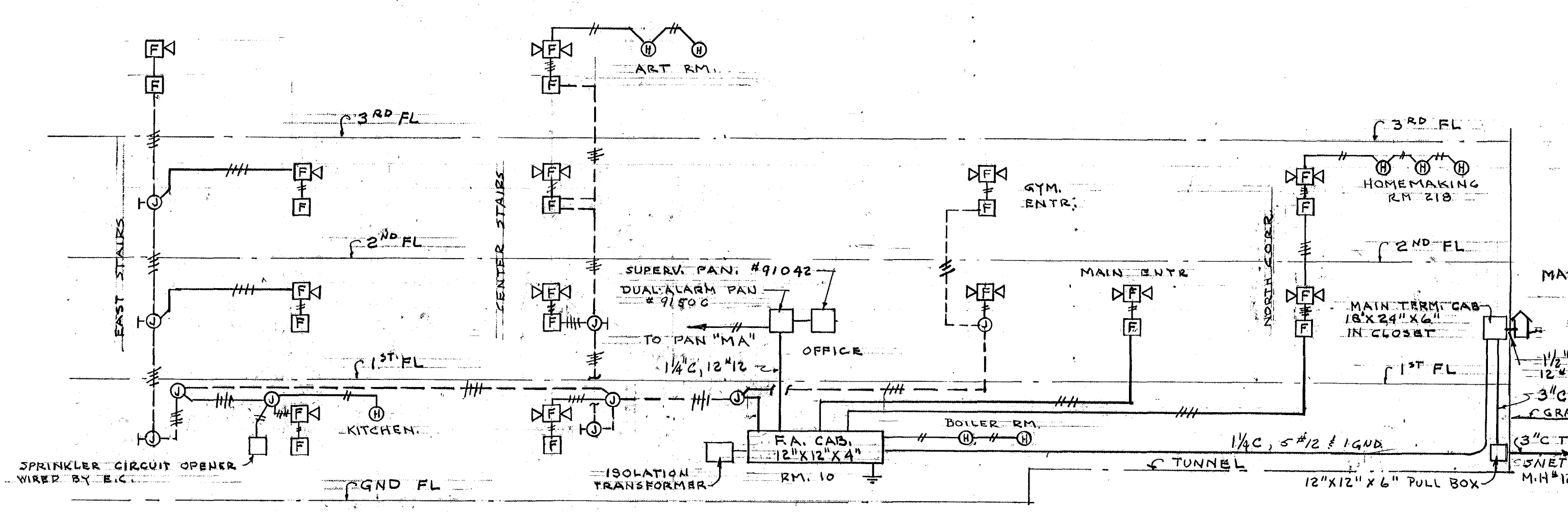
FIRE ALARM RISER DIAGRAM
