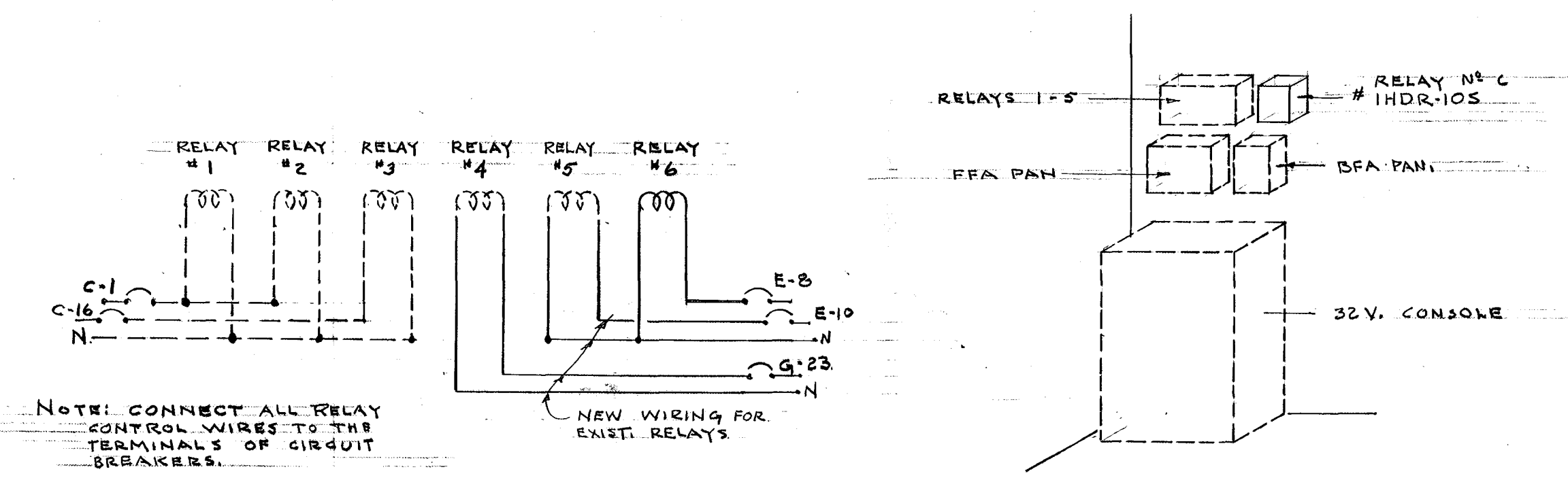
EMERGENCY LIGHTING SCHEMATIC
