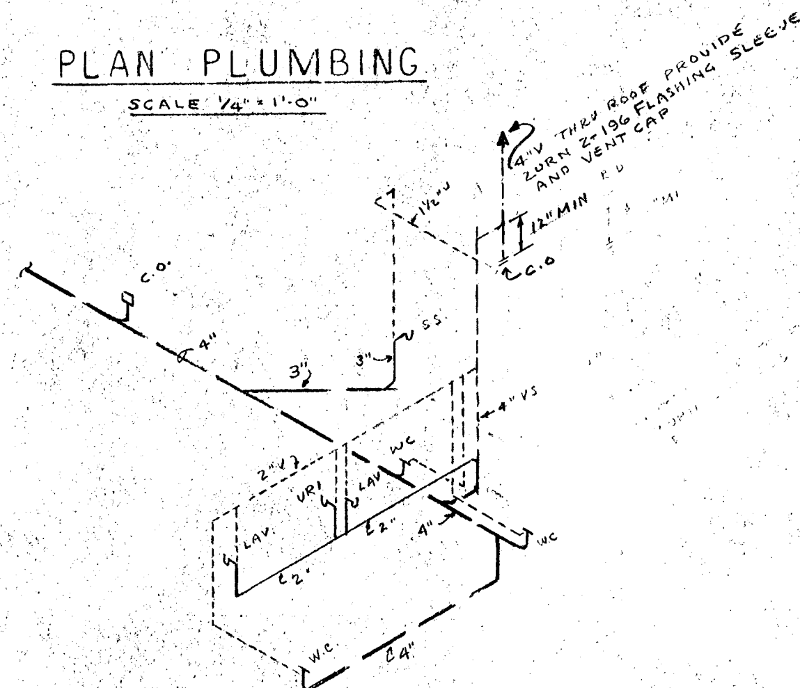
SCHEMATIC WASTE & VENT PIPING
