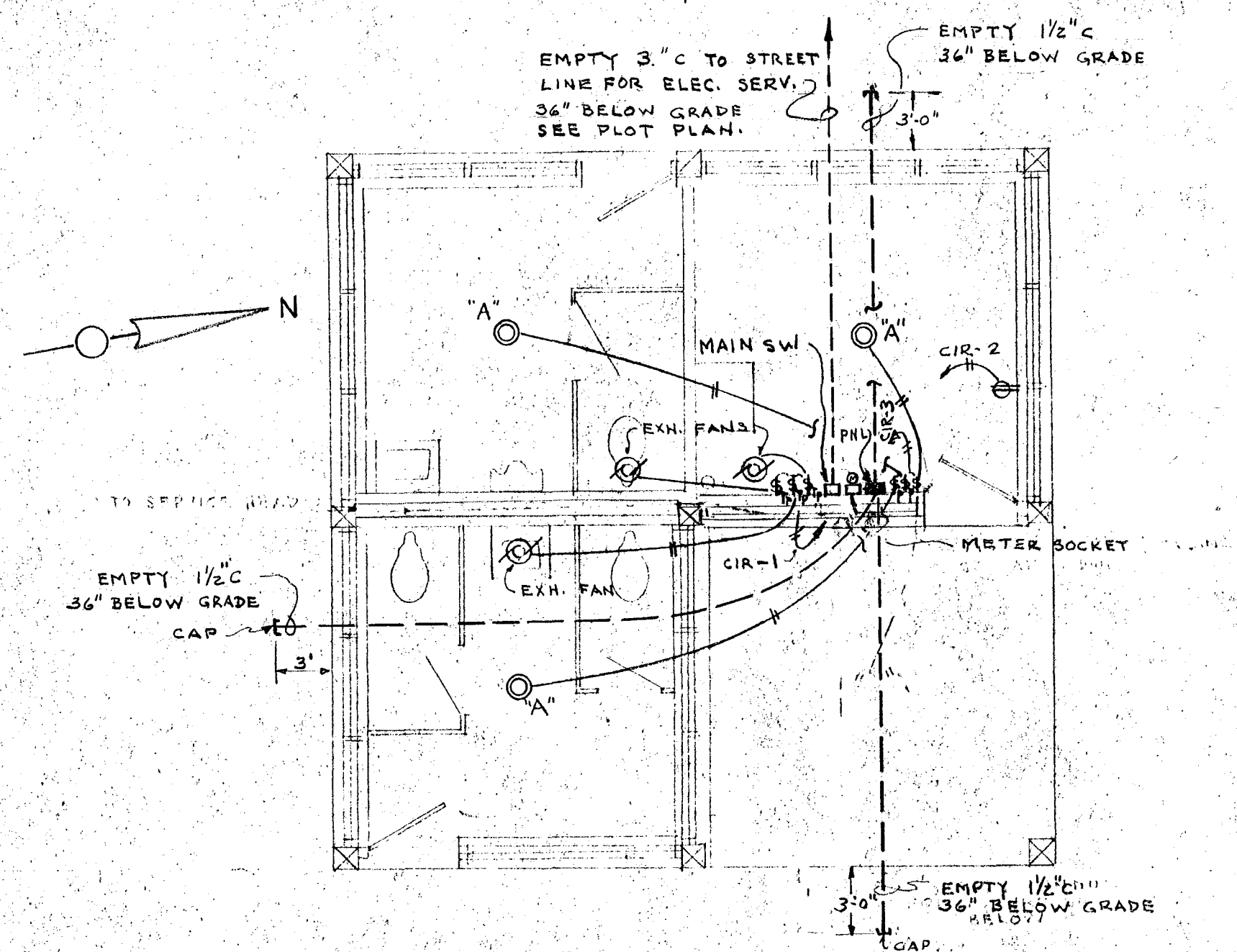
PLAN ELECTRICAL SCALE 1/4" = 1'-0"
