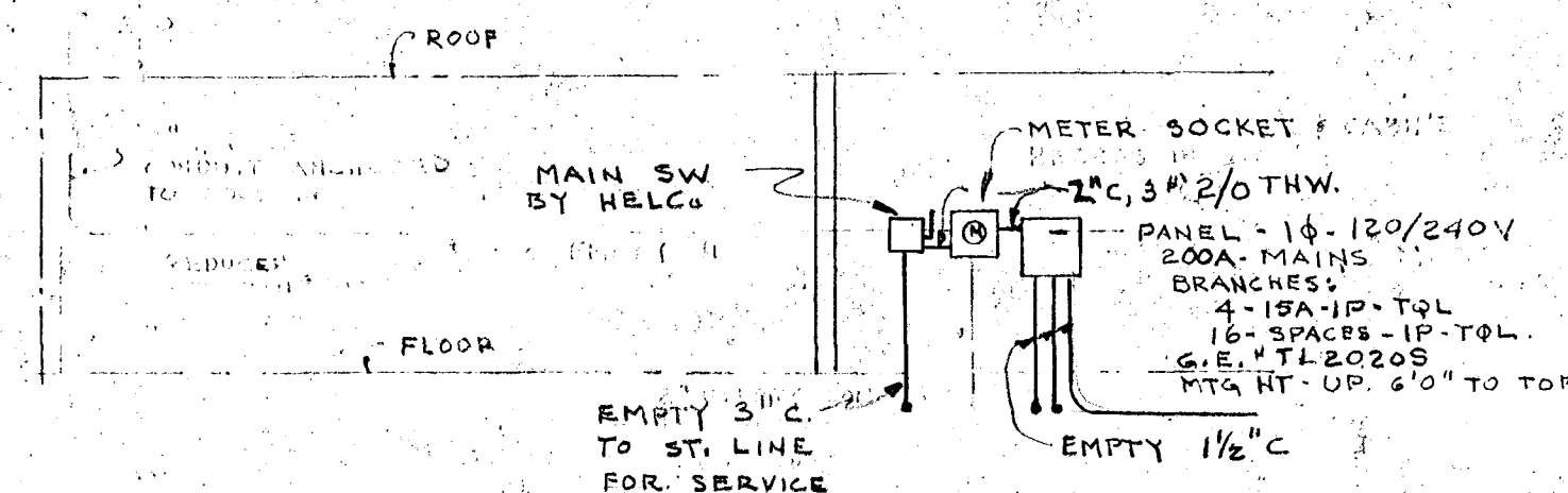
POWER RISER DIAGRAM NO SCALE
