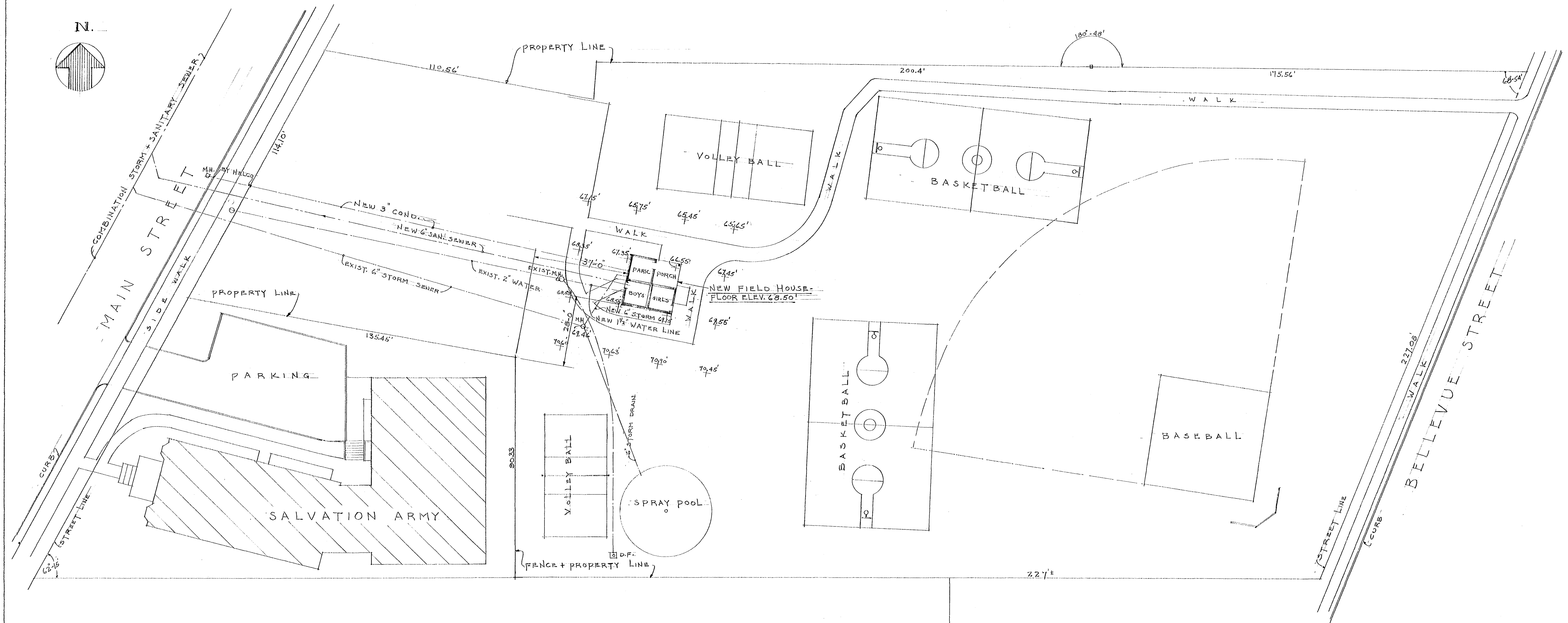
• PLOT PLAN - ST. BENEDICT'S PLAYGROUND • SCALE 1" = 20'-0"
