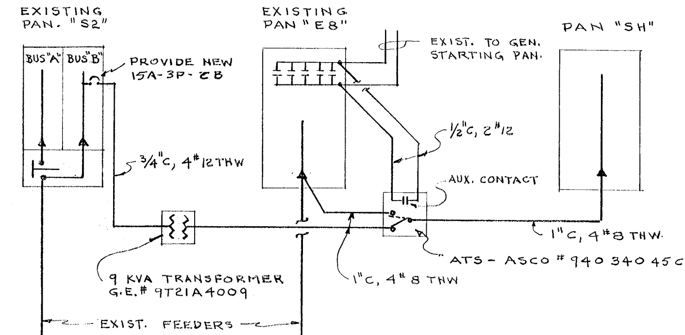
POWER RISER DIAGRAM NO SCALE
