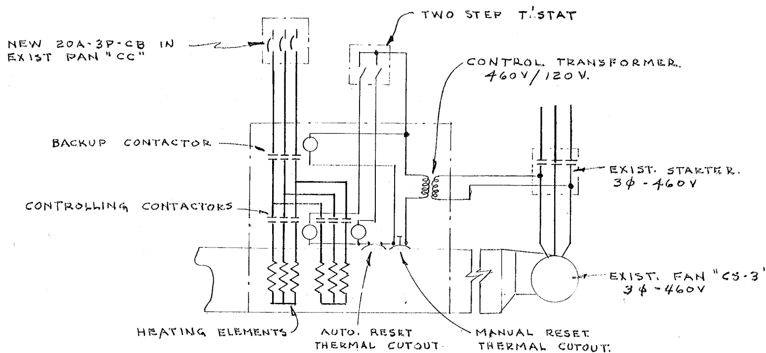
DUCT HEATER WIRING DIAGRAM NO SCALE
