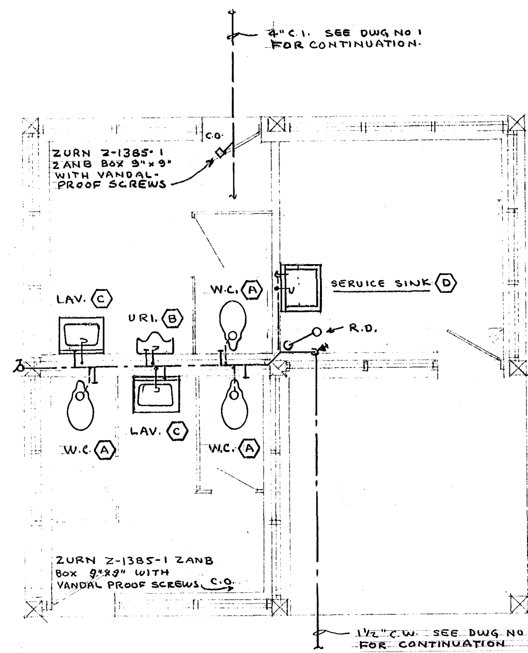
PLAN PLUMBING SCALE 1/8" = 1'-0"
