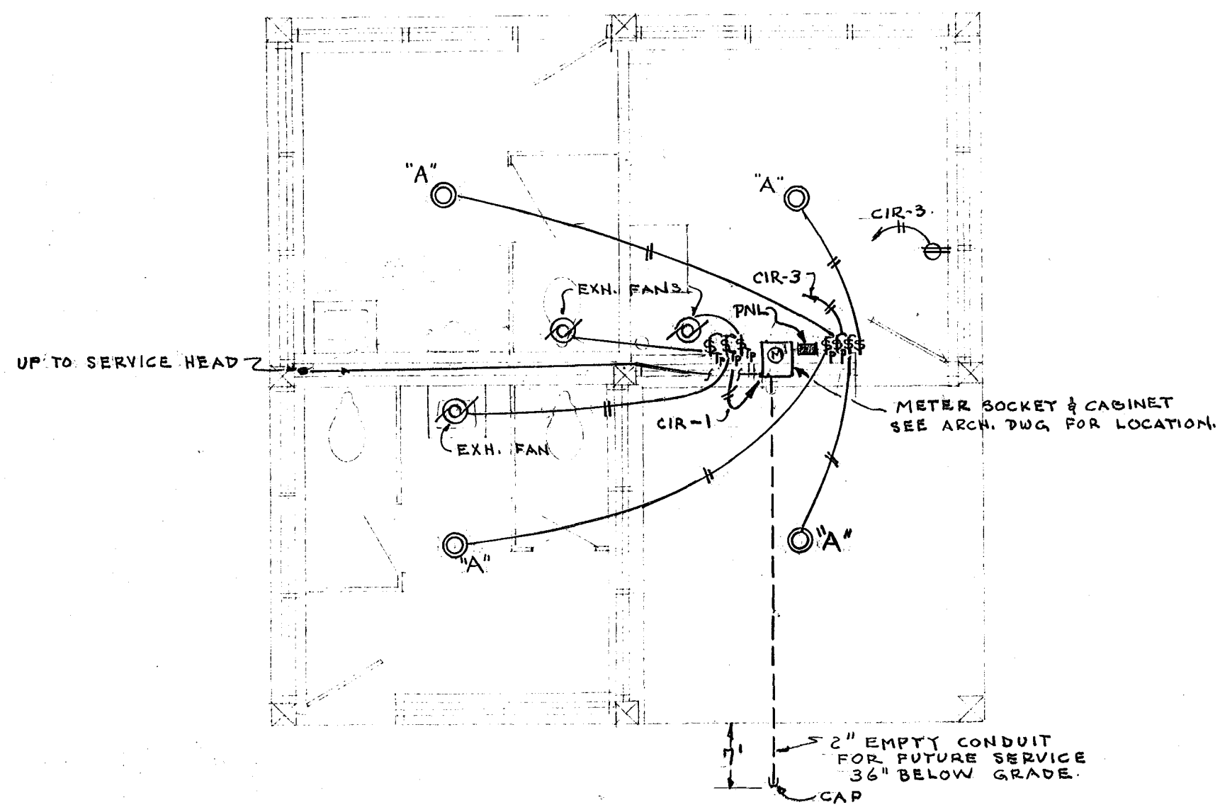
PLAN ELECTRICAL SCALE 1/8" = 1'-0"
