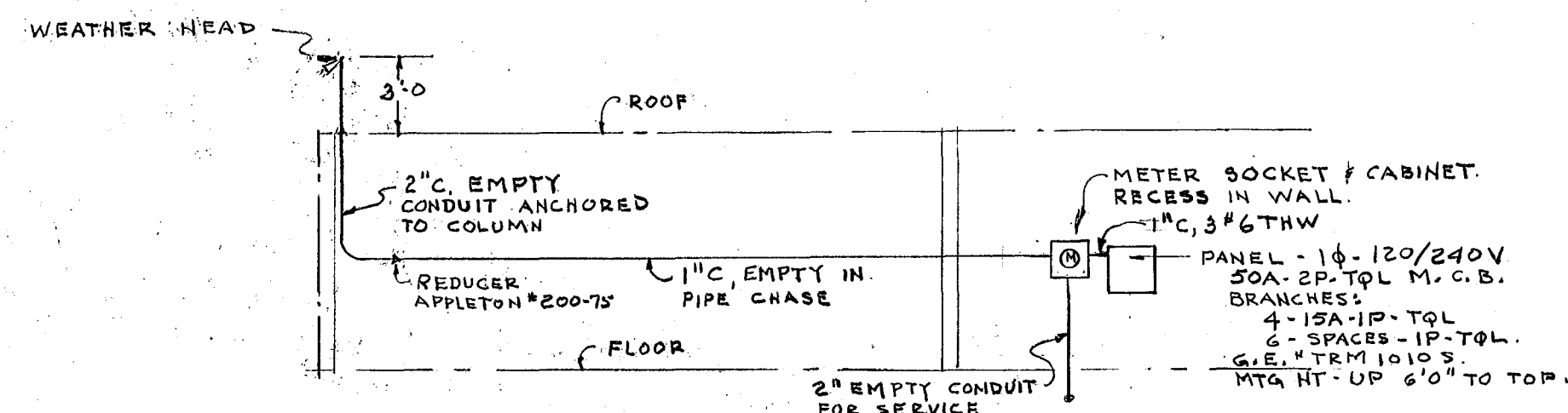
POWER RISER DIAGRAM NO SCALE
