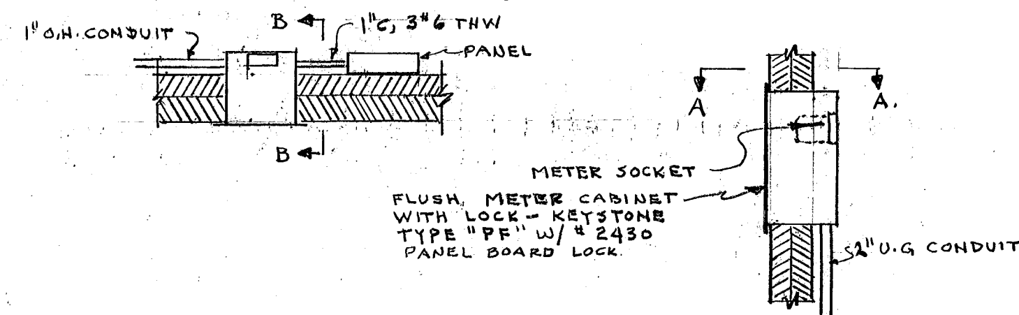
SECTION A-A DETAIL OF METER CABINET
