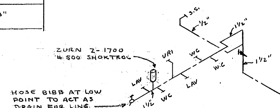
SCHEMATIC WATER PIPING NO SCALE
