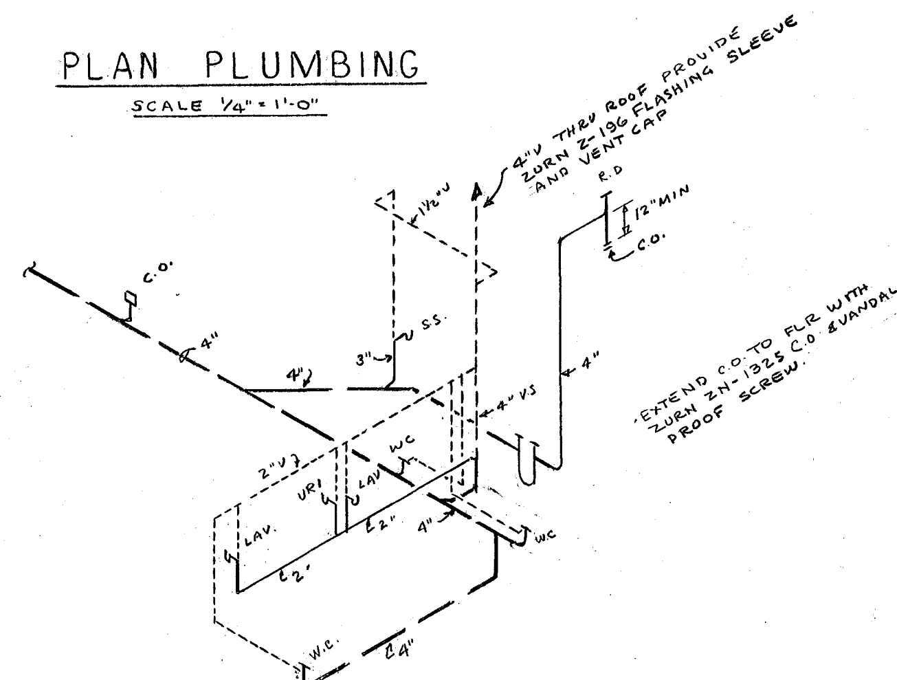
SCHEMATIC WASTE & VENT PIPING
