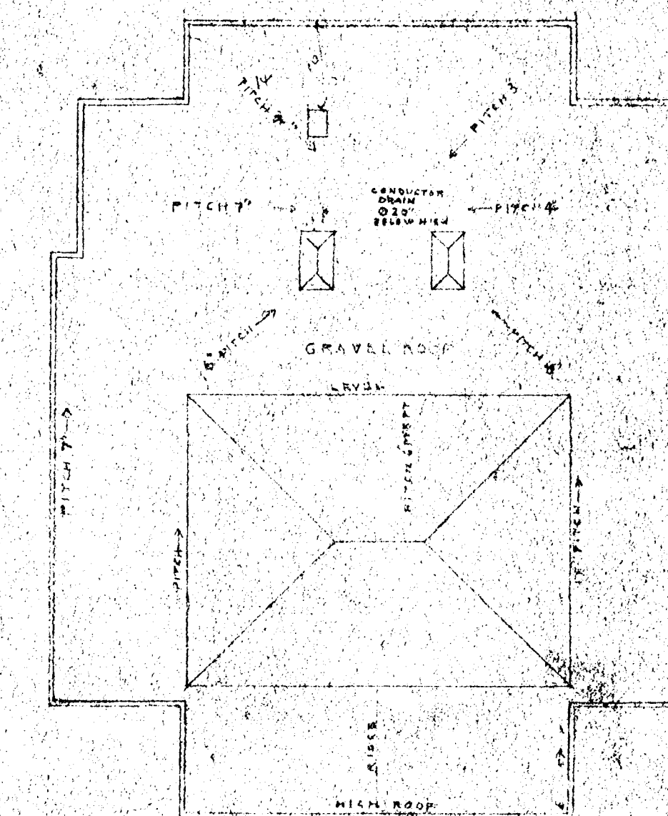
ROOF PLAN 1/4" = 1'00"
