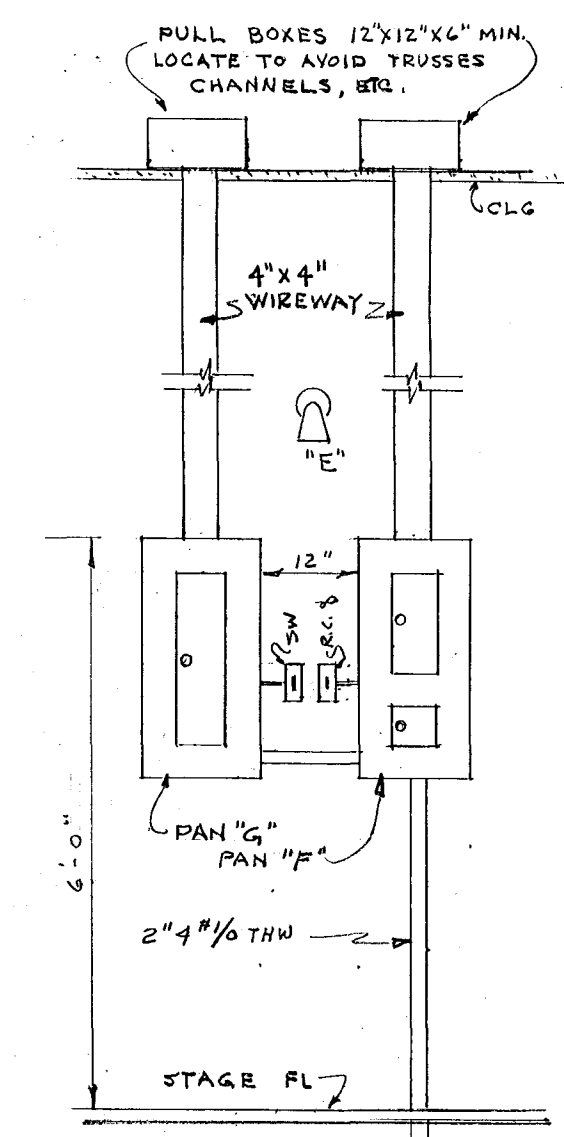
SECTION A-A NO SCALE
