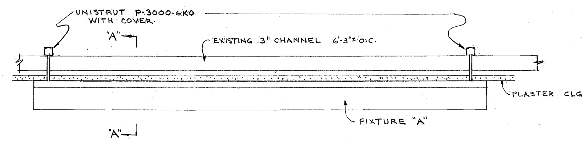
SECTION B-B
