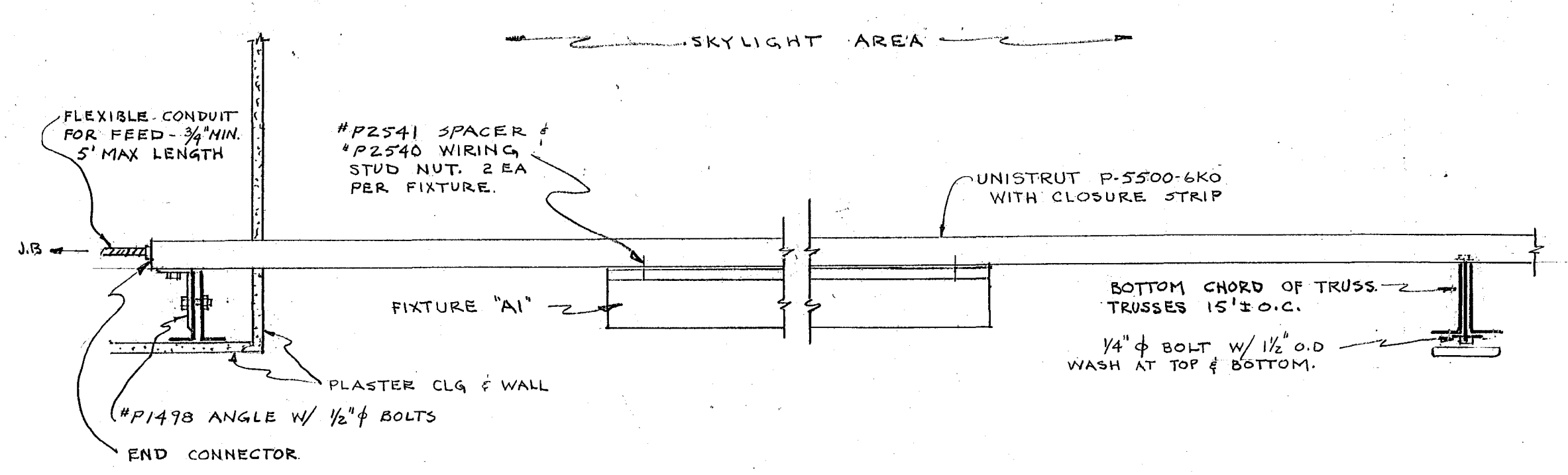
TYPICAL MOUNTING DETAIL FOR FIXTURE "A1" 1" = 1'-0" (APPROX)
