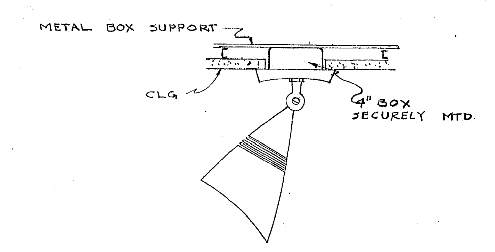
MOUNTING DETAIL FIXTURES "C" & "D" NO SCALE
