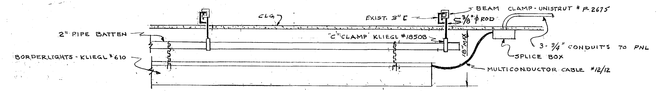
BORDERLIGHT MOUNTING DETAIL NO SCALE
