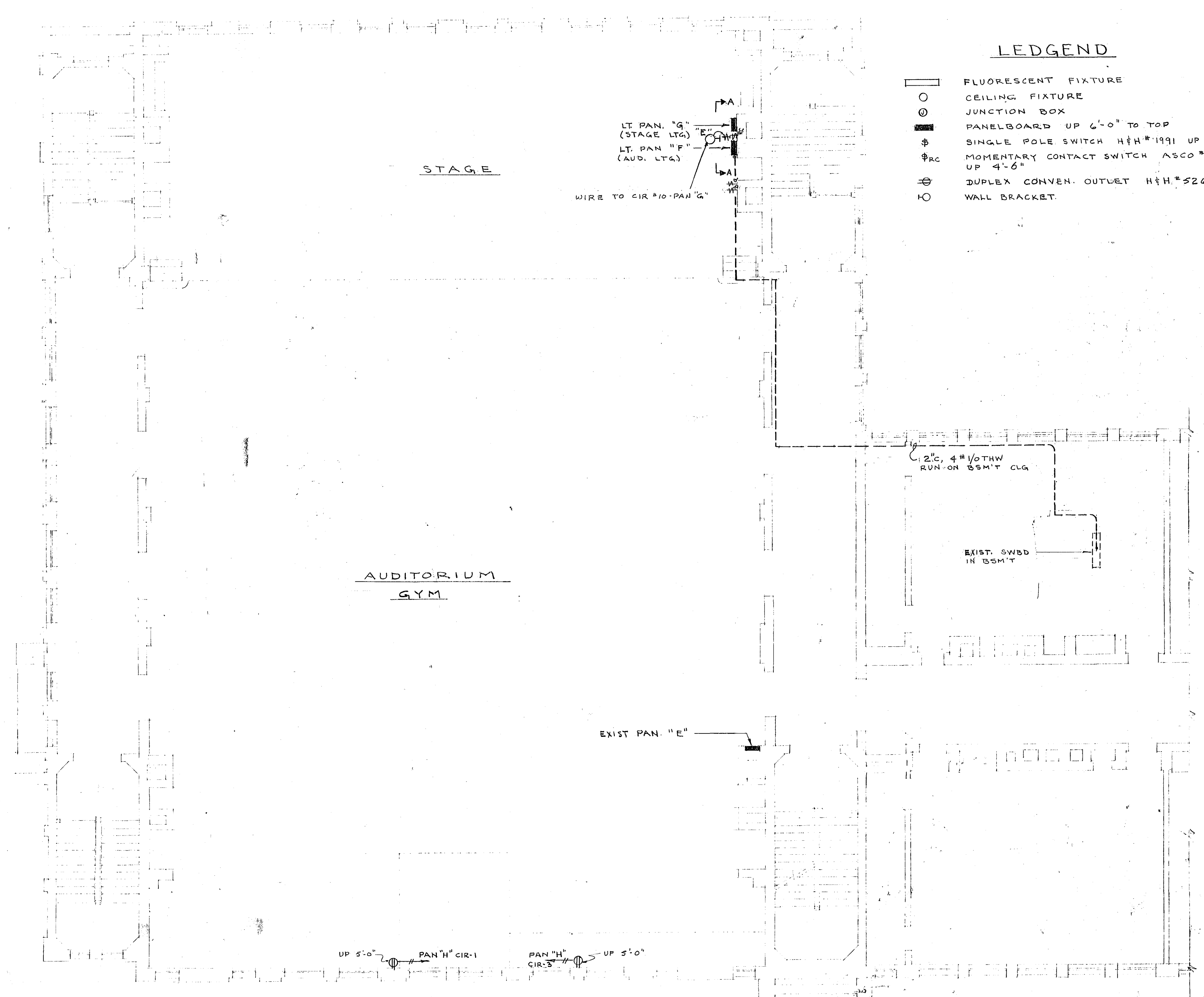
PARTIAL FIRST FLOOR PLAN SCALE 1/8" = 1' - 0"
