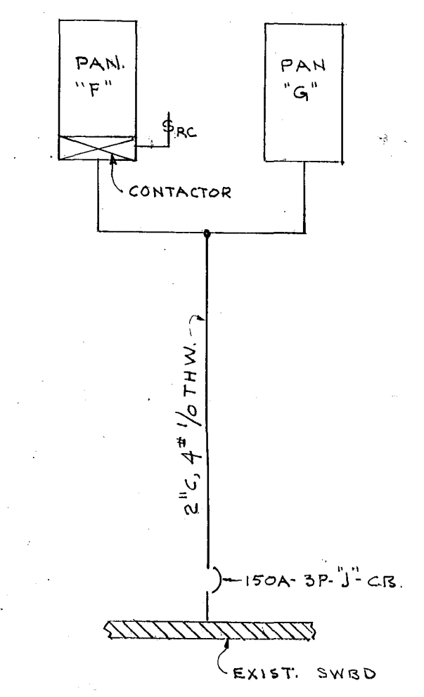
RISER DIAGRAM NO SCALE
