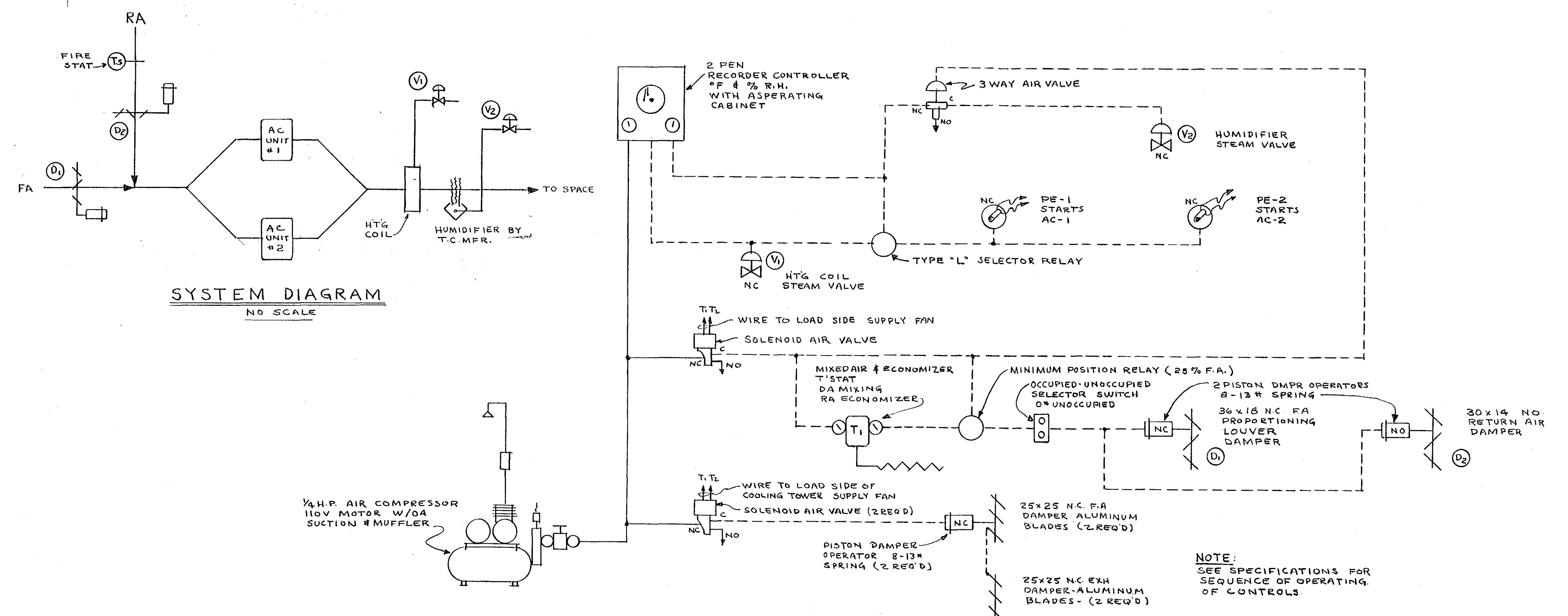
TEMPERATURE CONTROL DIAGRAMS NO SCALE
