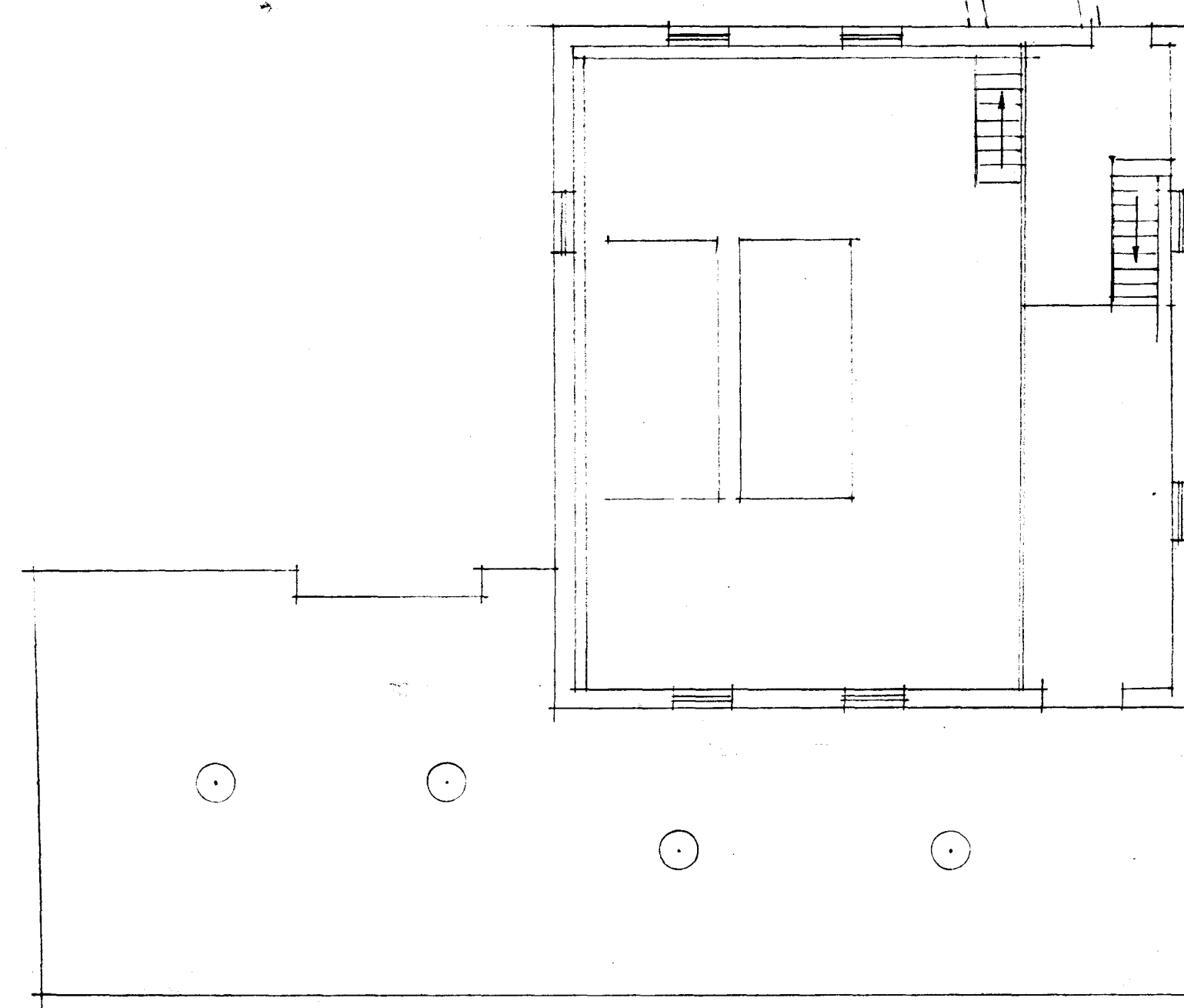
BOILER ROOM PLAN SCALE 1/8" = 1' - 0"
