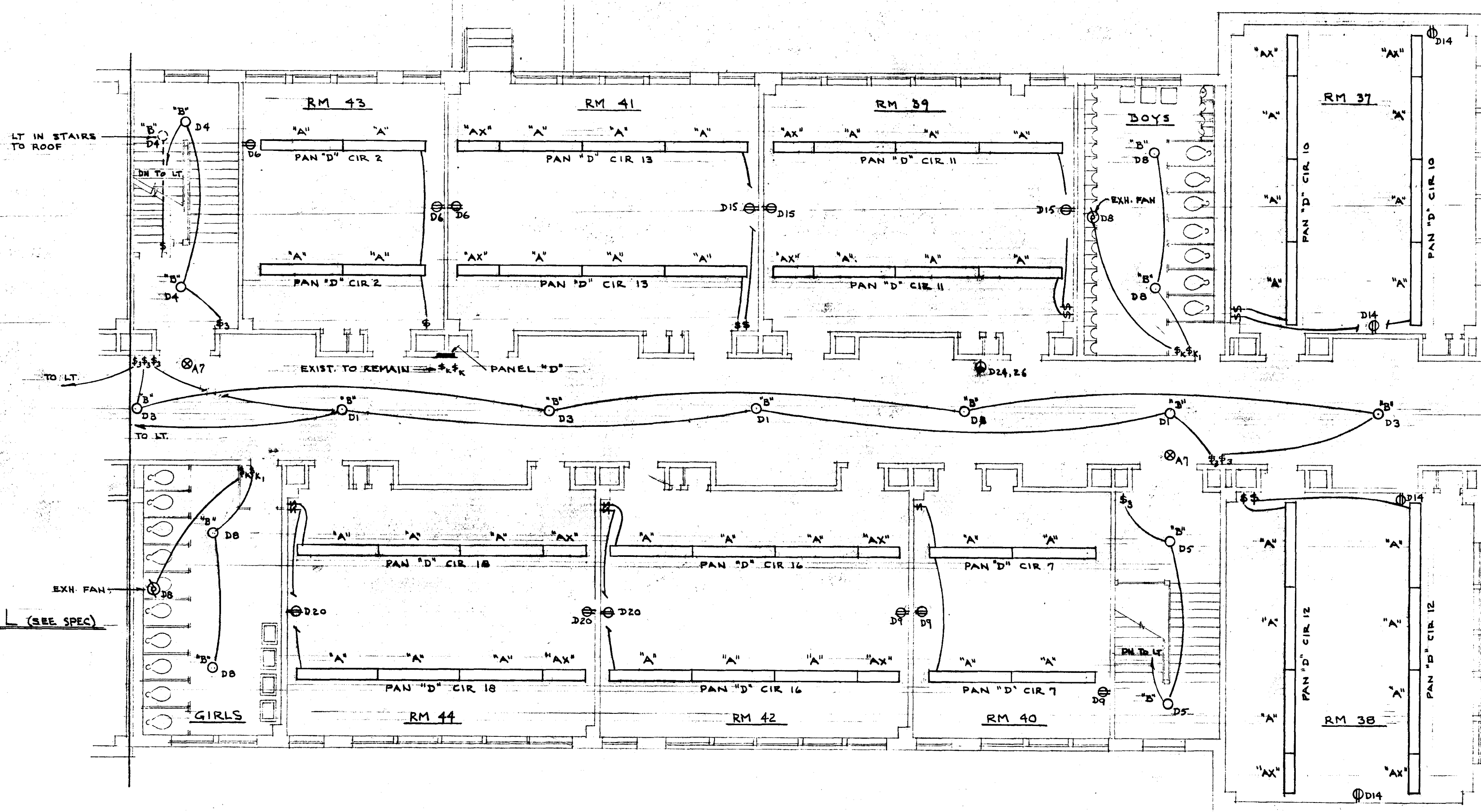
SECOND FLOOR PLAN - BLDG "B" SOUTH SECTION SCALE 1/8" = 1' - 0"
