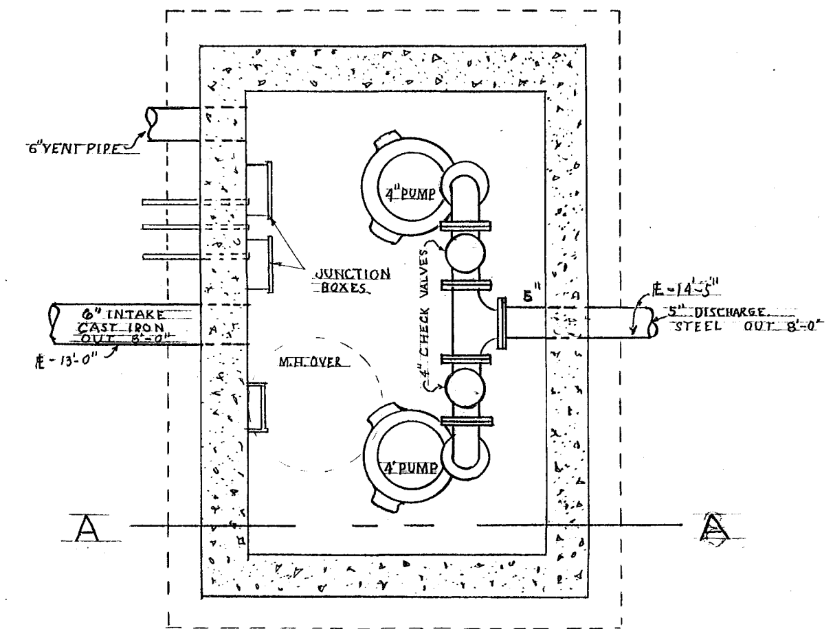
PLAN THRU PUMP STATION SCALE - 1" = 10'
