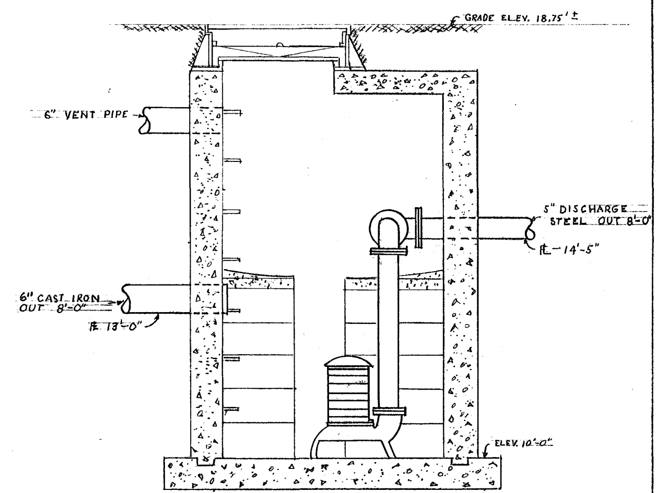
SECTION THRU A SCALE - \frac{1}{2}" = 1'-0"
