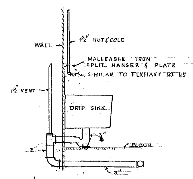
DRIP SINK DETAIL NO SCALE
