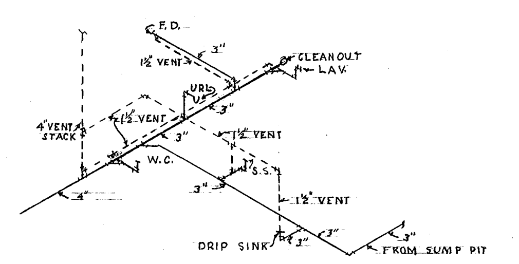
SOIL, WASTE AND VENT PIPING ISOMETRIC FOR TOILET NO SCALE
