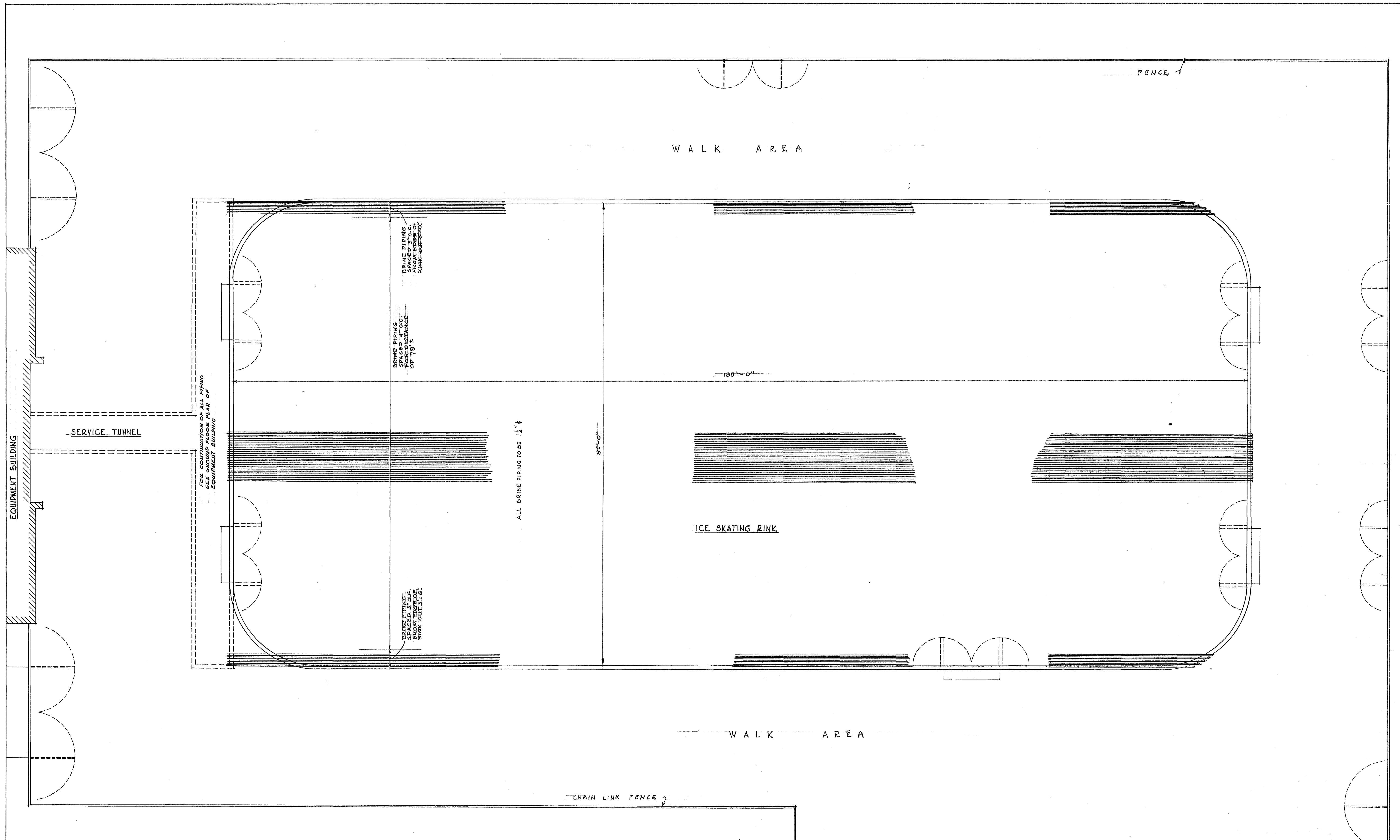
MECHANICAL REFRIGERATION PLAN OF SKATING RINK SCALE 1/8" = 1'-0"
