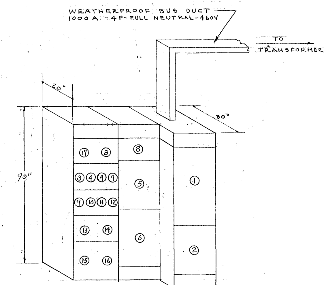
SWITCHBOARD ISOMETRIC. NO SCALE
