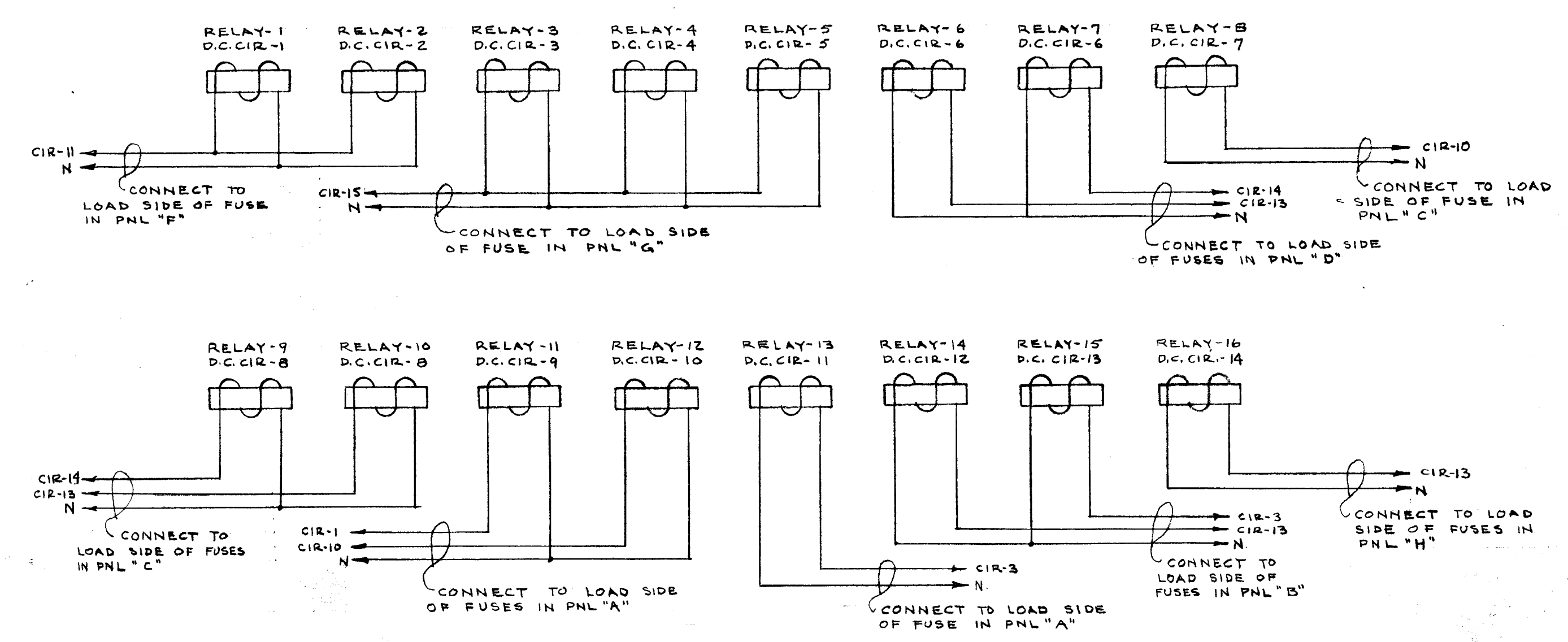
WIRING DIAGRAM OF A.C. CONTROL FOR RELAYS IN TRANSFER PANELS NO SCALE
