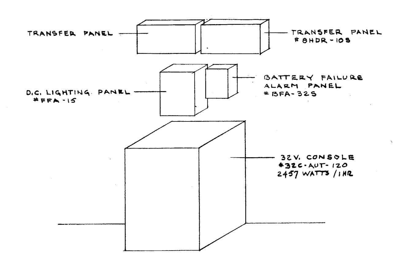
ISOMETRIC OF EMERGENCY EQUIPMENT NO SCALE
