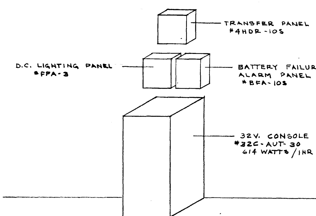
ISOMETRIC OF EMERGENCY EQUIPMENT
