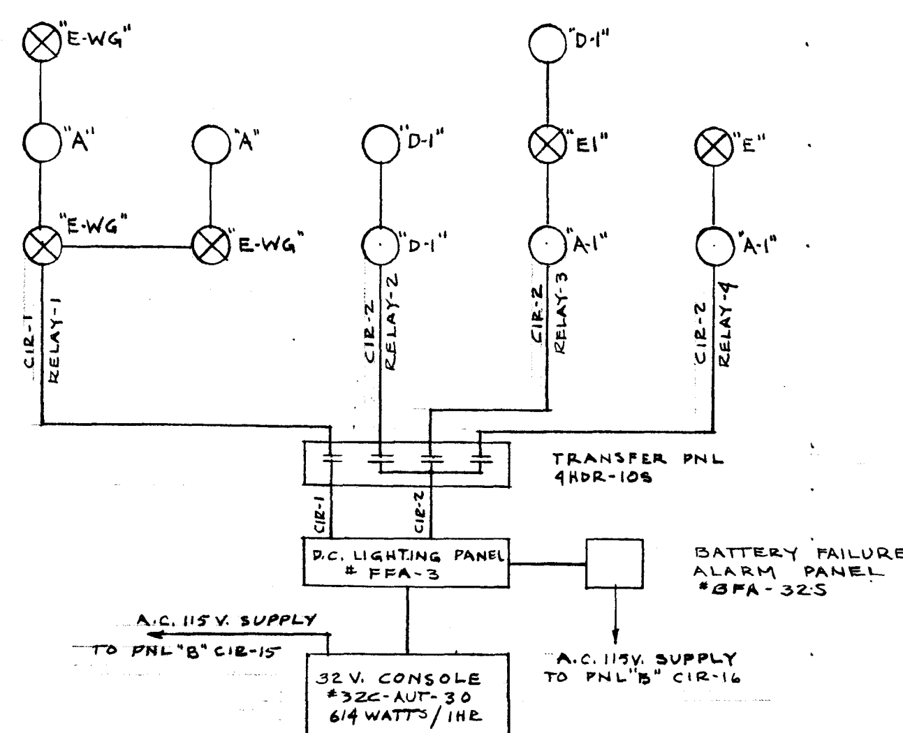
EMERGENCY LIGHTING SCHEMATIC
