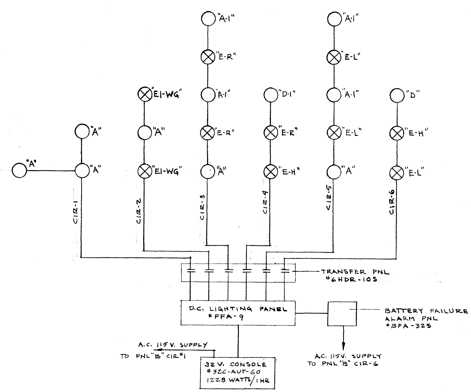
EMERGENCY LIGHTING SCHEMATIC NO SCALE
