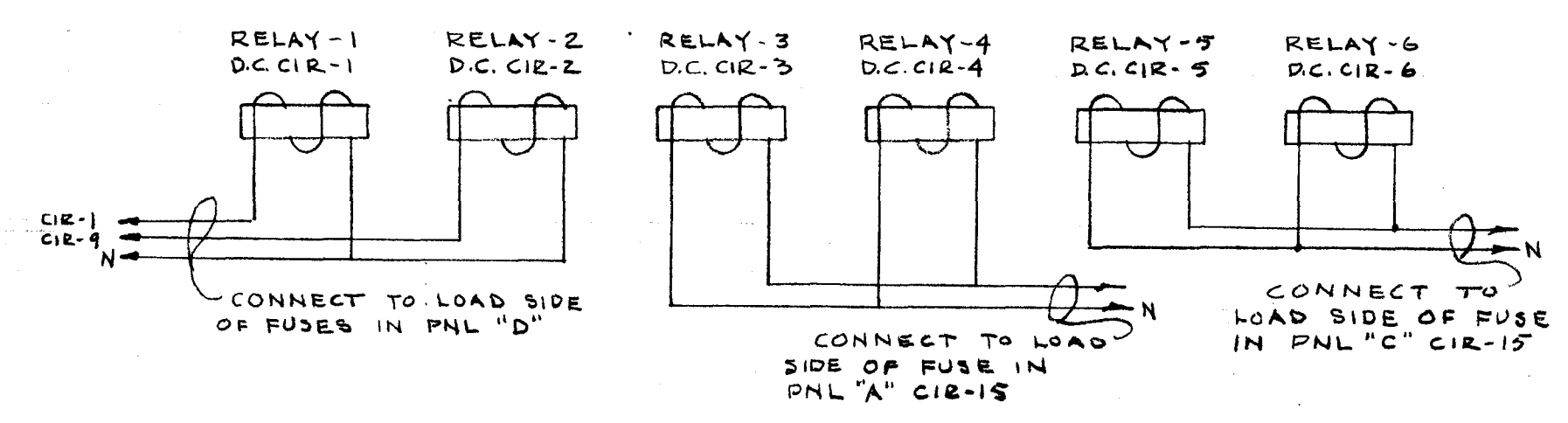
WIRING DIAGRAM FOR A.C. CONTROL OF RELAYS IN TRANSFER PANEL NO SCALE
