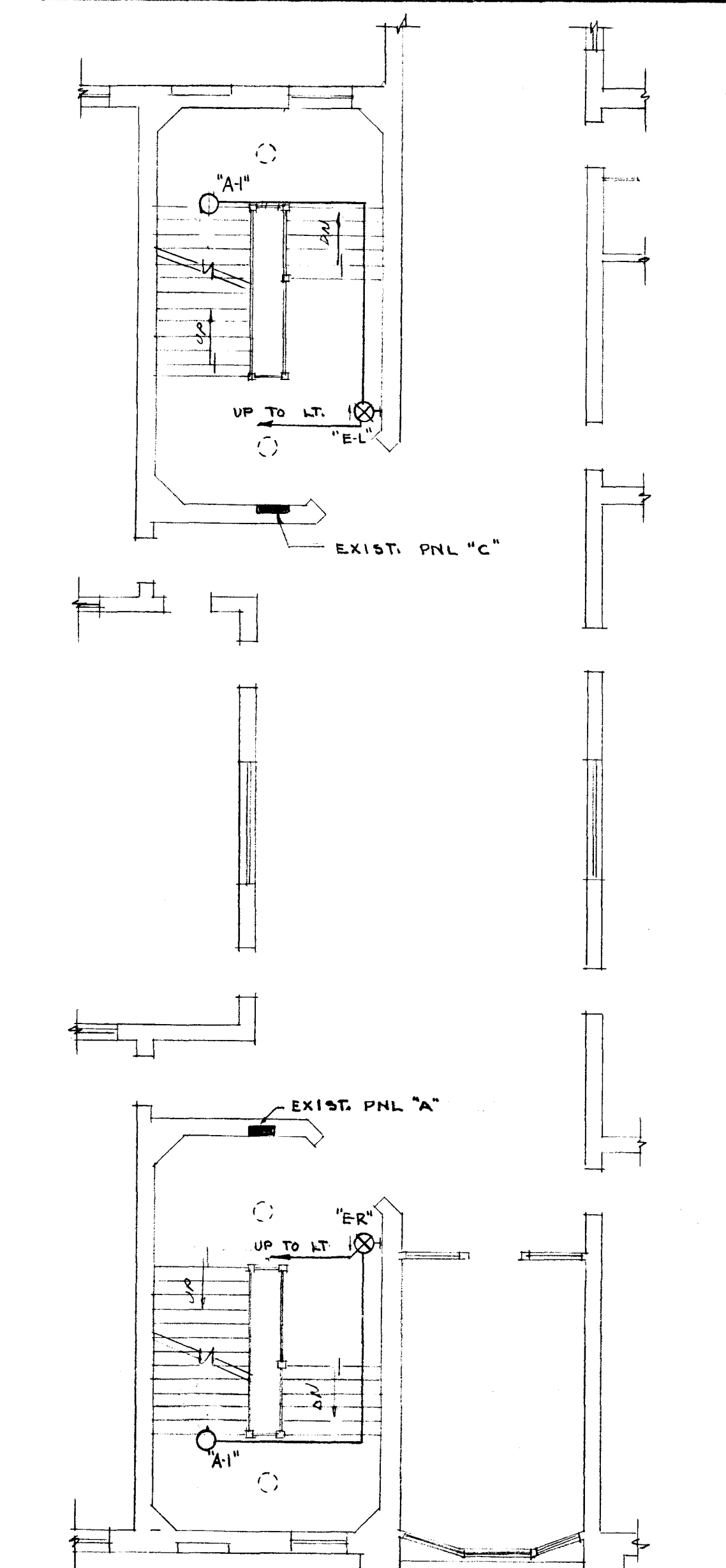
PARTIAL FIRST FLOOR PLAN SCALE 1/8" = 1'-0"
