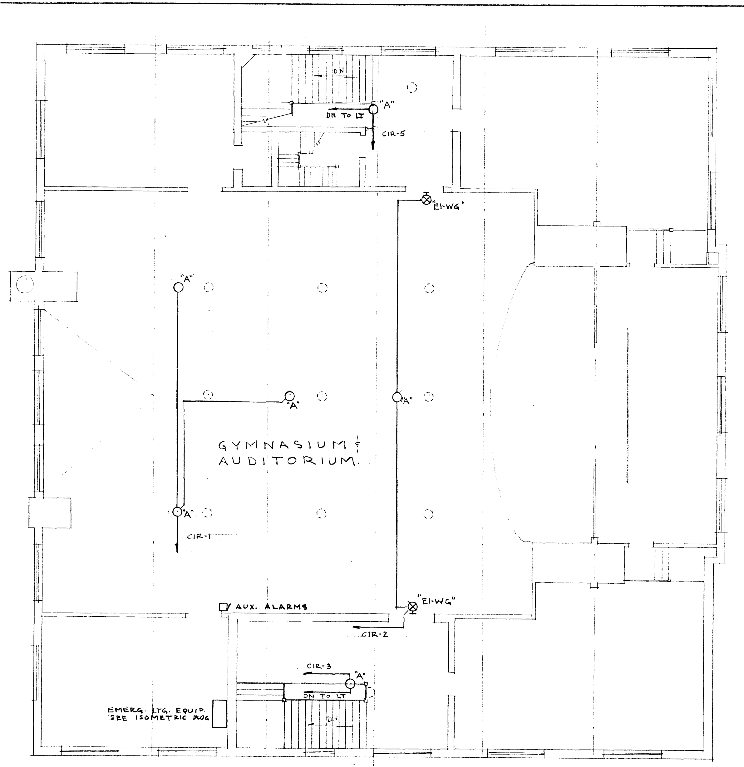
THIRD FLOOR PLAN SCALE 1/8" = 1'-0"
