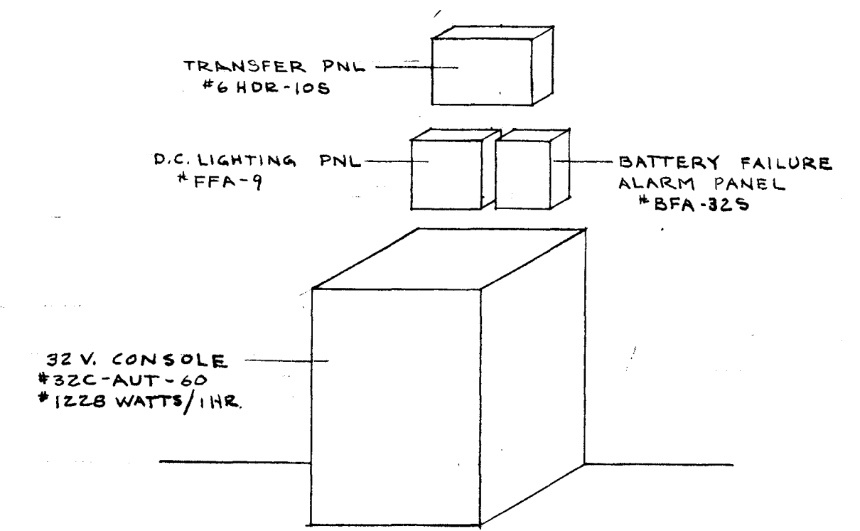
ISOMETRIC OF EMERGENCY EQUIPMENT NO SCALE
