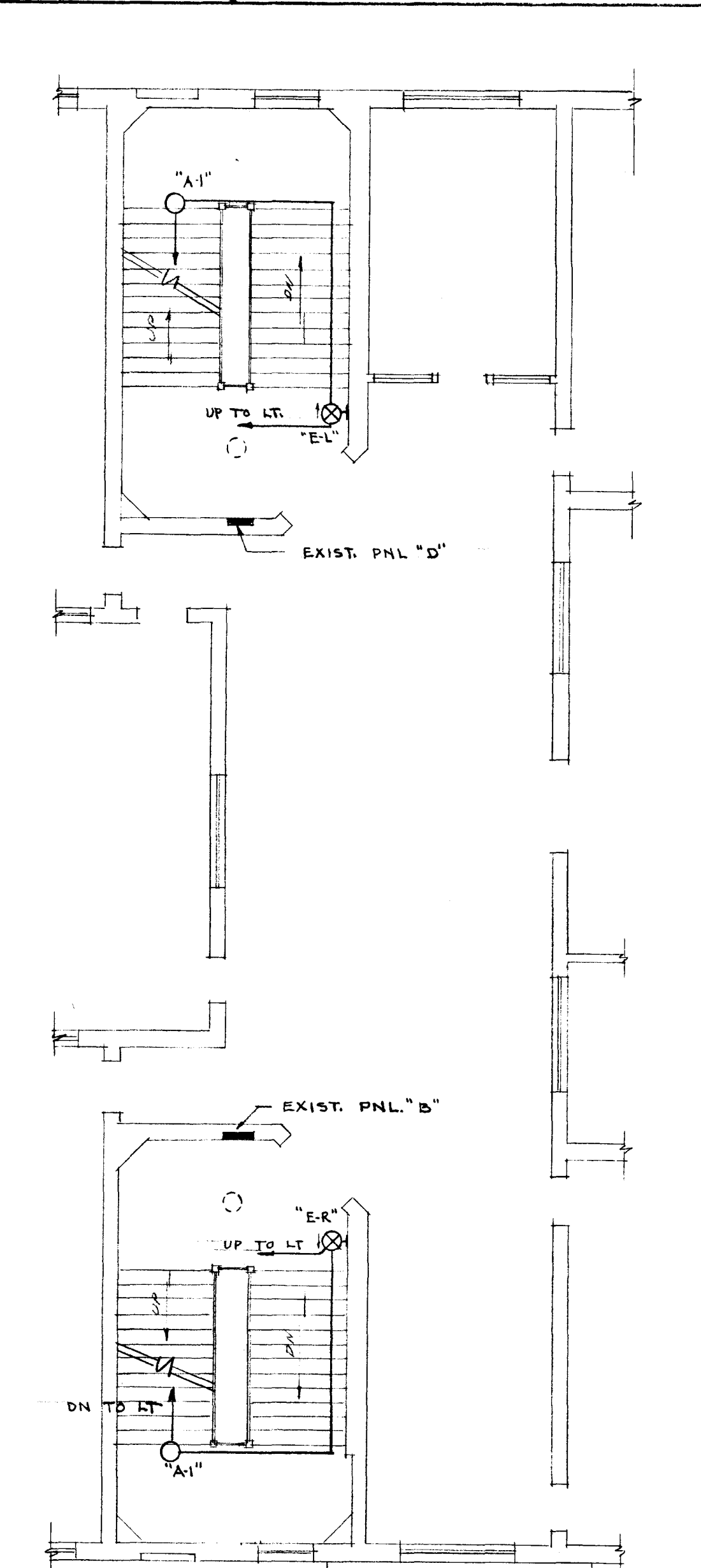
PARTIAL SECOND FLOOR PLAN SCALE 1/8" = 1'-0"
