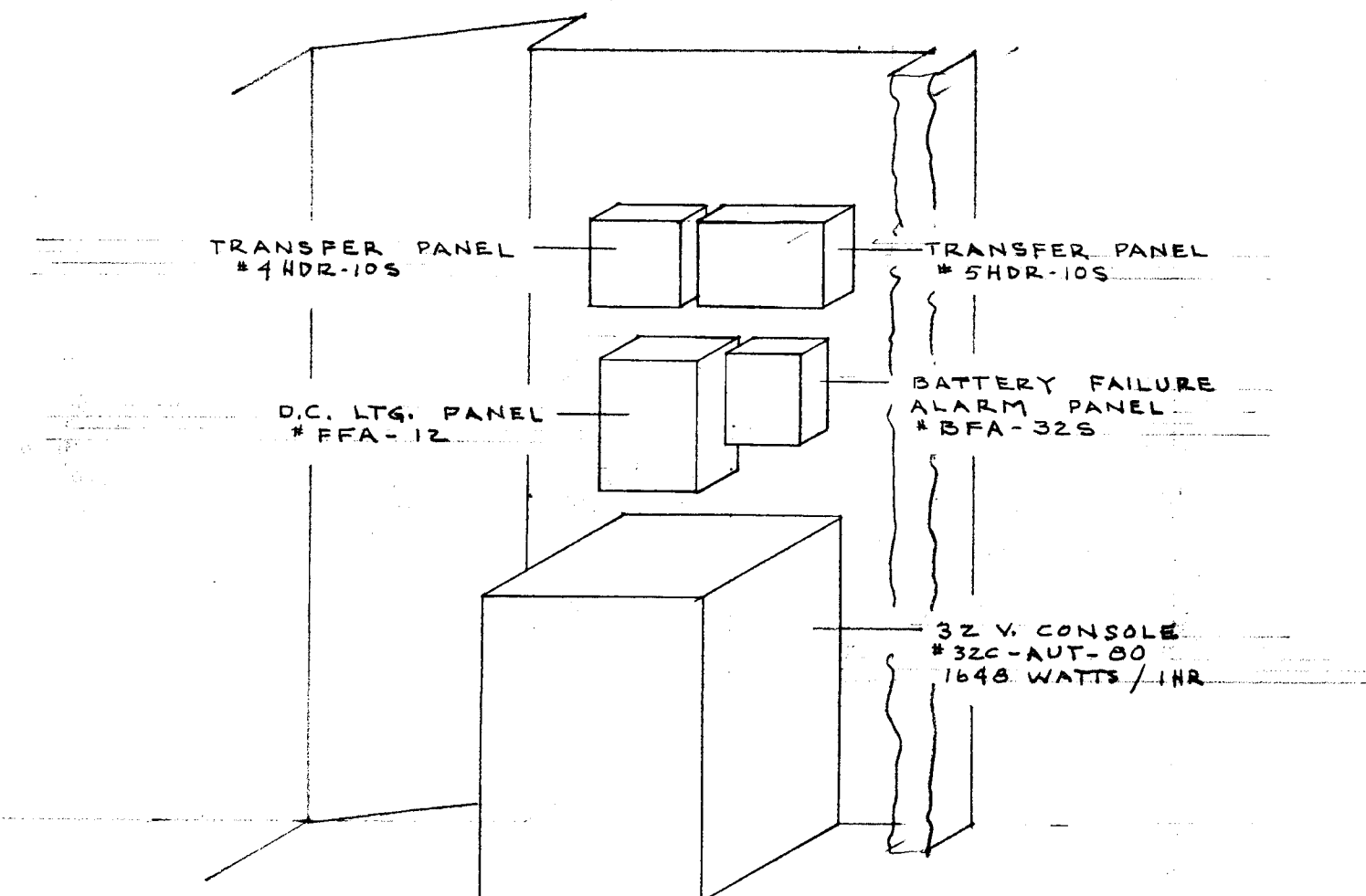
ISOMETRIC OF EMERGENCY EQUIPMENT
