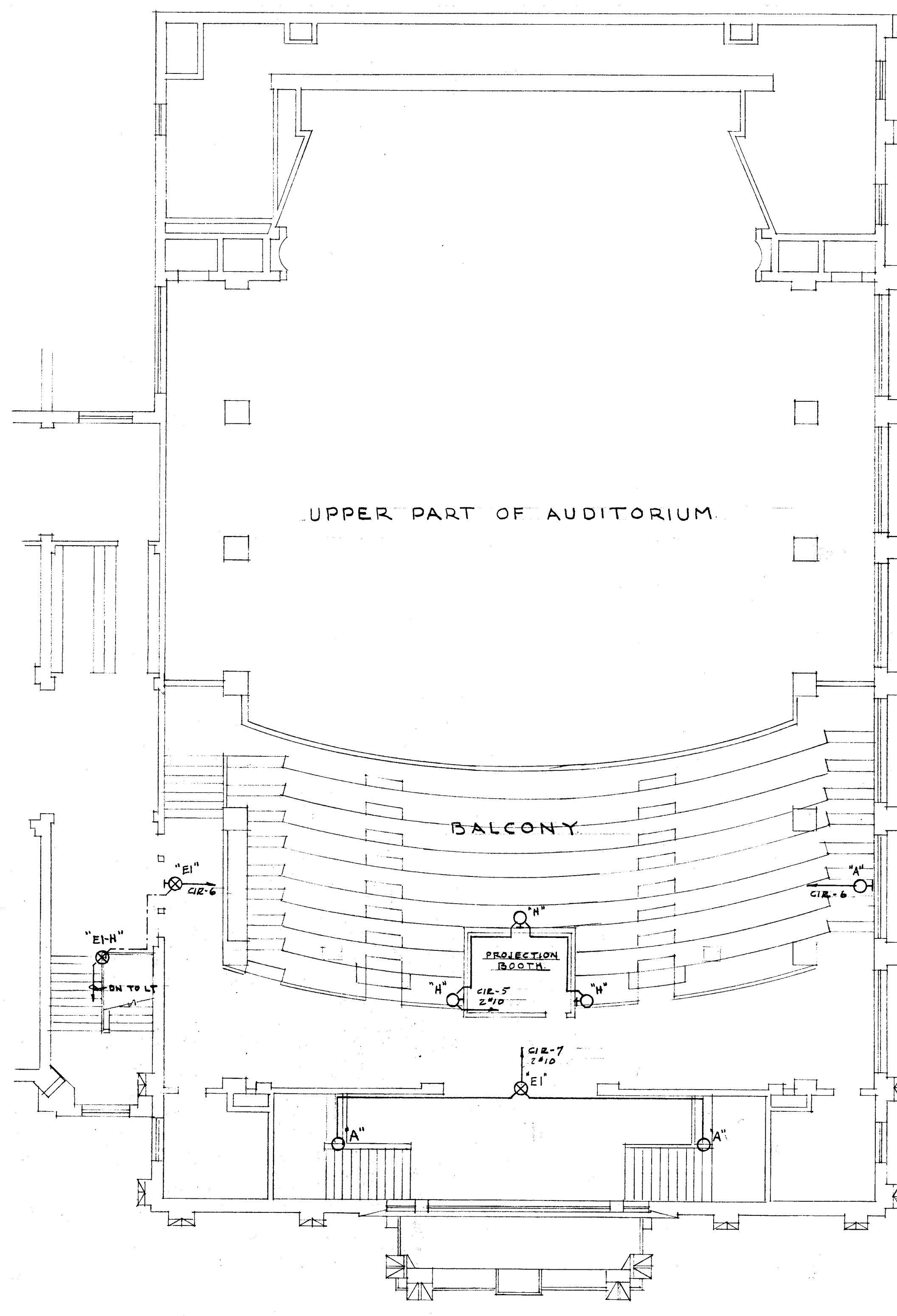
BALCONY (2ND FL.) PLAN
