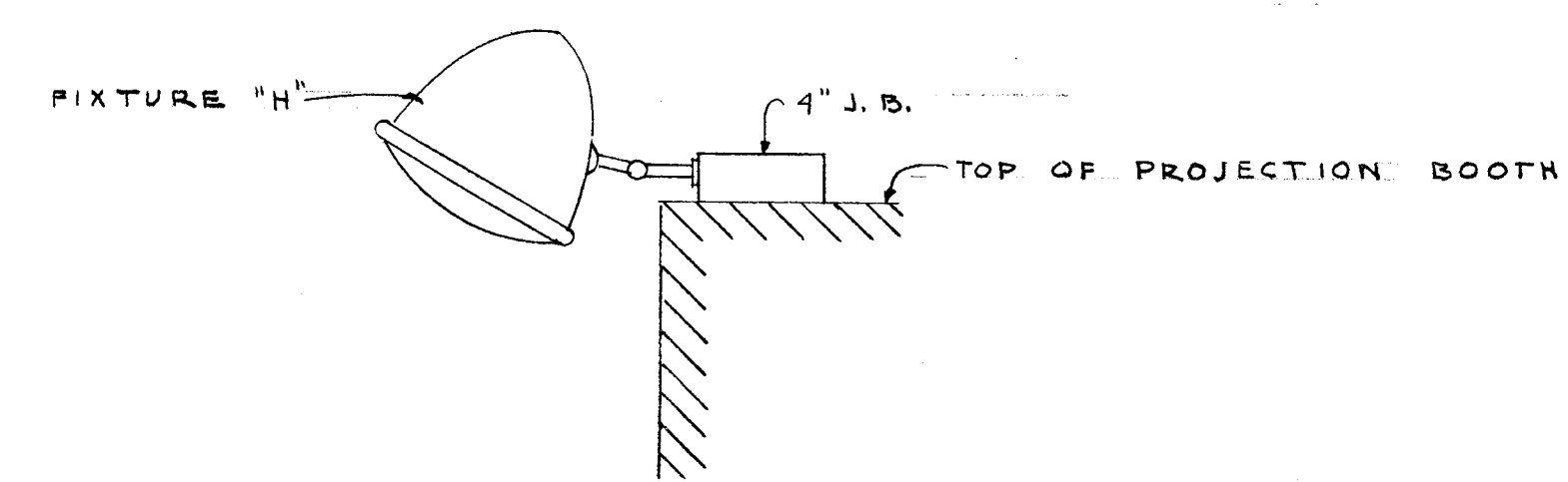
FIXTURE "H" MTG. DETAIL
