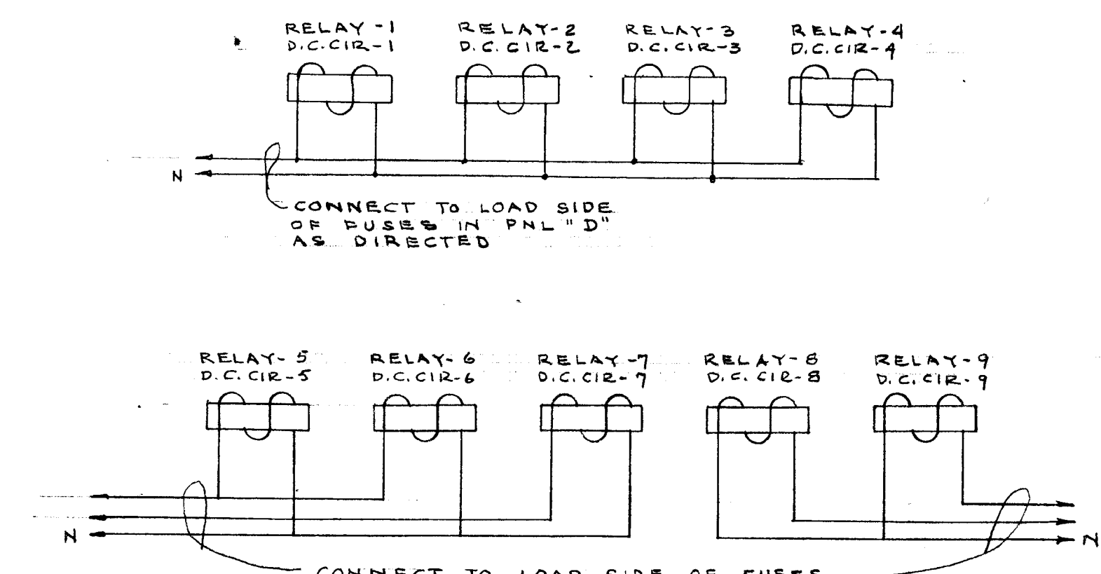
WIRING DIAGRAM OF A.C. CONTROL FOR RELAYS IN TRANSFER PANELS
