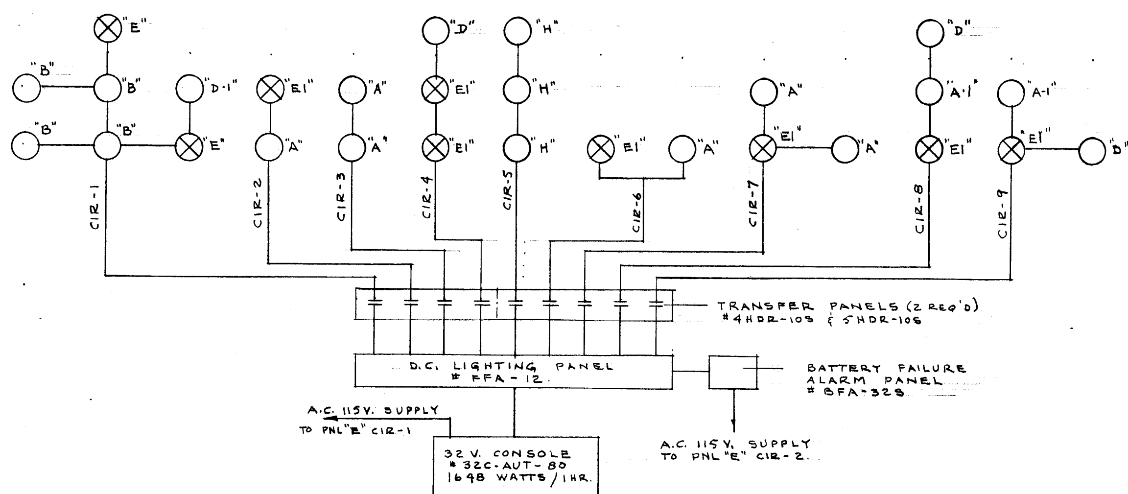
EMERGENCY LIGHTING SCHEMATIC
