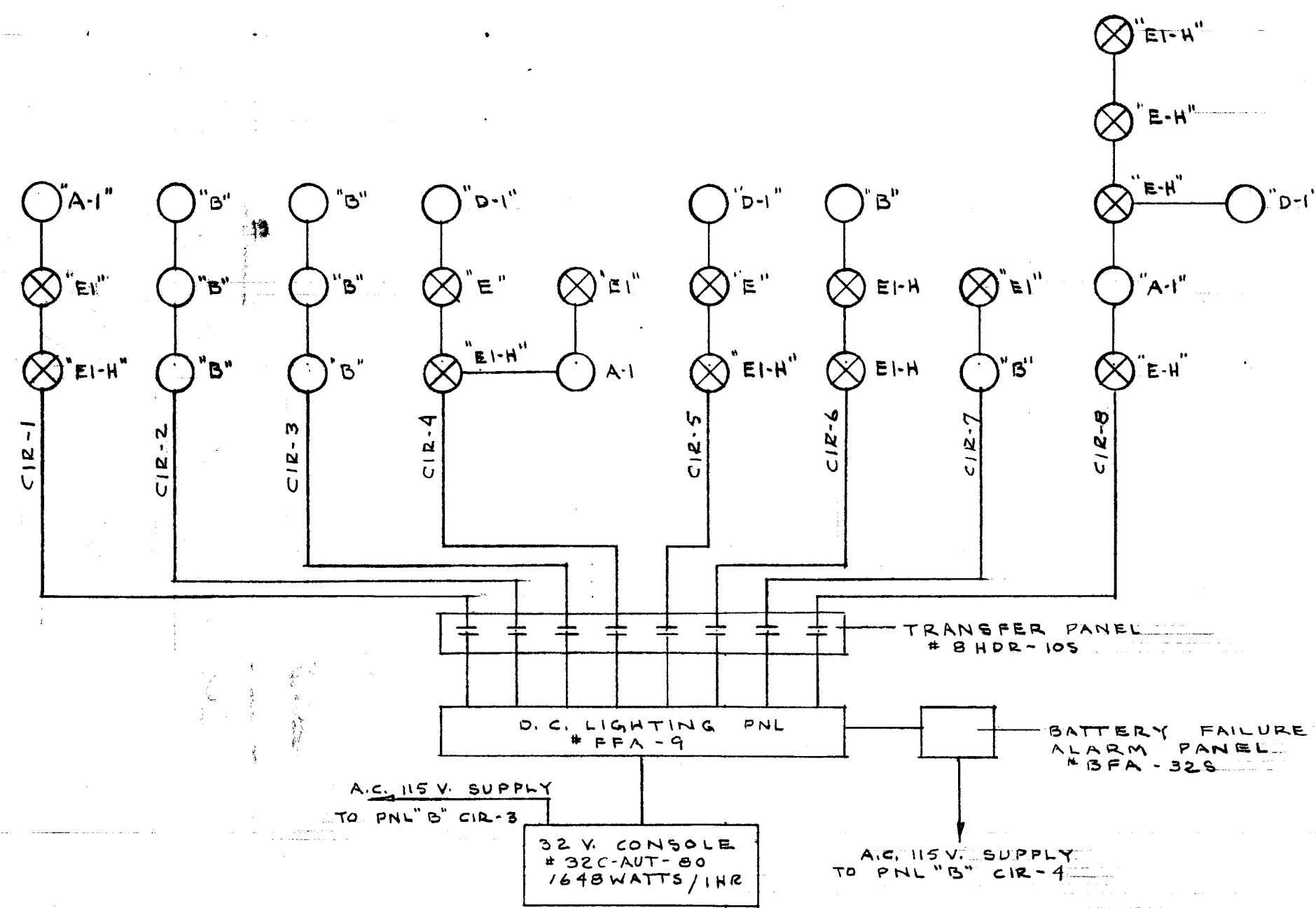
EMERGENCY LIGHTING SCHEMATIC NO SCALE
