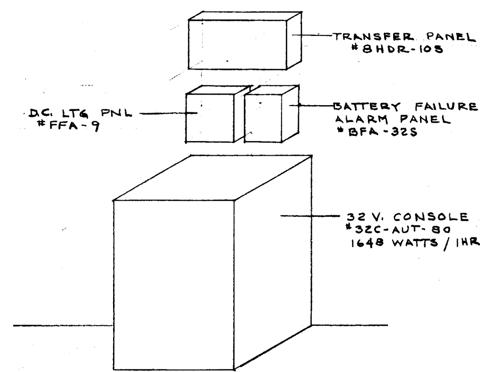
ISOMETRIC OF EMERGENCY EQUIPMENT NO SCALE
