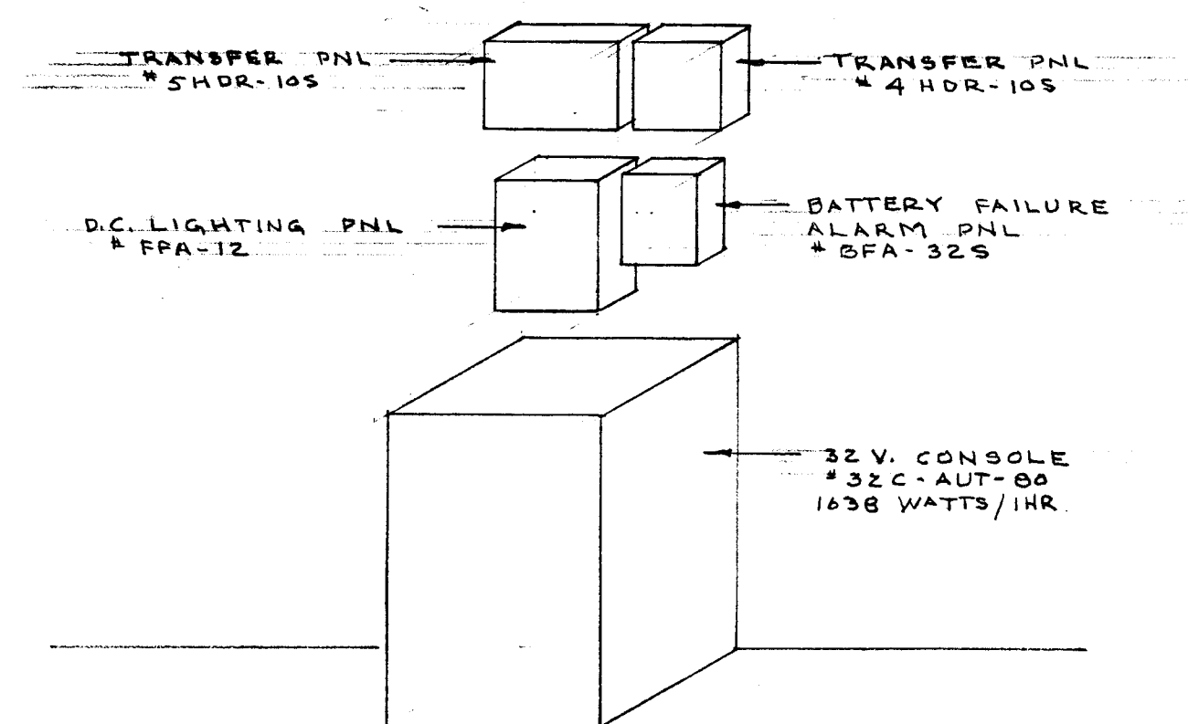
ISOMETRIC OF EMERGENCY EQUIPMENT NO SCALE
