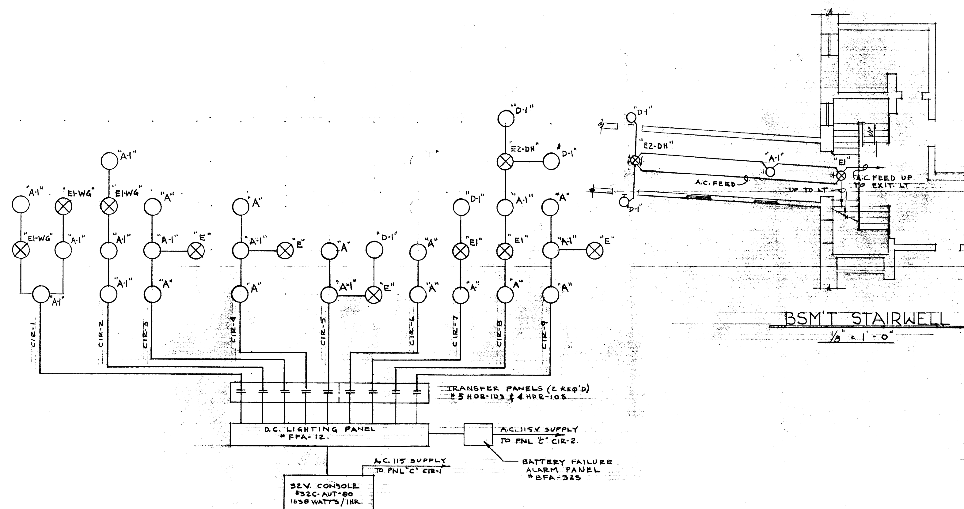
EMERGENCY LIGHTING SCHEMATIC NO SCALE
