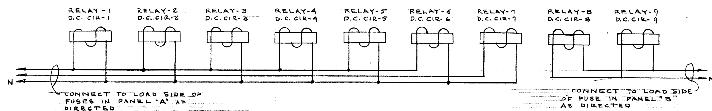
WIRING DIAGRAM OF A.C. CONTROL FOR RELAYS IN TRANSFER PANELS NO SCALE
