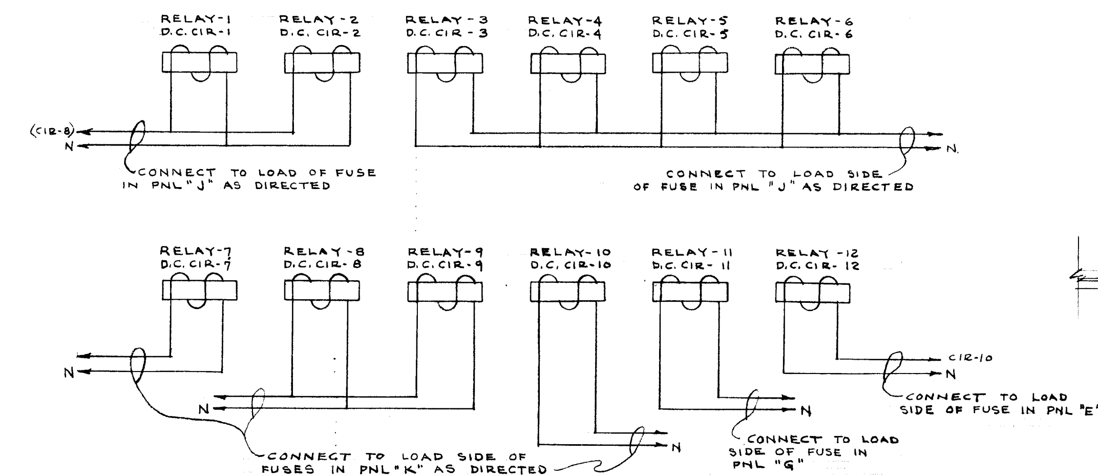
WIRING DIAGRAM OF A.C. CONTROL FOR RELAYS IN TRANSFER PANELS NO SCALE
