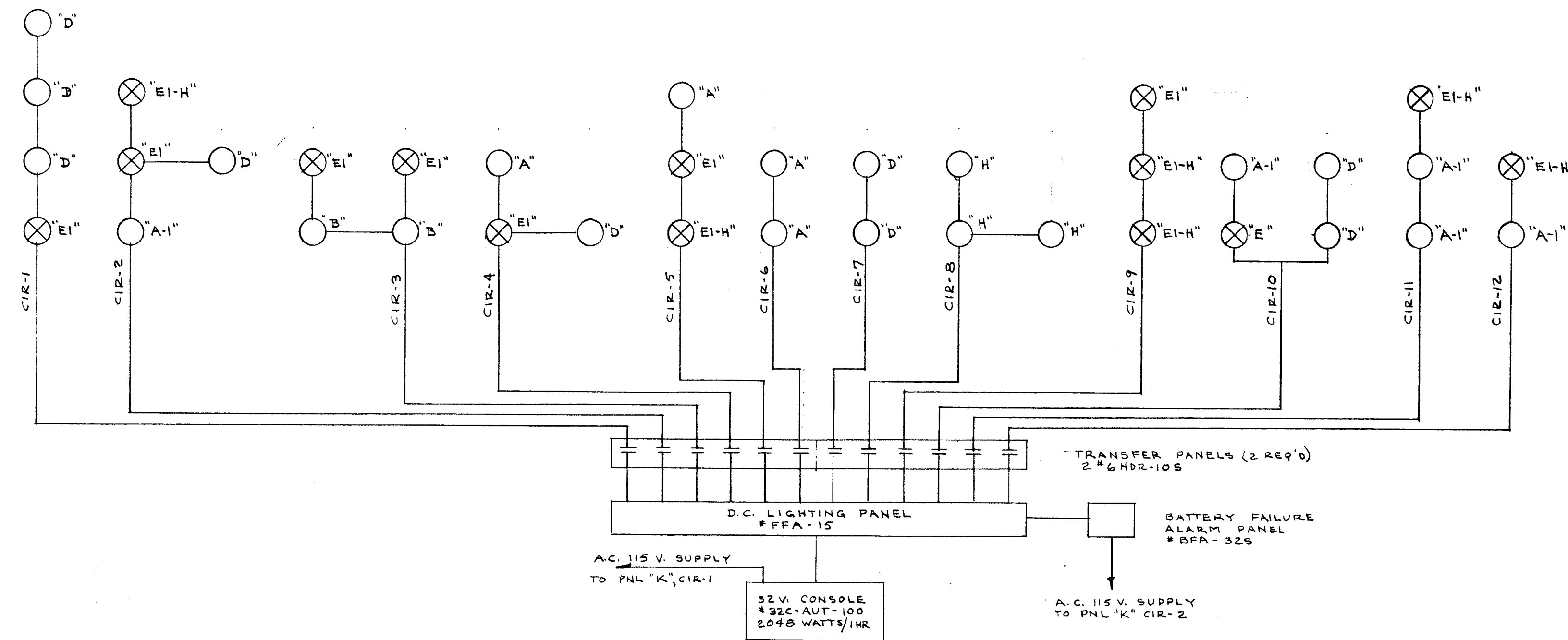
EMERGENCY LIGHTING SCHEMATIC NO SCALE
