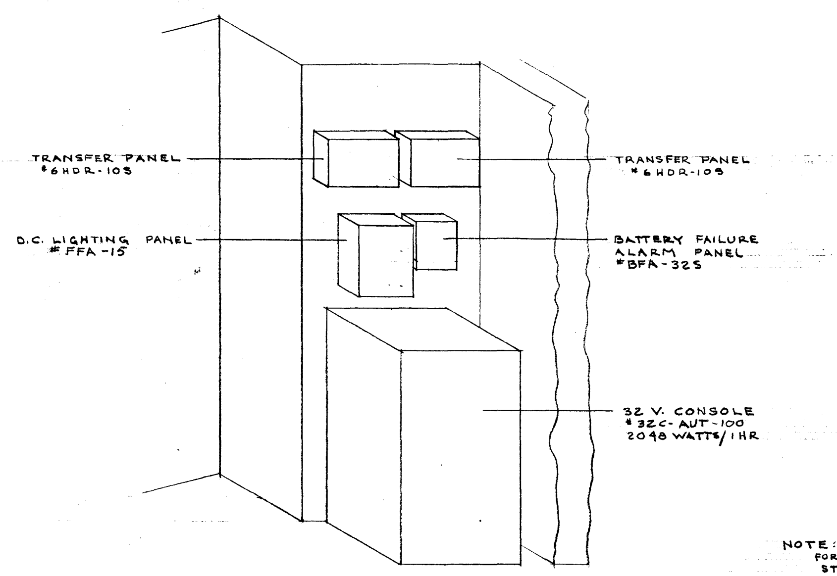
ISOMETRIC OF EMERGENCY EQUIPMENT NO SCALE
