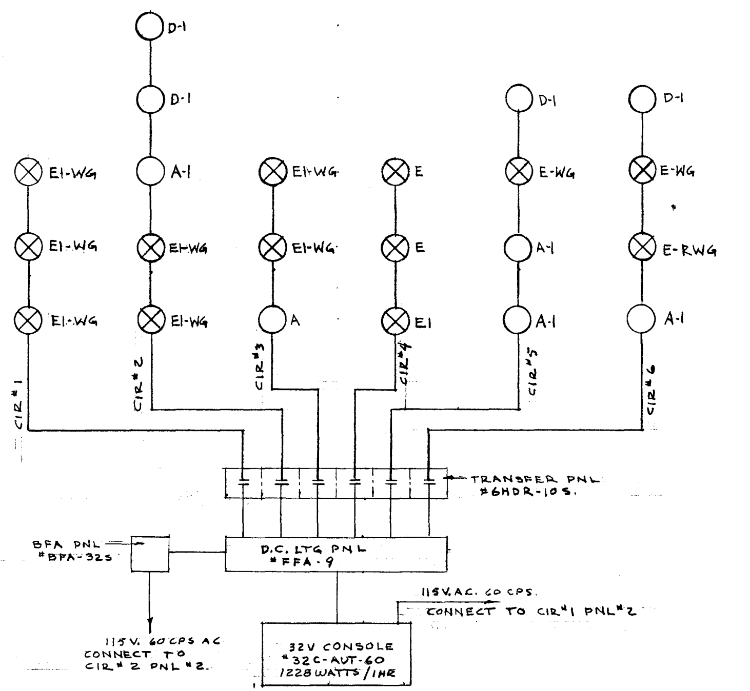
EMERGENCY LIGHTING SCHEMATIC NO SCALE
