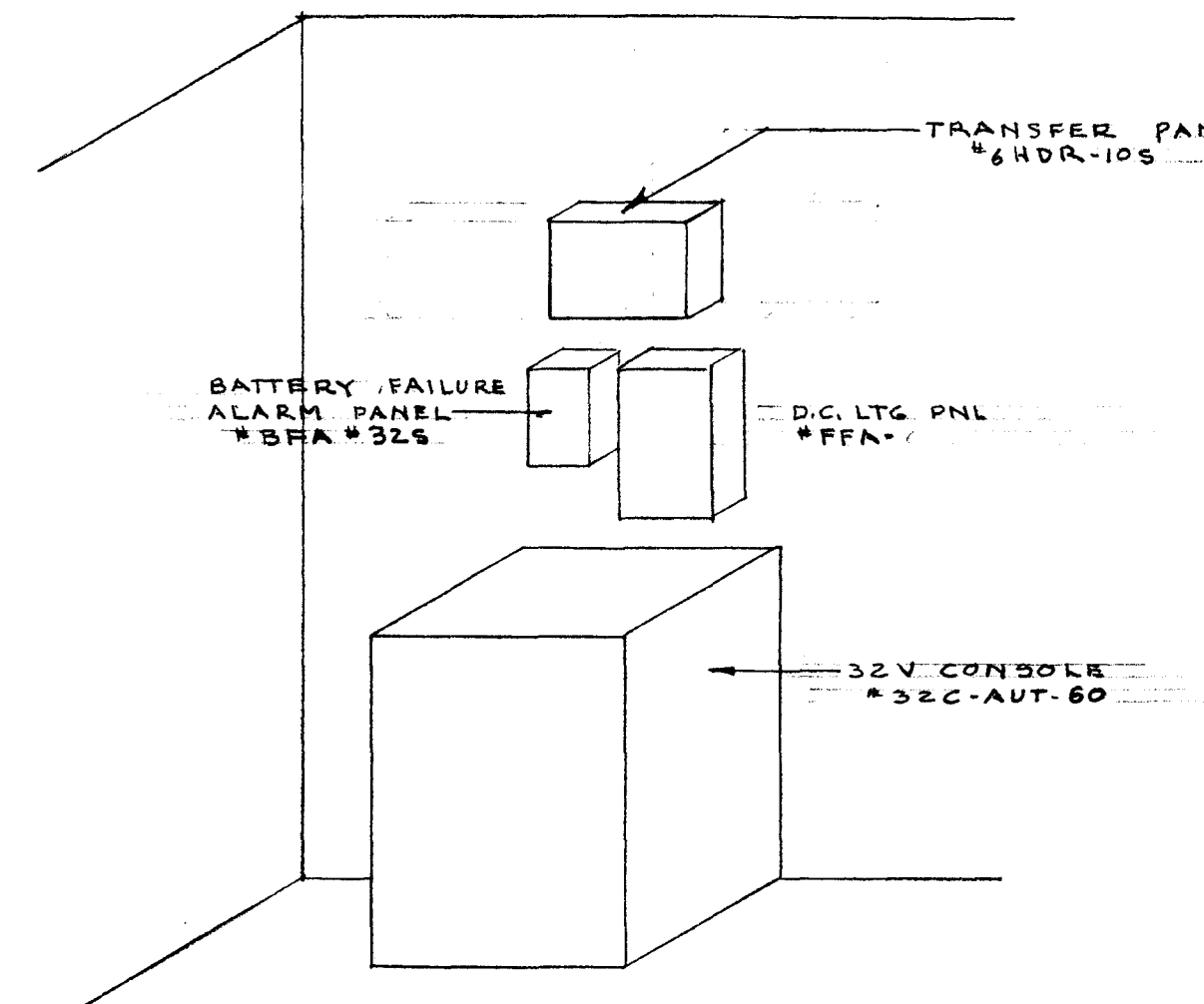
ISOMETRIC OF EMERGENCY EQUIPMENT NO SCALE
