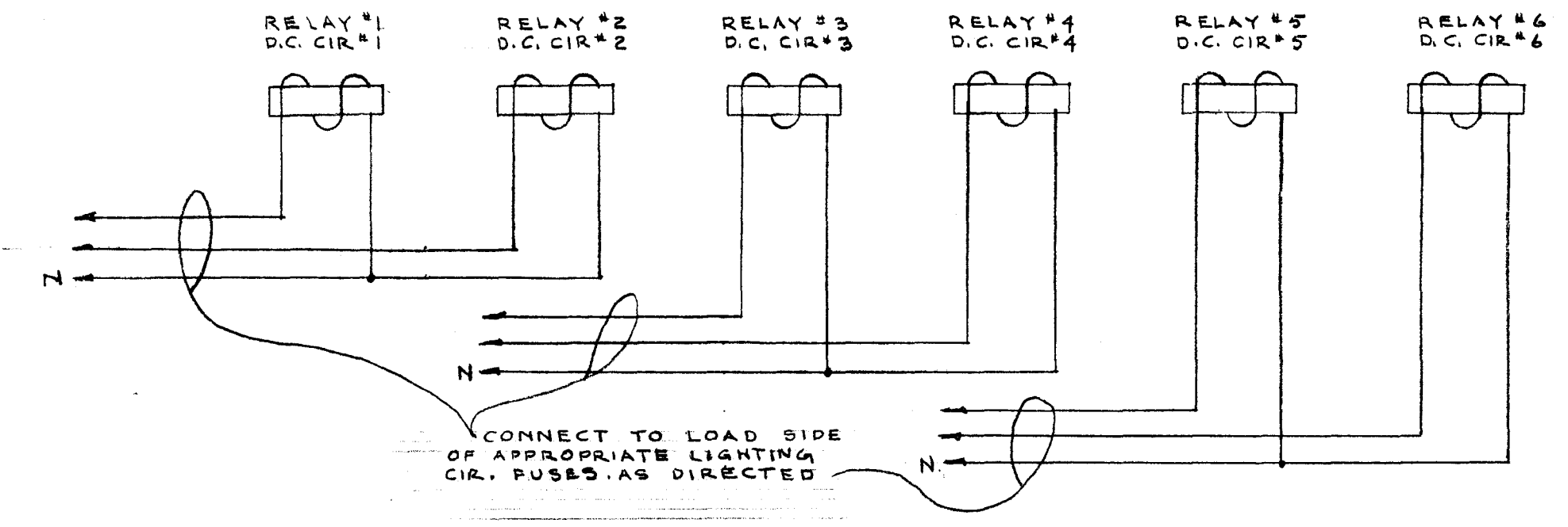
WIRING DIAGRAM OF A.C. CONTROL FOR RELAYS IN TRANSFER PANELS NO SCALE
