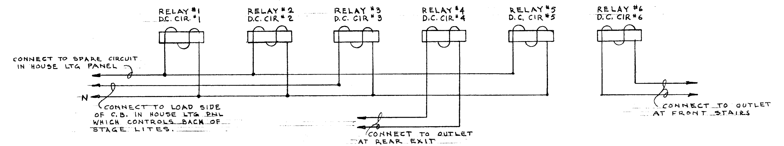
WIRING DIAGRAM OF A.C. CONTROL FOR RELAYS IN TRANSFER PANELS NO SCALE
