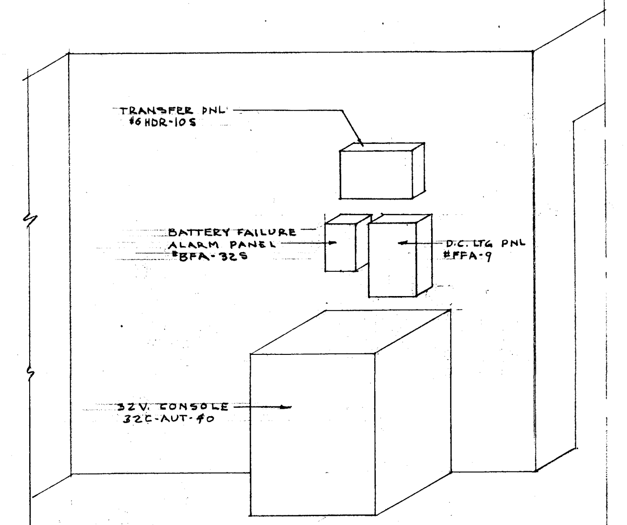
ISOMETRIC OF EMERGENCY EQUIPMENT NO SCALE
