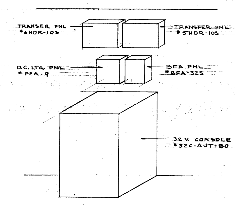
ISOMETRIC OF EMERGENCY EQUIPMENT NO SCALE
