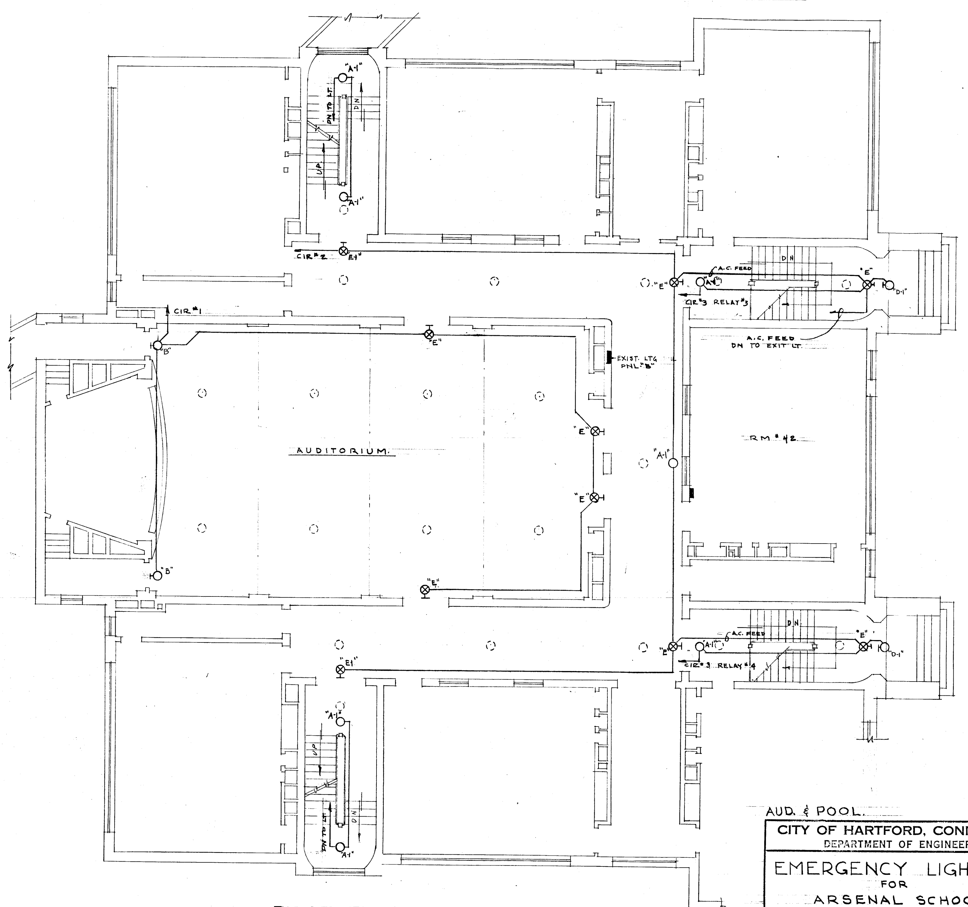
FIRST FLOOR PLAN SCALE 1/8" = 1'-0"
