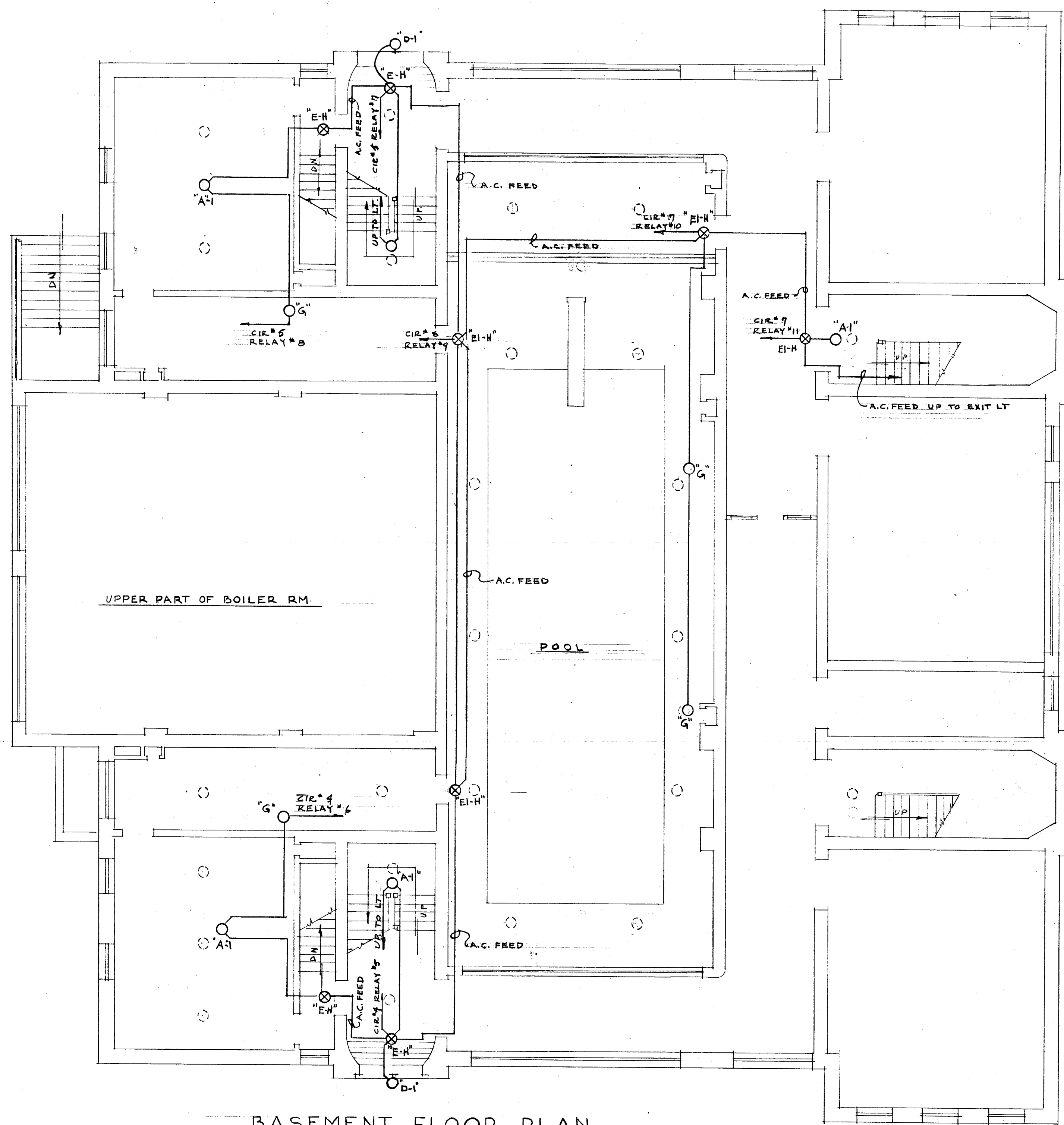
BASEMENT FLOOR PLAN SCALE 1/8" = 1'-0"
