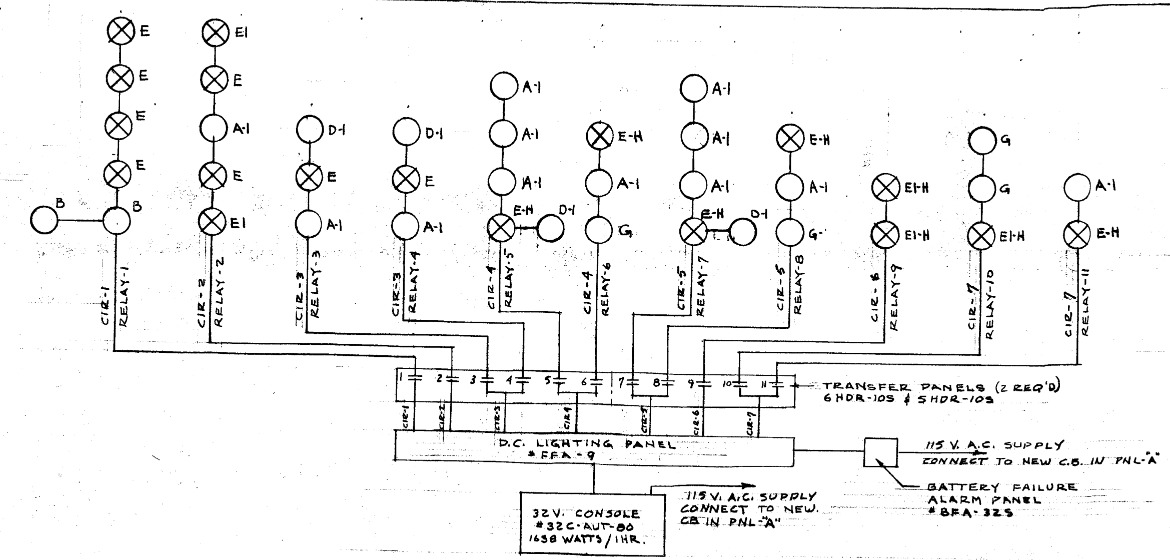
EMERGENCY LIGHTING SCHEMATIC NO SCALE
