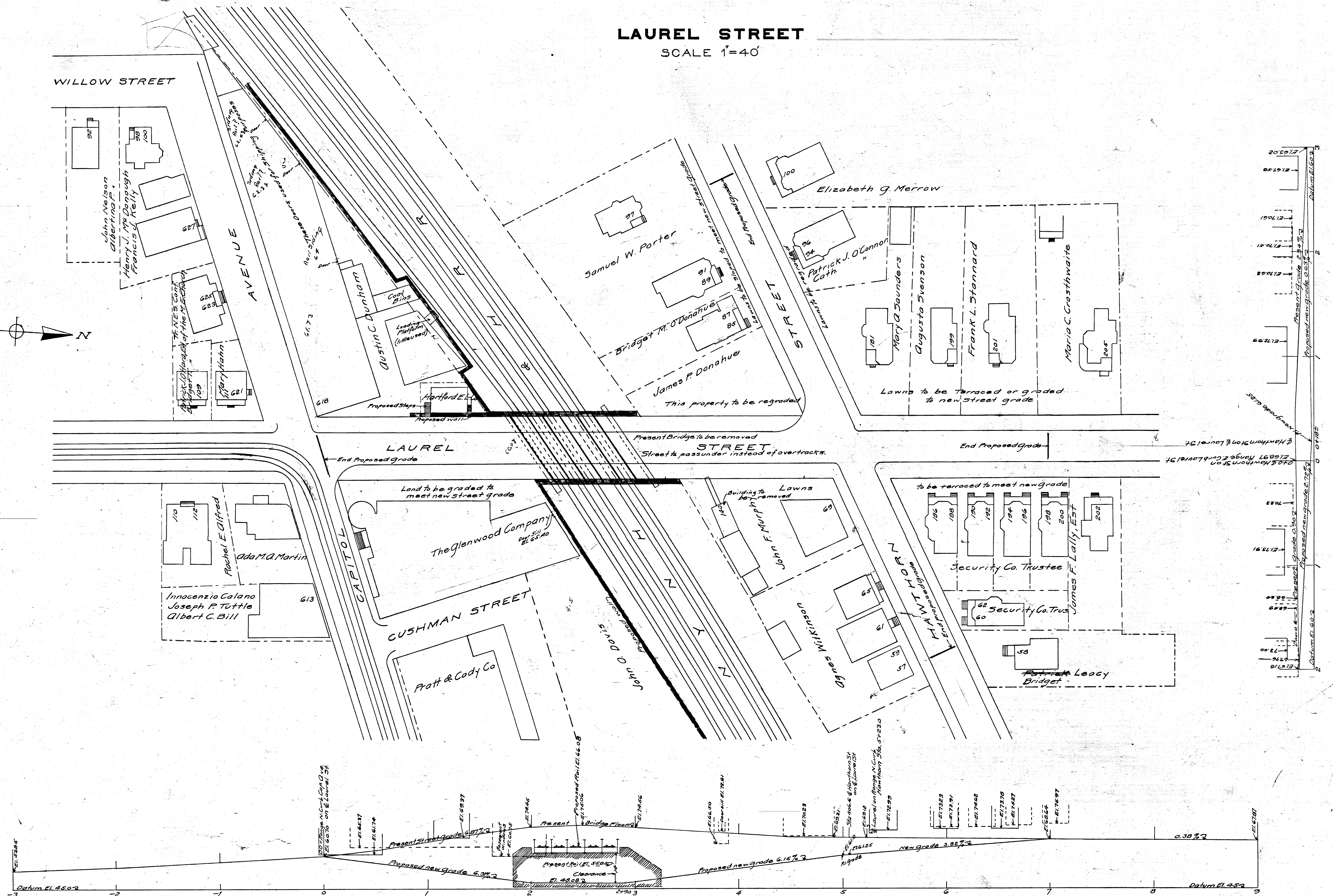
Profile of Laurel Street Horizontal Scale One inch = 40 feet Vertical Scale One inch = 20 feet Watertables of Buildings on West Side indicated by full lines East Side indicated by dash lines
