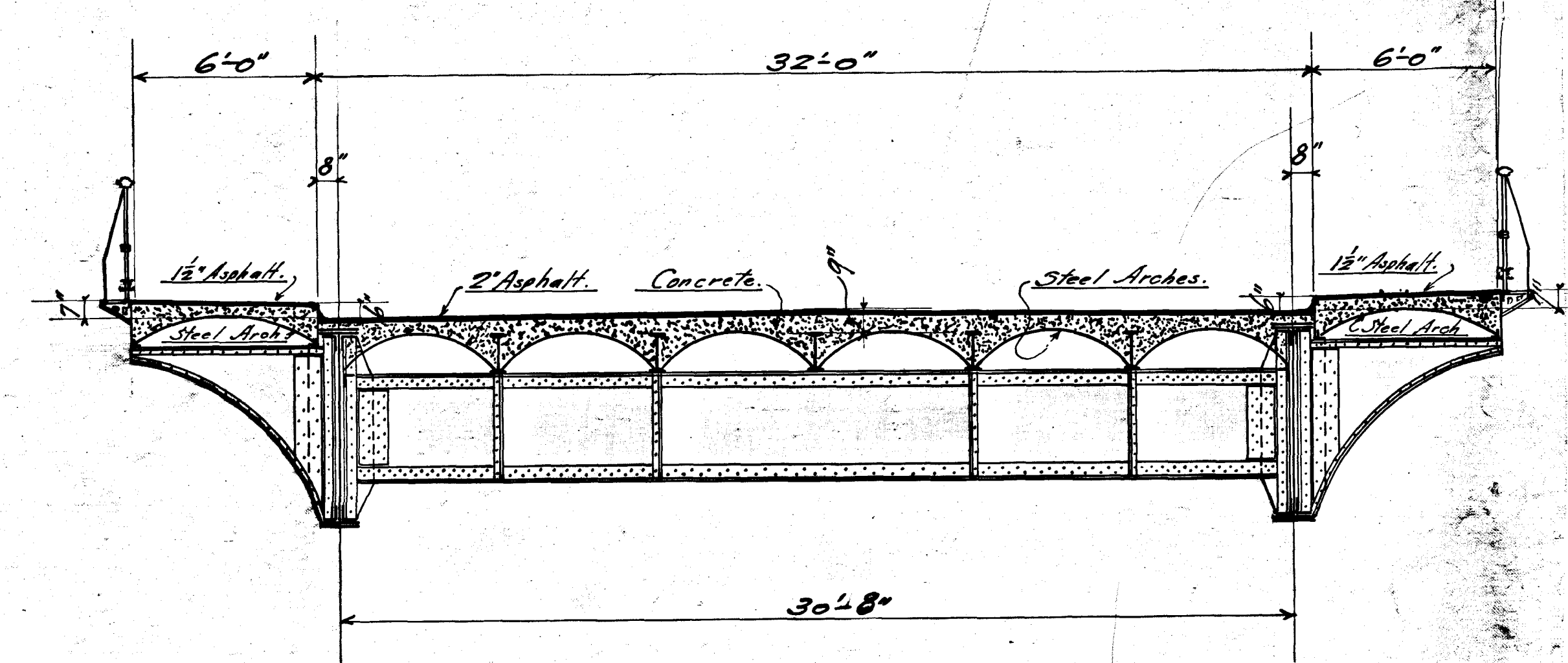
Cross Section with Steel Arch Floor
