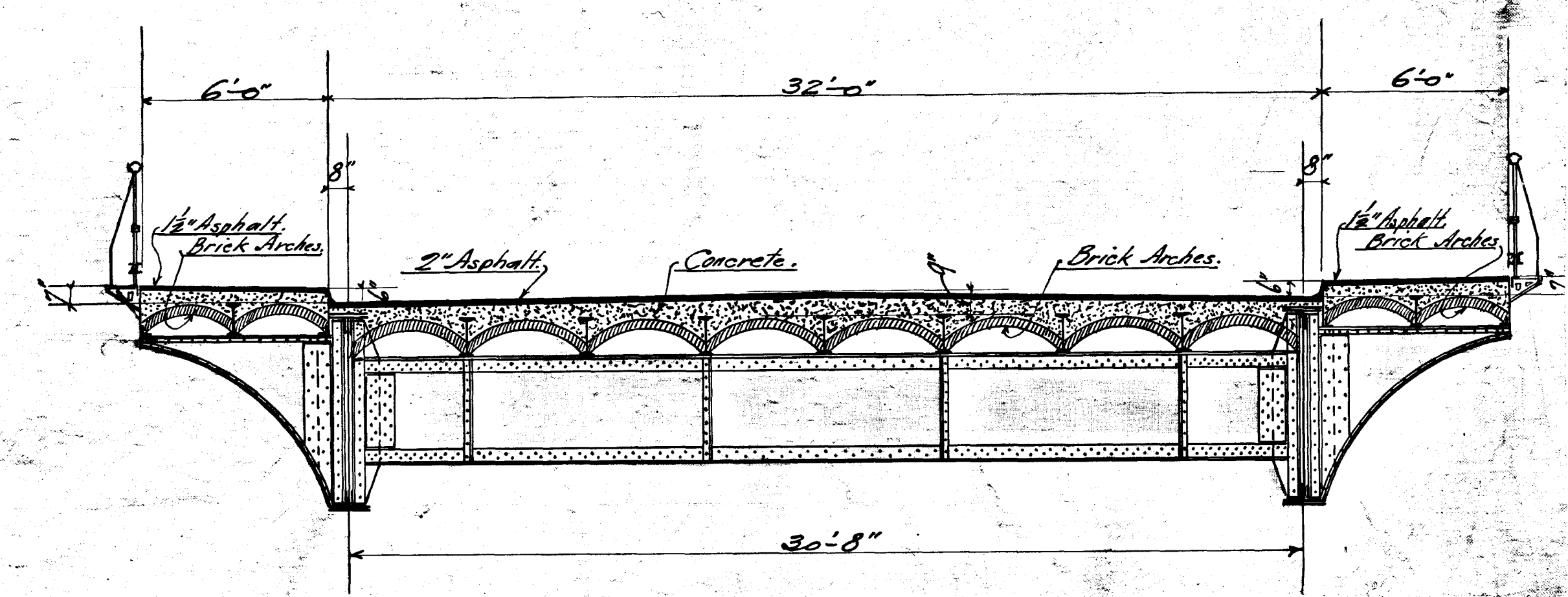
Cross Section with Brick Arch Floor
