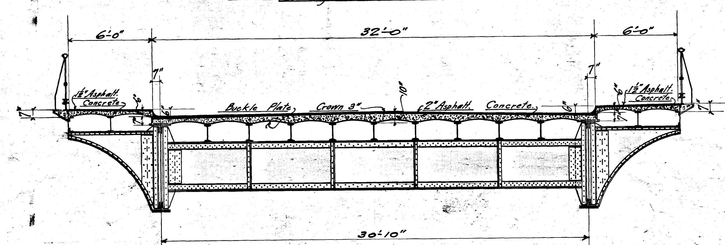
Cross Section with Buckle Plate Floor
