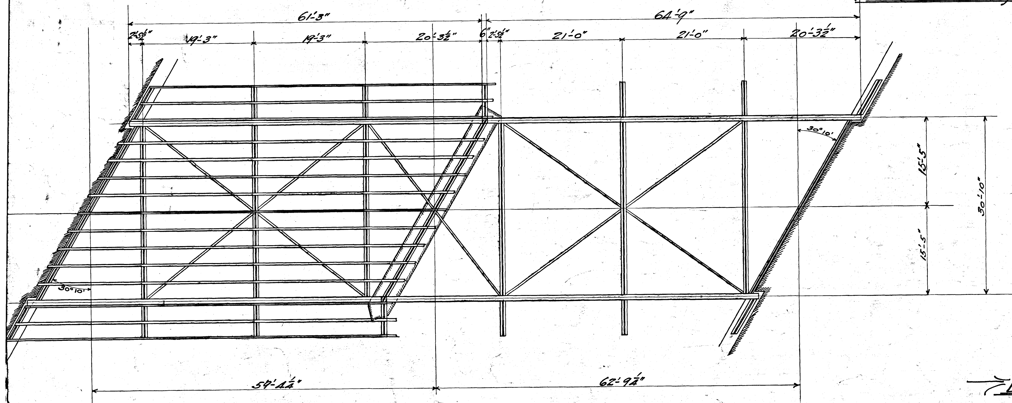
Plan of Bridge
