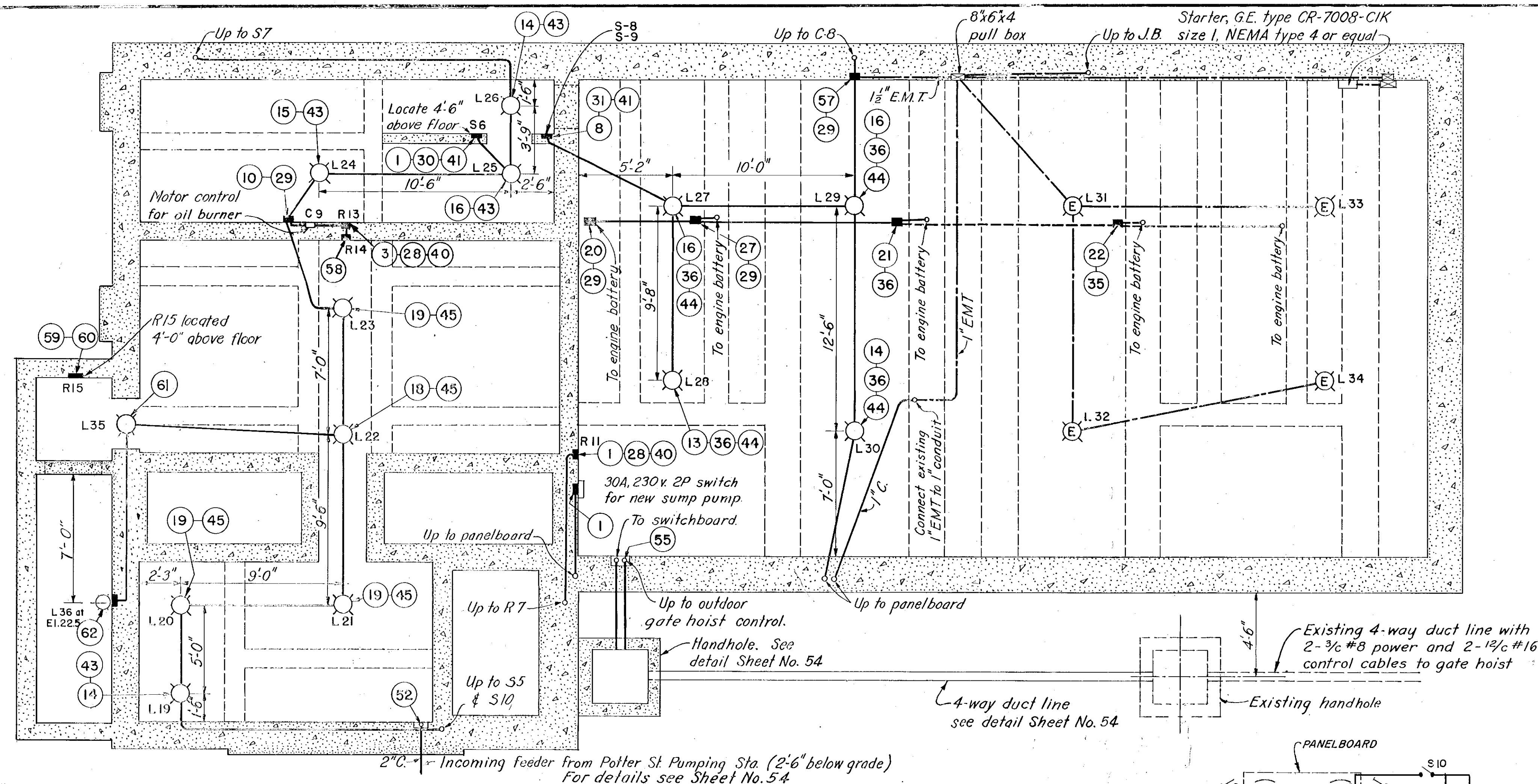
WIRING PLAN OF PUMP ROOM CEILING
