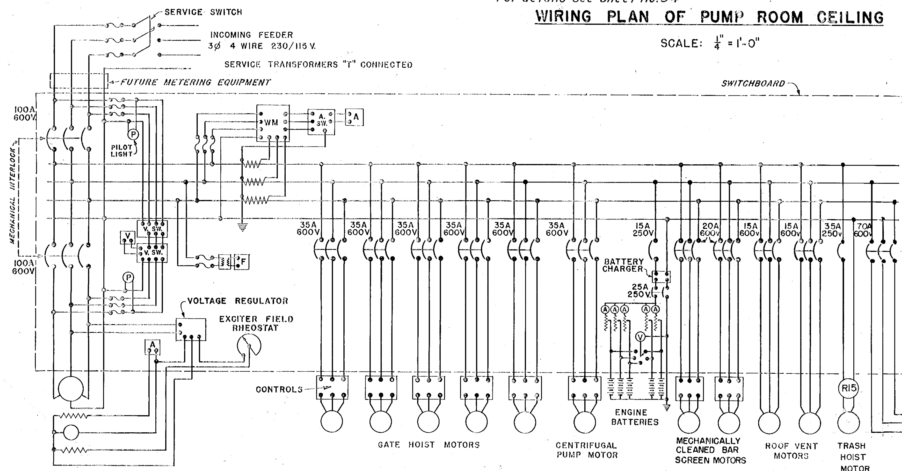
SCHEMATIC WIRING DIAGRAM
