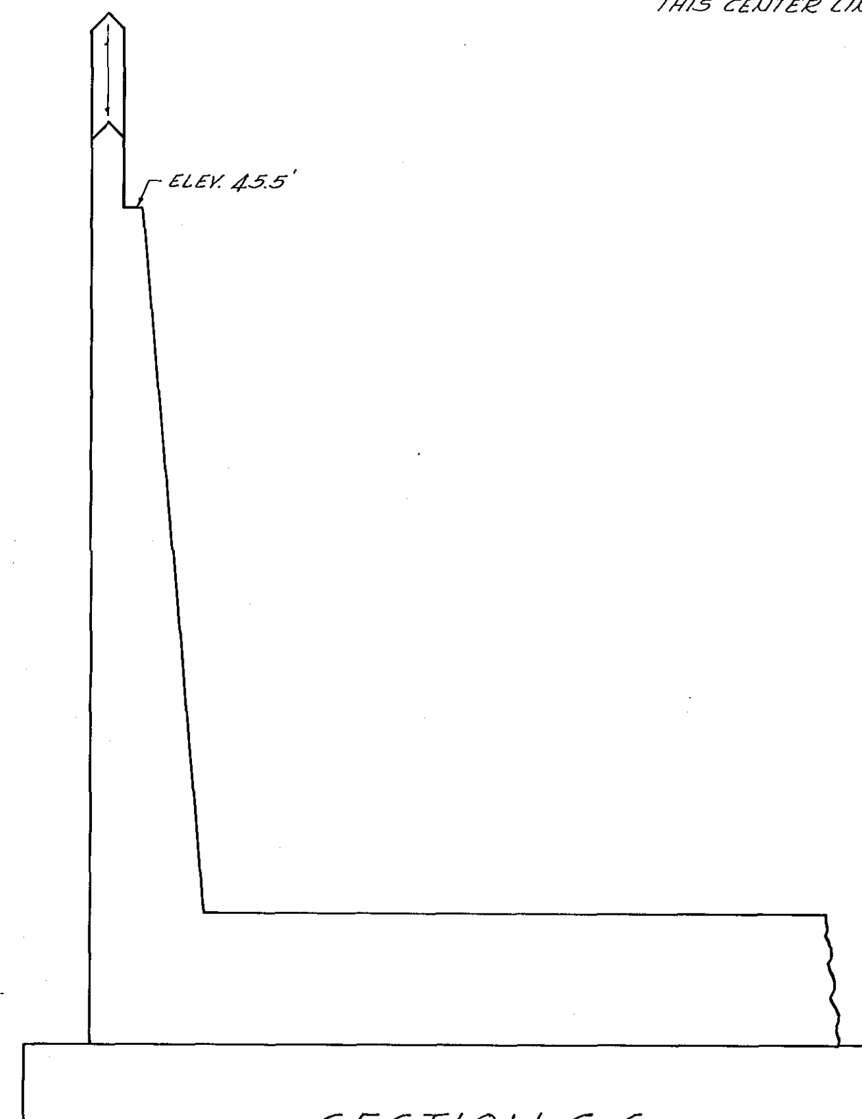
SECTION C-C
