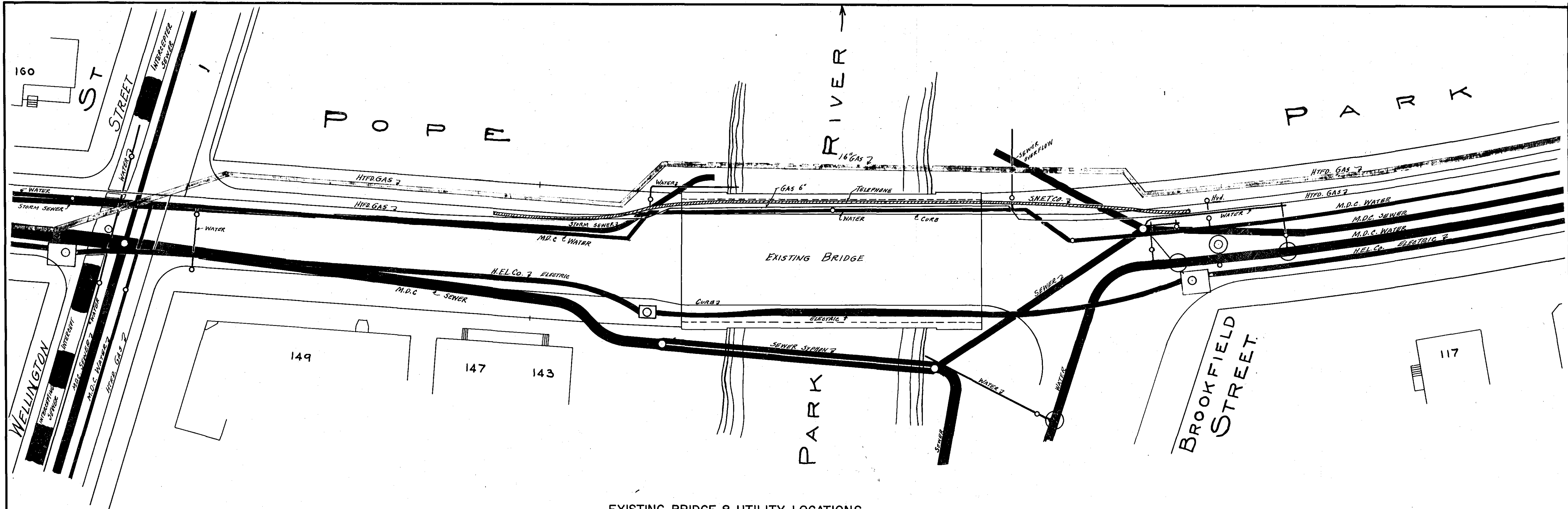
EXISTING BRIDGE & UTILITY LOCATIONS
