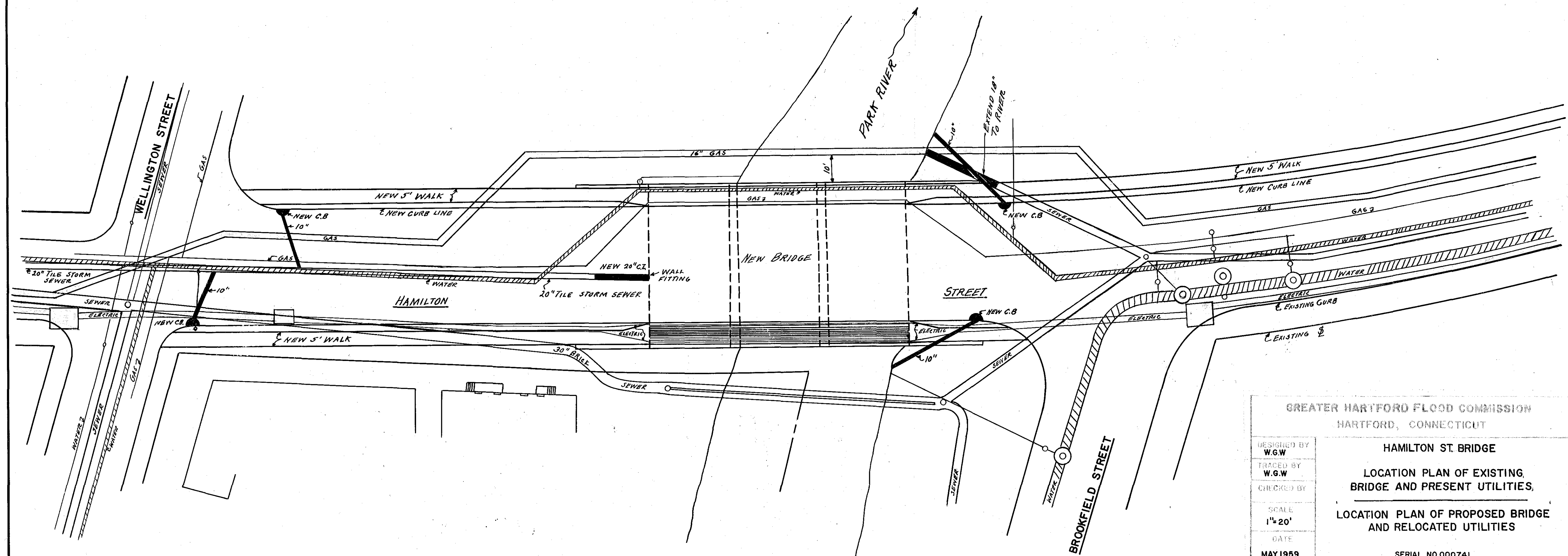
PROPOSED RELOCATION OF BRIDGE & UTILITIES
