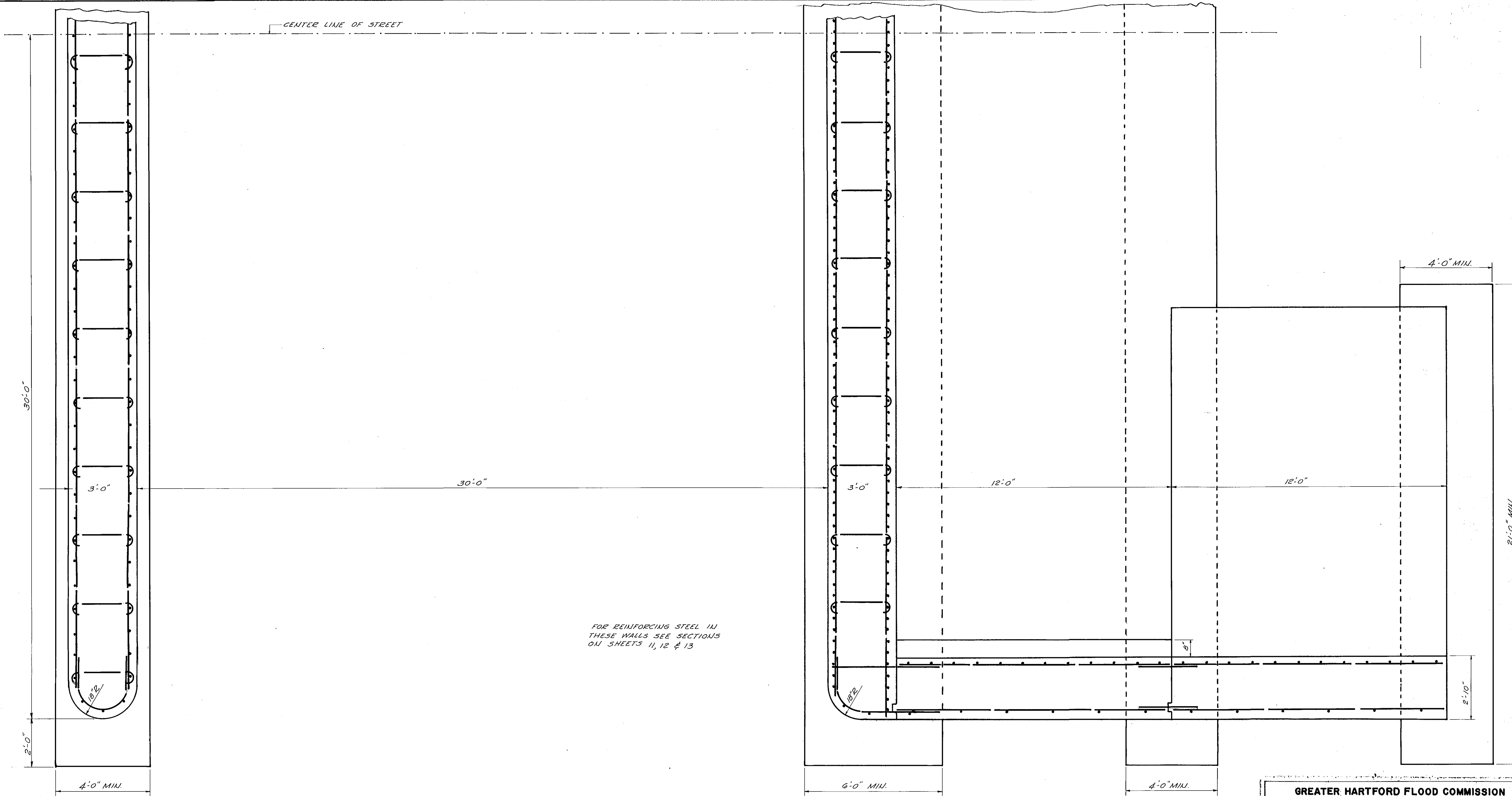
HORIZONTAL SECTION AT ELEVATION 31.0'
