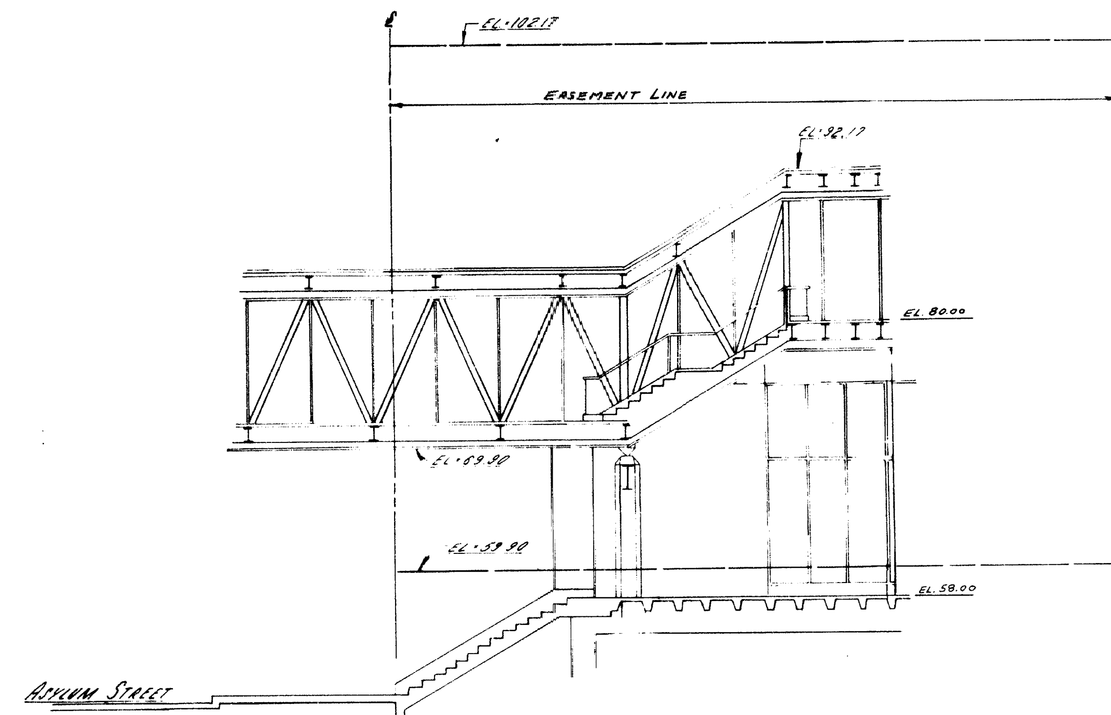
SECTION "B-B"
