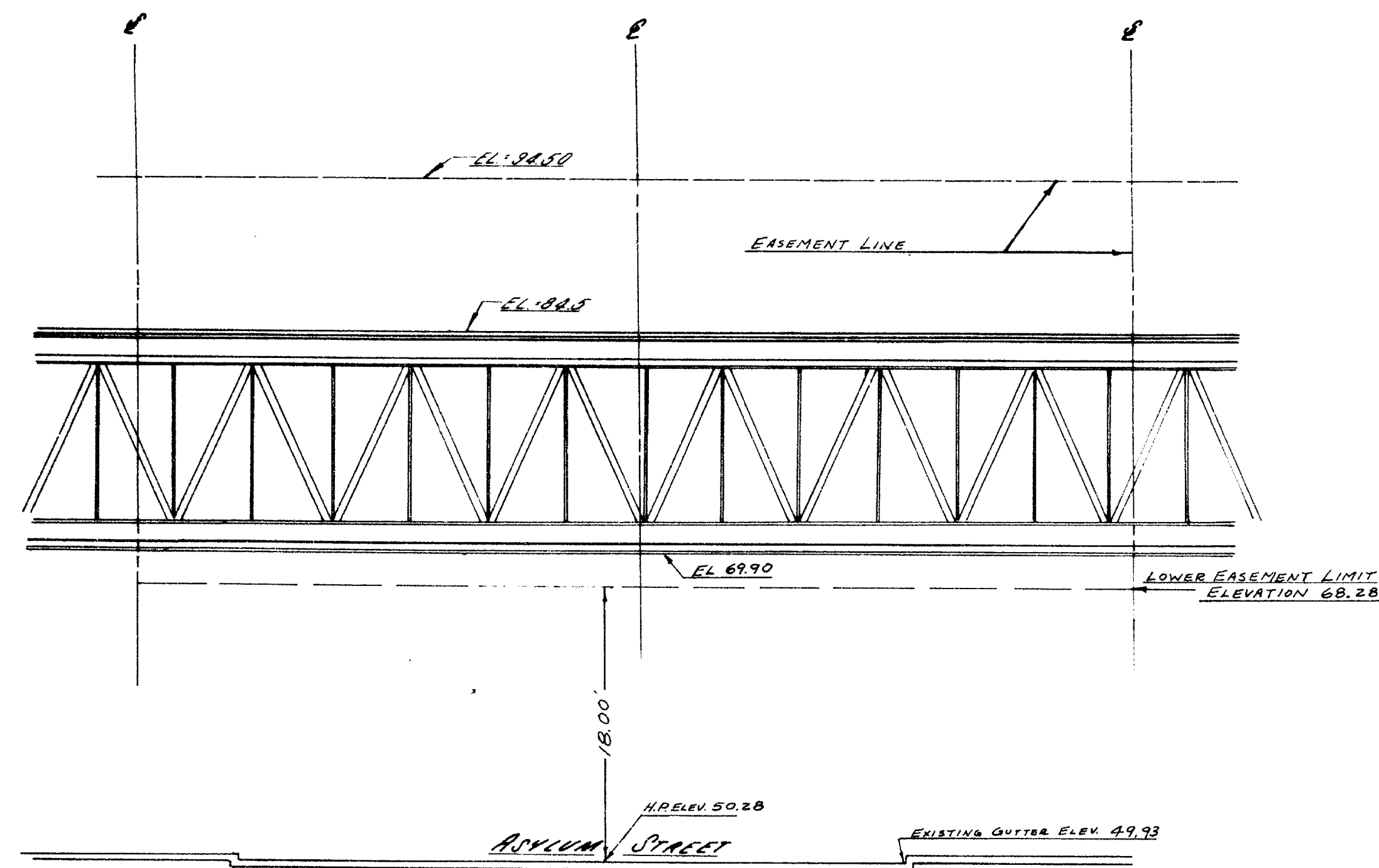
SECTION "A-A"
