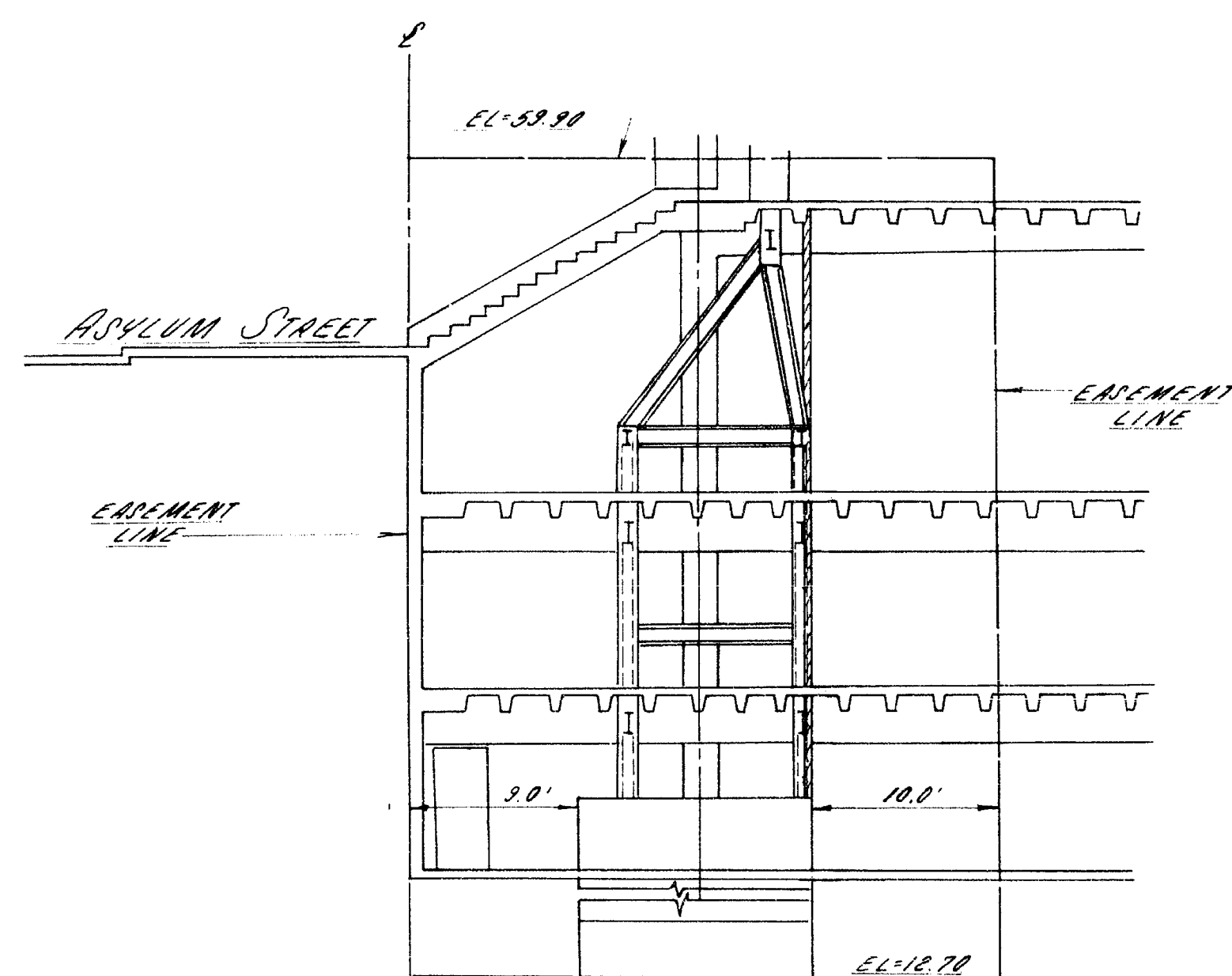
SECTION "B-B"
