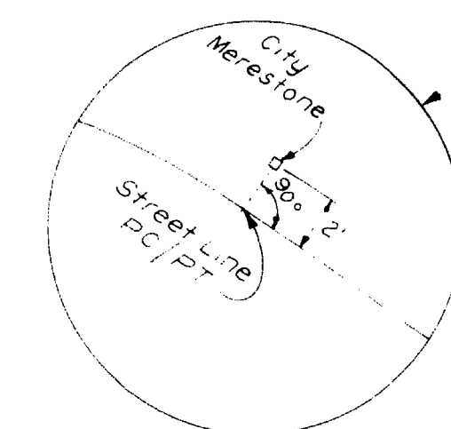
DETAIL City of Hartford standard method of monumentation
