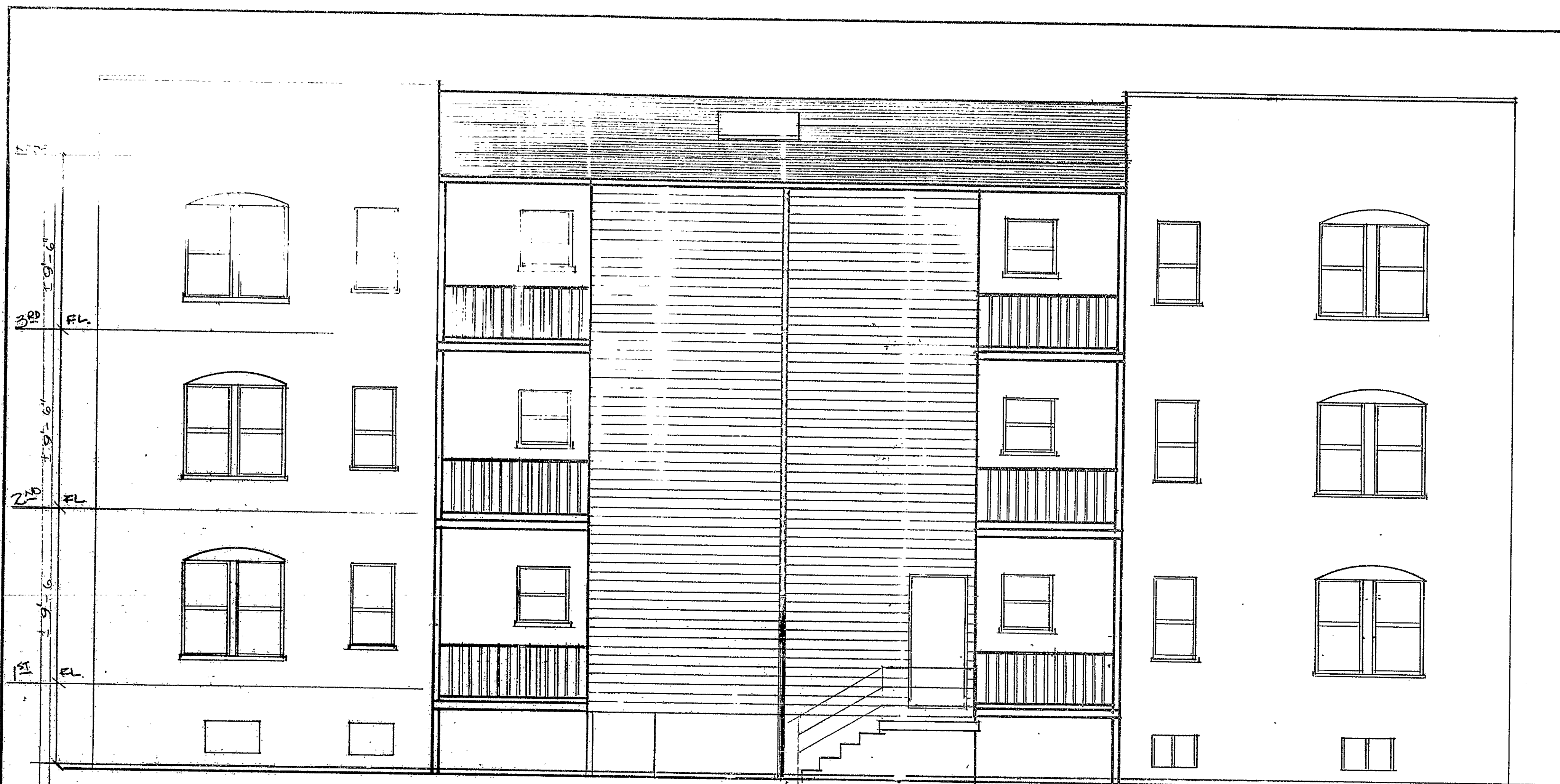
SOUTH ELEVATION
