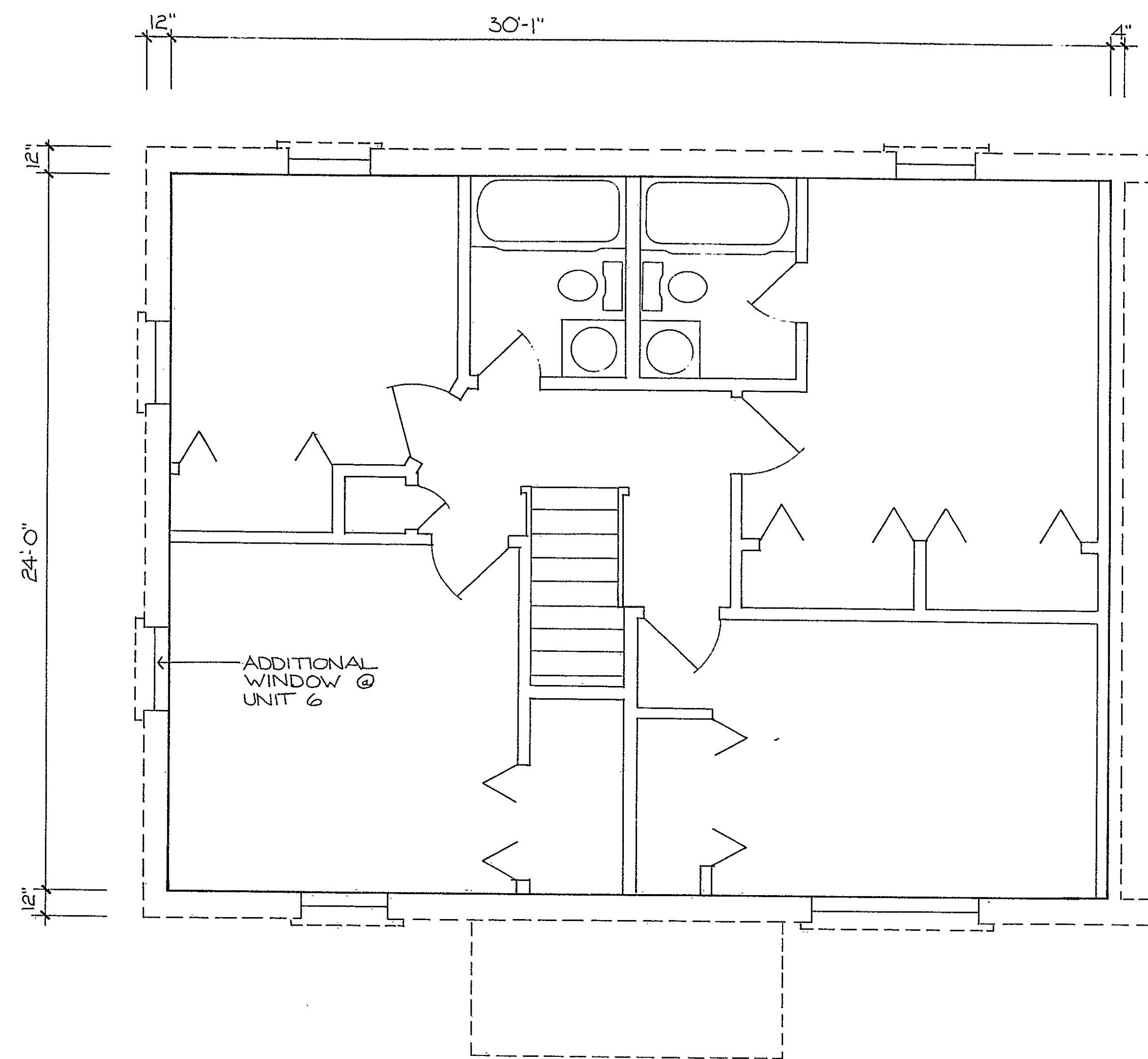
SECOND FLOOR
