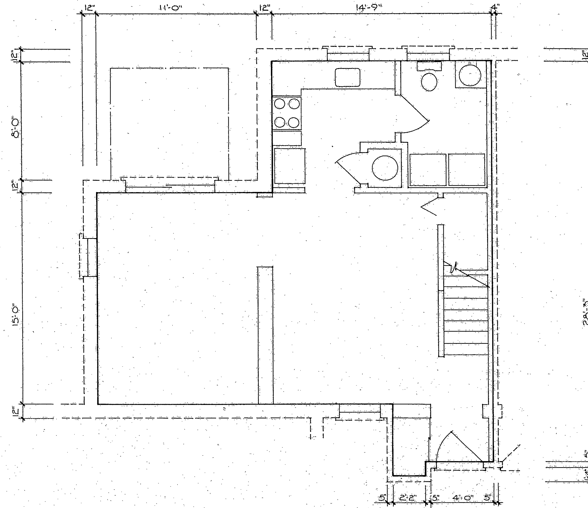
FIRST FLOOR
