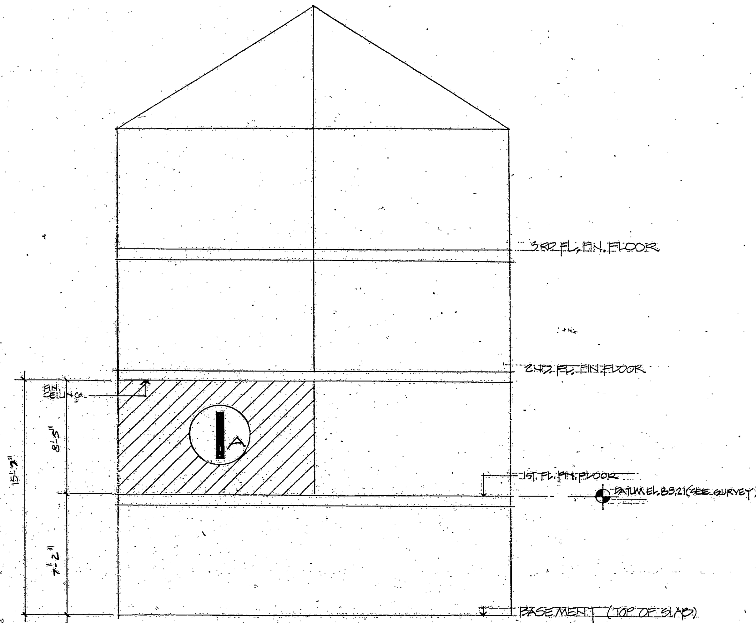
SCHEMATIC SECTION (N16)
