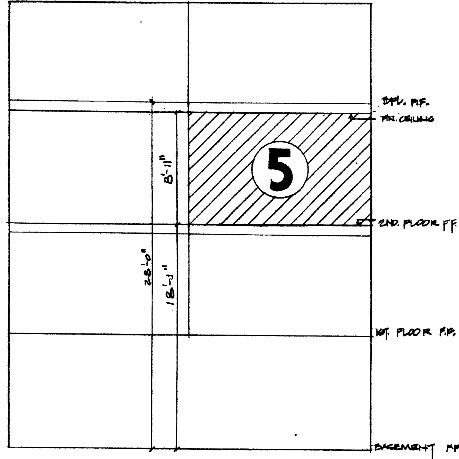
SCHEMATIC SECTION
