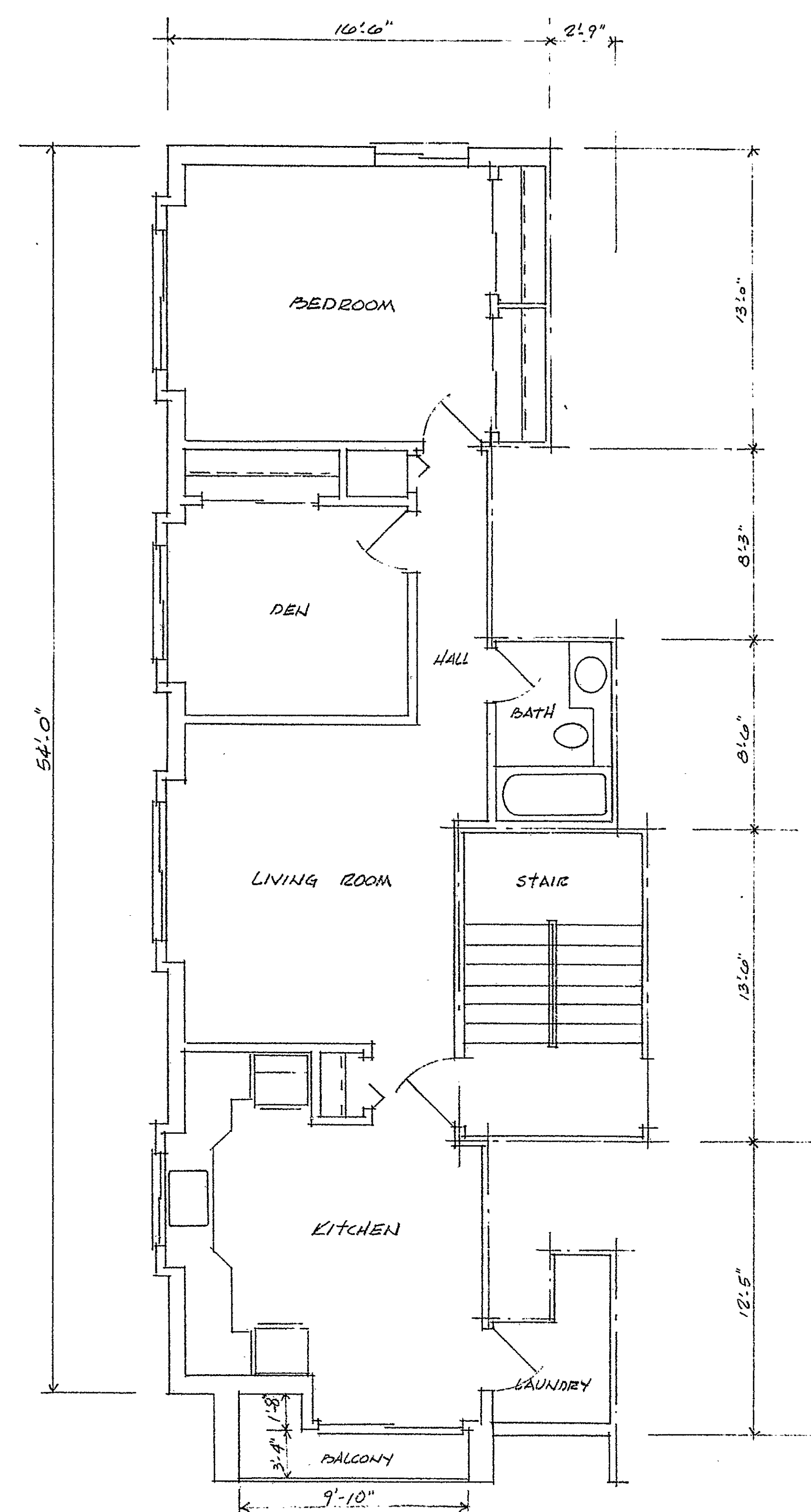
CARRIAGE HOUSE CONDOMINIUM TYPICAL DIAGRAMATIC FLOOR PLAN APPROXIMATE FLOOR AREA 864 SQ. FT. APPROXIMATE COMMON AREA 90 SQ. FT.
