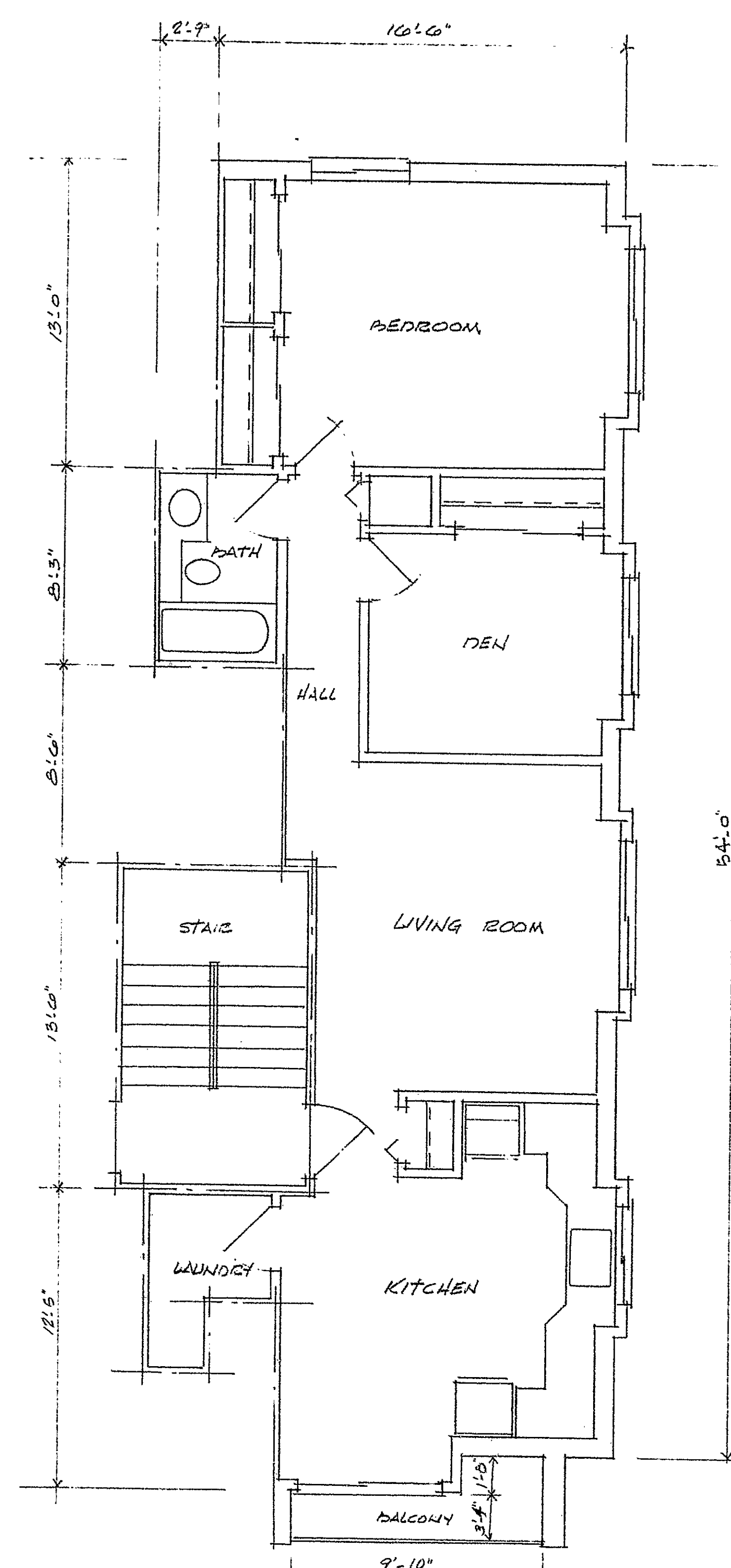
CARRIAGE HOUSE CONDOMINIUM TYPICAL DIAGRAMATIC FLOOR PLAN APPROXIMATE FLOOR AREA 864 SQ. FT. APPROXIMATE COMMON AREA 90 SQ. FT.
