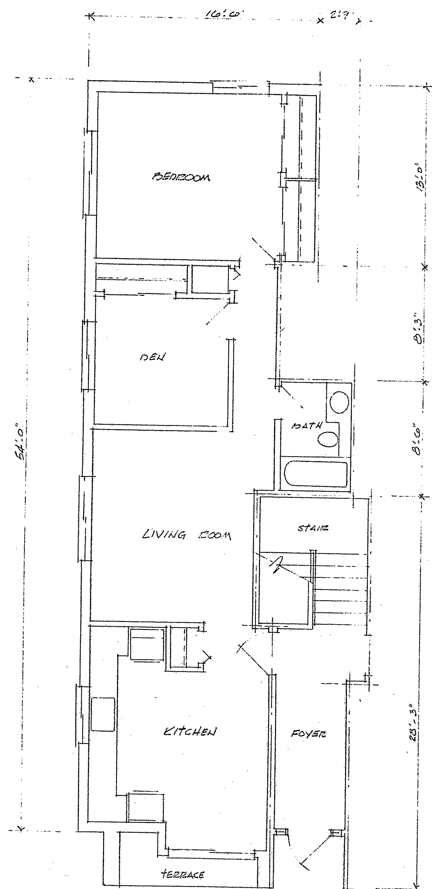
CARRIAGE HOUSE CONDOMINIUM HARTFORD, CONN. TYPICAL DIAGRAMATIC FLOOR PLAN APPROXIMATE FLOOR AREA 820 SQ. FT. APPROXIMATE COMMON AREA 253 SQ. FT. UNIT TYPE 1
