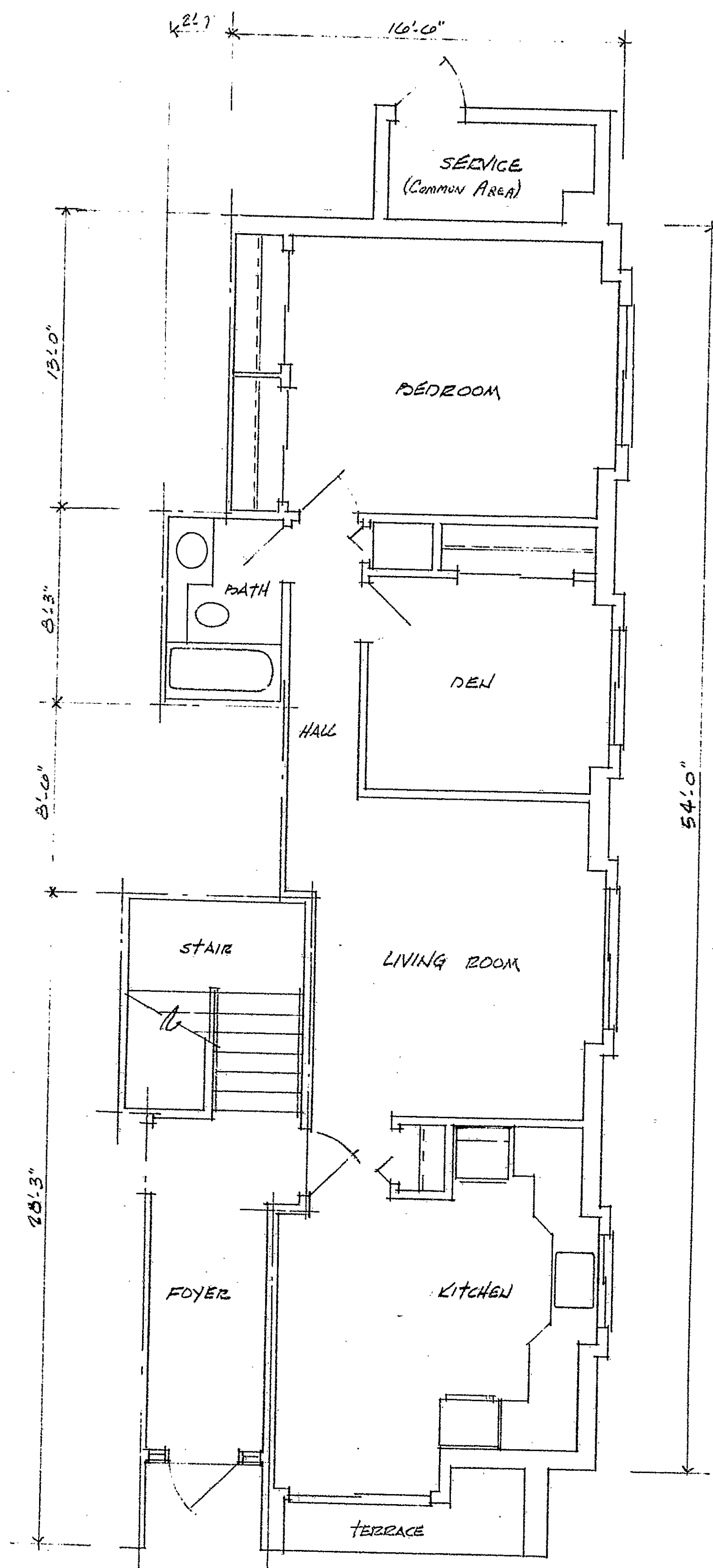
CARRIAGE HOUSE CONDOMINIUM HARTFORD, CONN. TYPICAL DIAGRAMATIC FLOOR PLAN APPROXIMATE FLOOR AREA 833 SQ. FT. APPROXIMATE COMMON AREA 253 SQ. FT. UNIT TYPE 2
