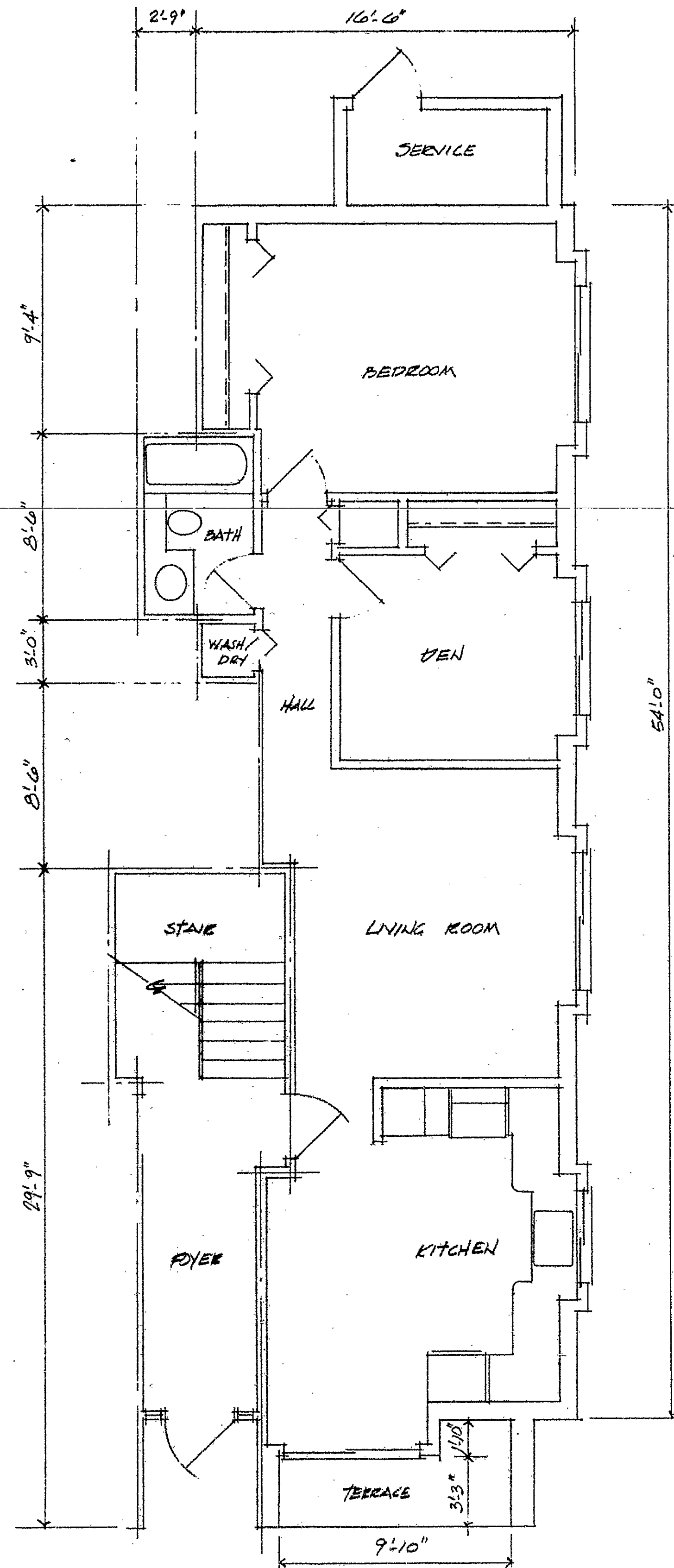
CARRIAGE HOUSE CONDOMINIUM HARTFORD, CONN. TYPICAL DIAGRAMATIC FLOOR PLAN - AMENDED APPROXIMATE FLOOR AREA - 833 S.F. APPROXIMATE COMMON AREA - 170 S.F. APPROXIMATE LIMITED COMMON AREA - 33 S.F. UNIT TYPE 2A
