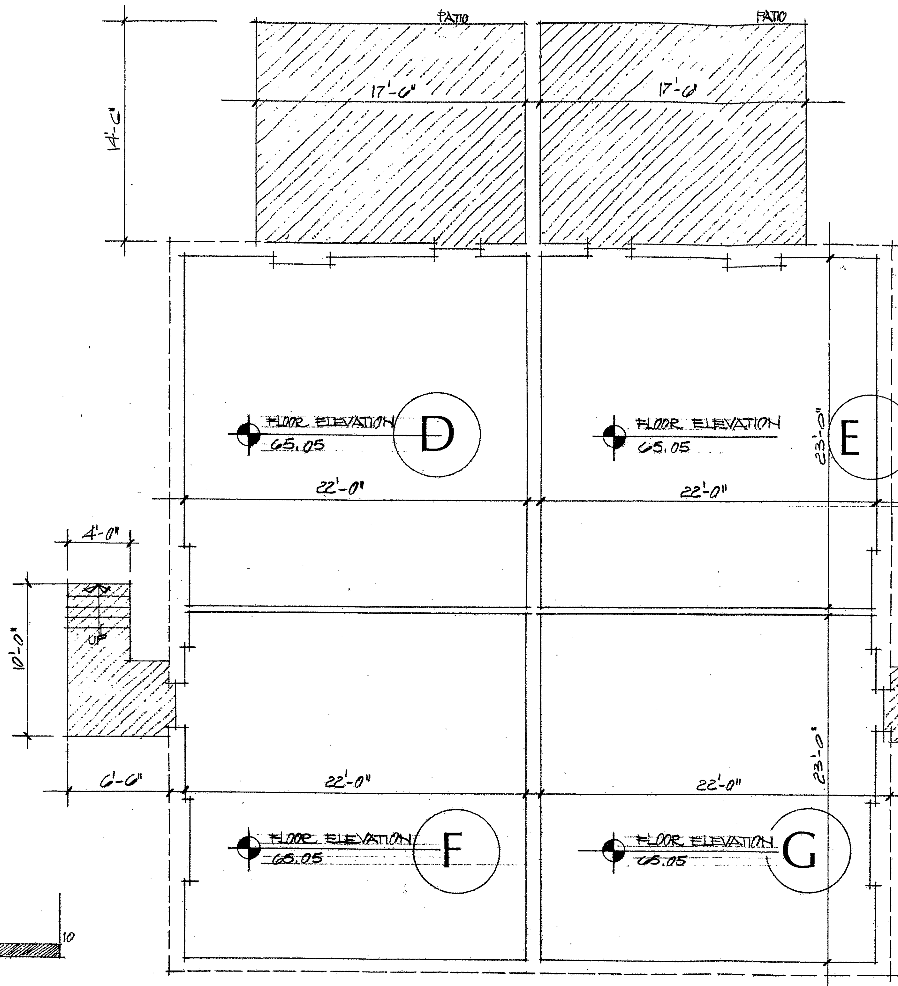
UNITS D, E, F, G LOWER FLOOR LEVEL
