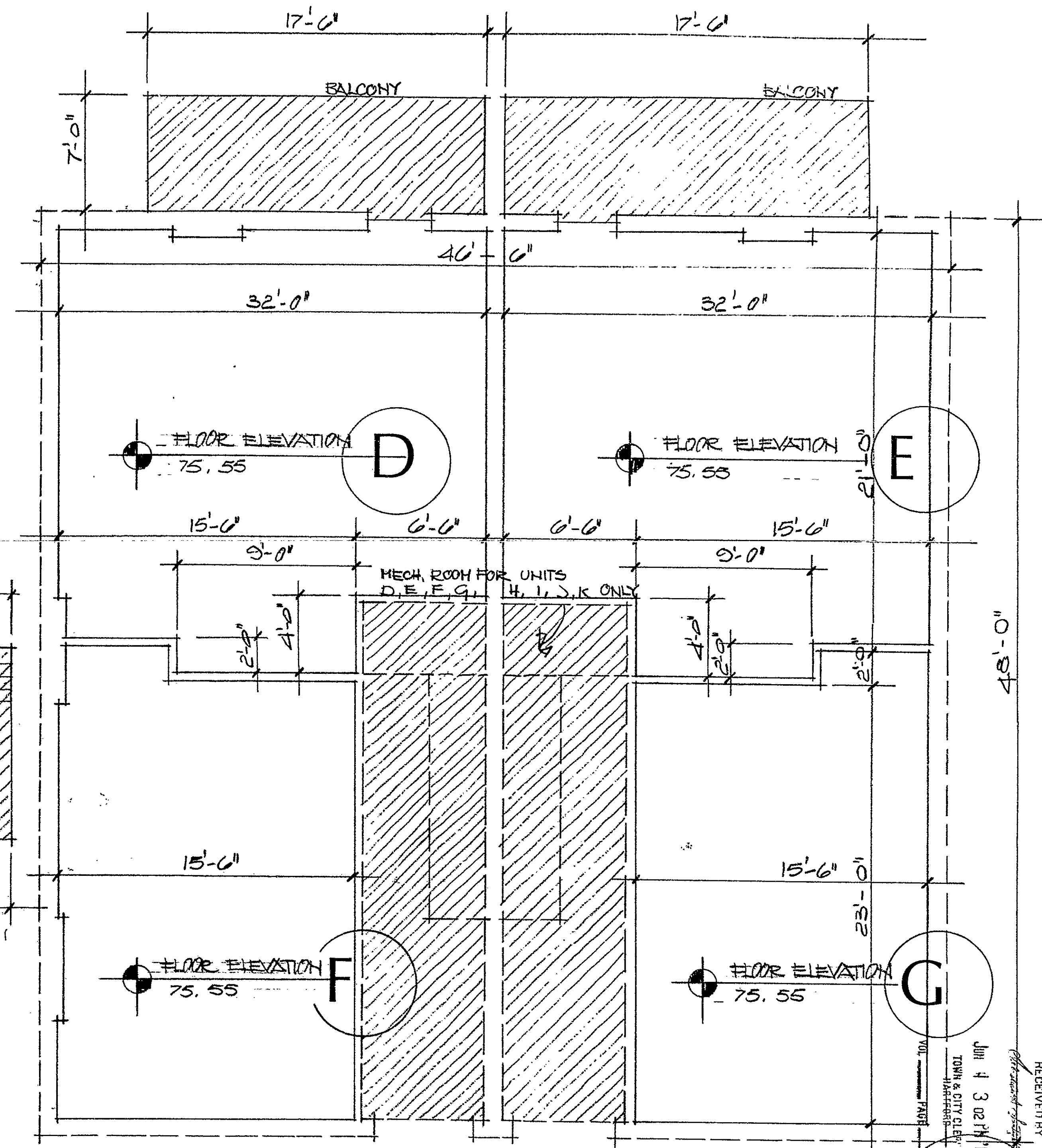
UNITS D, E, F, G MAIN FLOOR LEVEL
