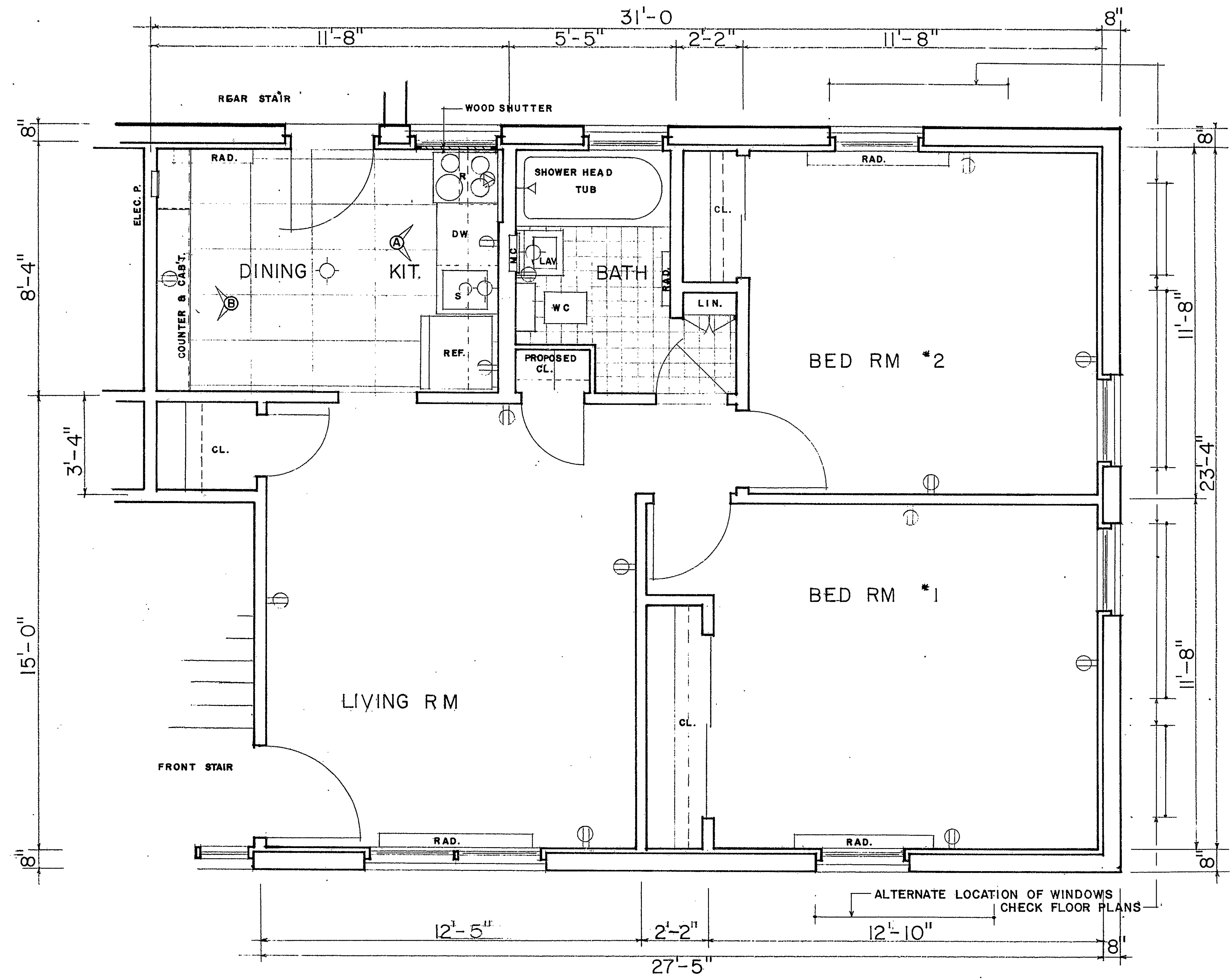
TYPICAL LAYOUT UNITS *2-*4-*6 SCALE 1/4" = 1'-0" ELEC. OUTLETS MAY VARY
