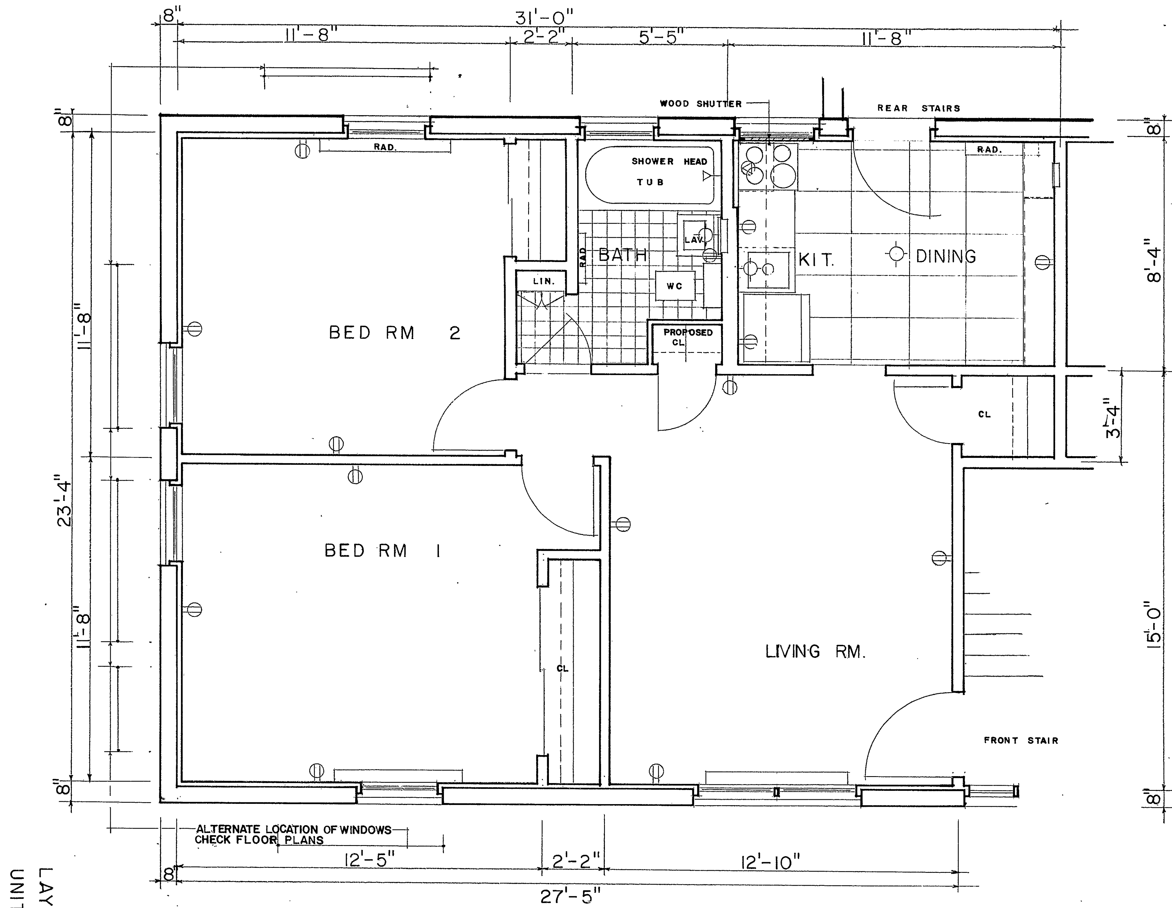
TYPICAL LAYOUT UNITS *1-3-5 SCALE 0 2 4 8ft ELEC. OUTLETS MAY VARY
