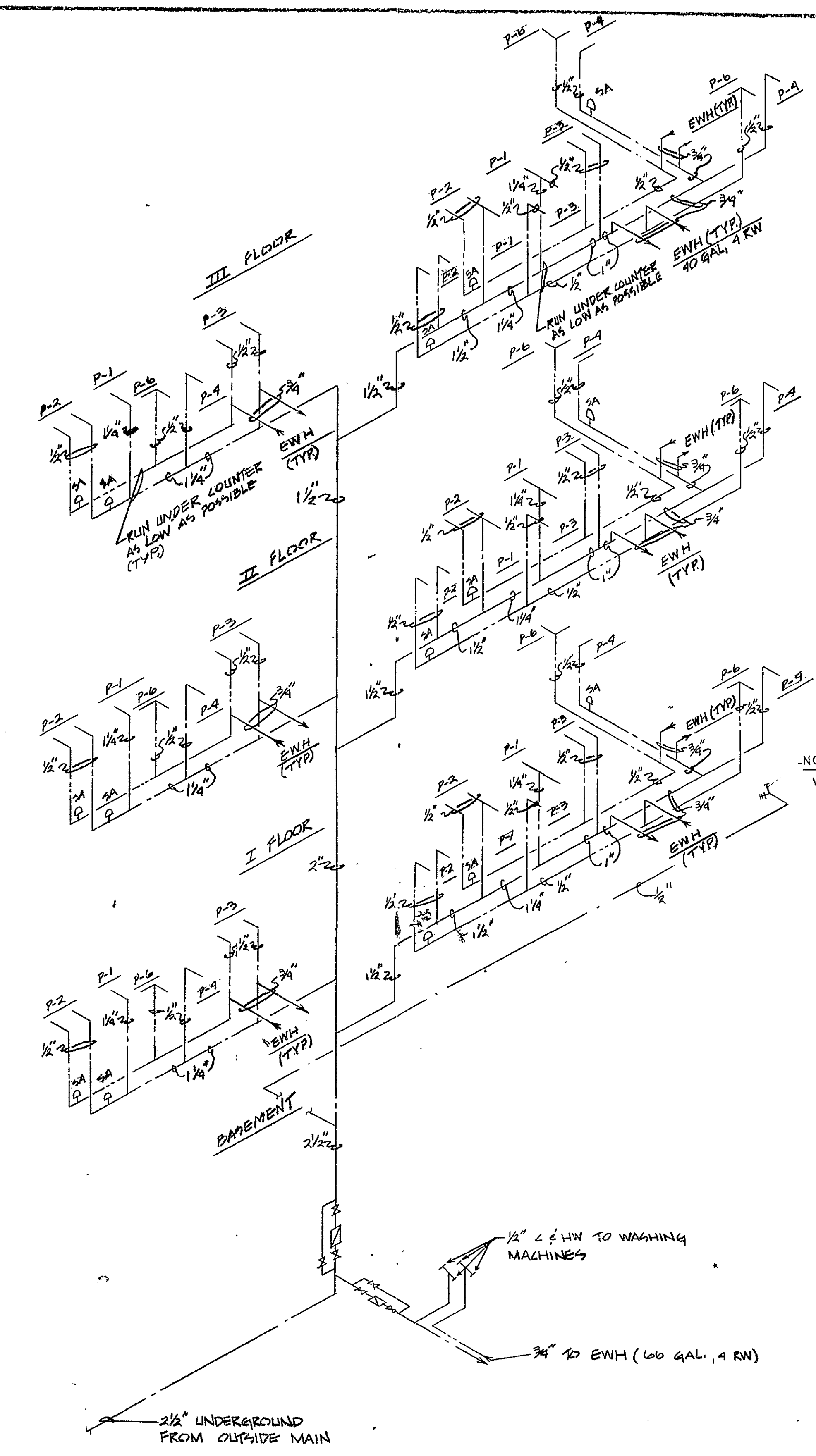
COLD & HOT WATER PIPING DIAGRAM NO SCALE
