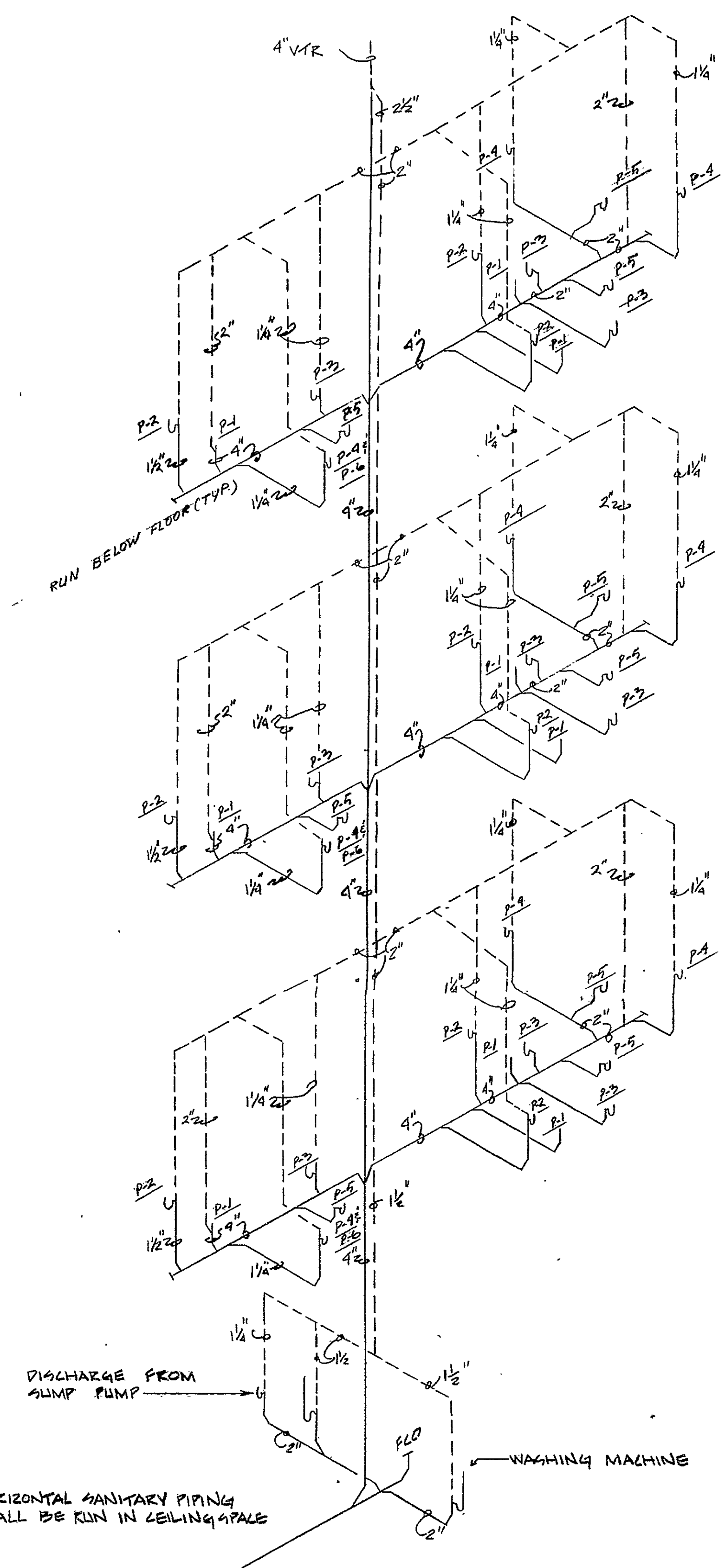
SANITARY & VENT PIPING DIAGRAM NO SCALE
