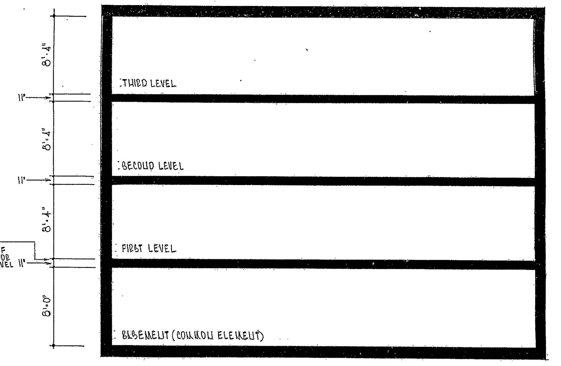
Schematic Section NOT TO SCALE
