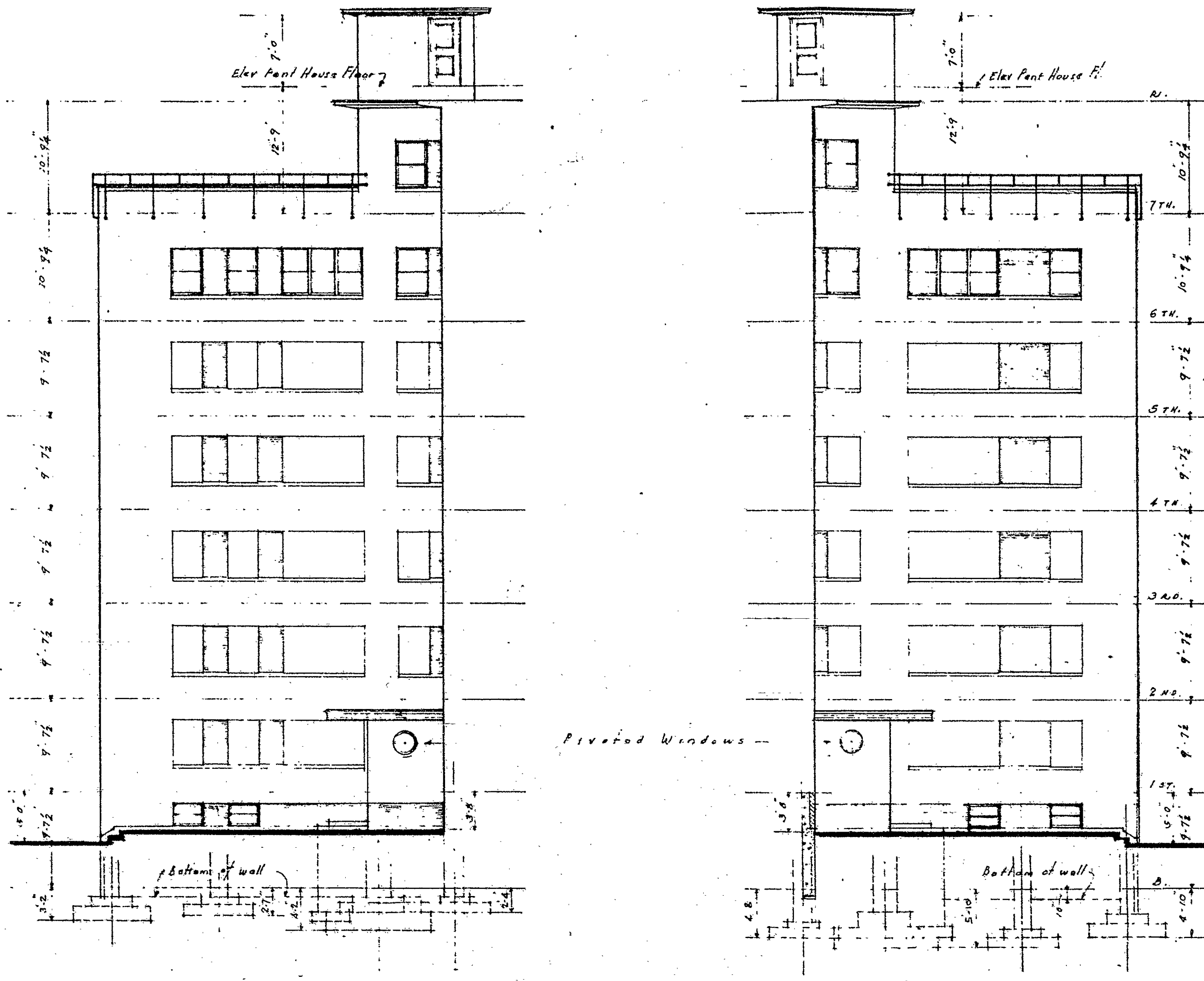
ELEVATIONS at EAST COURT south elev. north elev.
